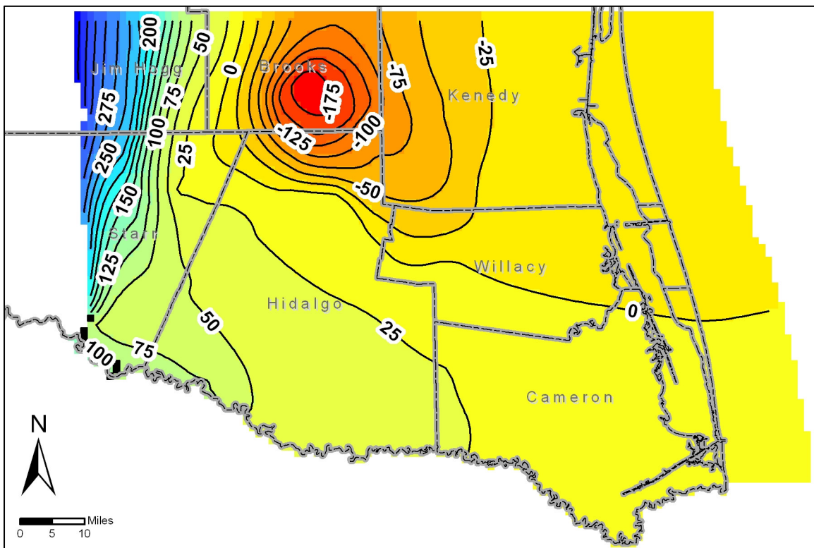
Figure 6. Water level elevations after 60 years using the specified pumpage in the Evangeline Aquifer. Water level elevations are in feet above mean sea level. Contour interval is 25 feet. Dry cells are shown in black.
