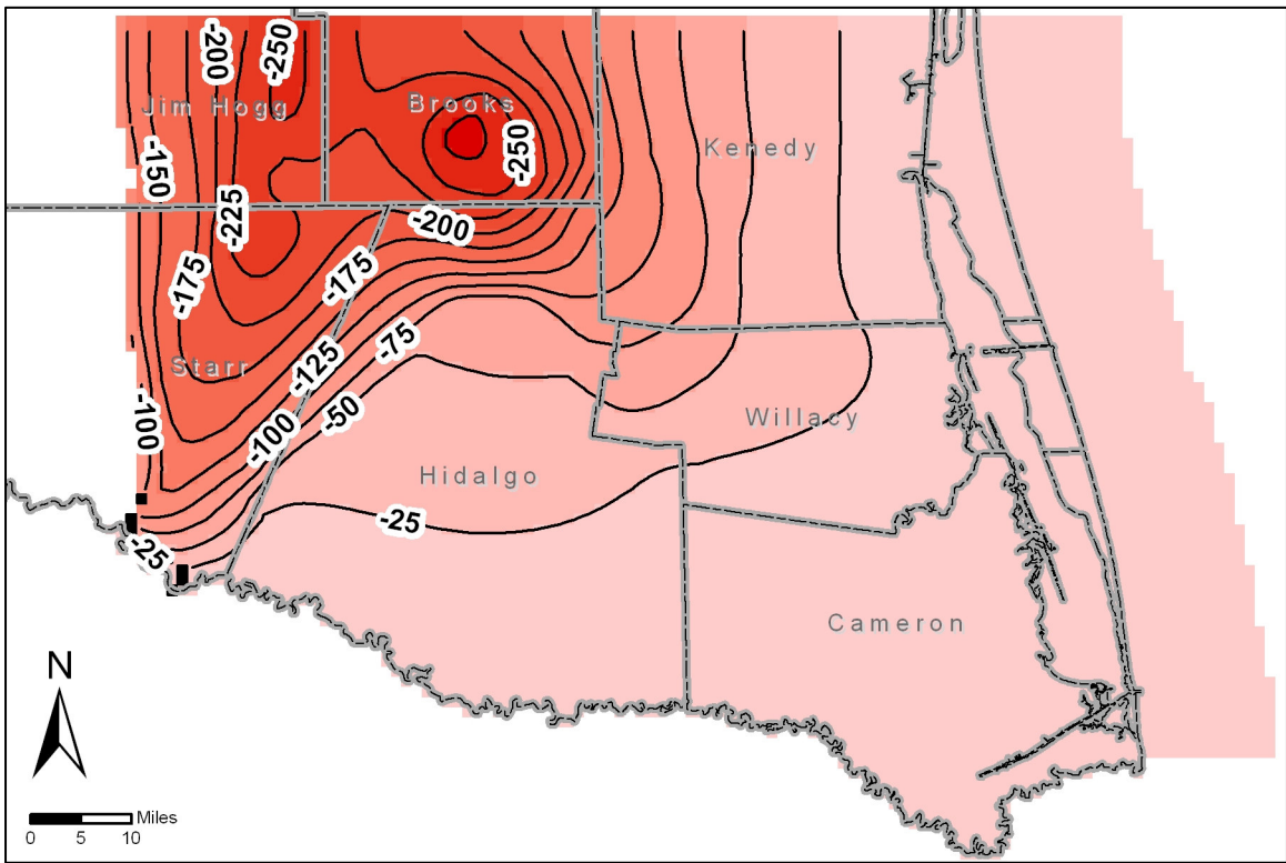
Figure 8. Water level changes (in feet) after 60 years using the specified pumpage in the Evangeline Aquifer. Contour interval is 25 feet. Areas of decreasing water levels (drawdown) are shown in red. Dry cells are shown in black.
