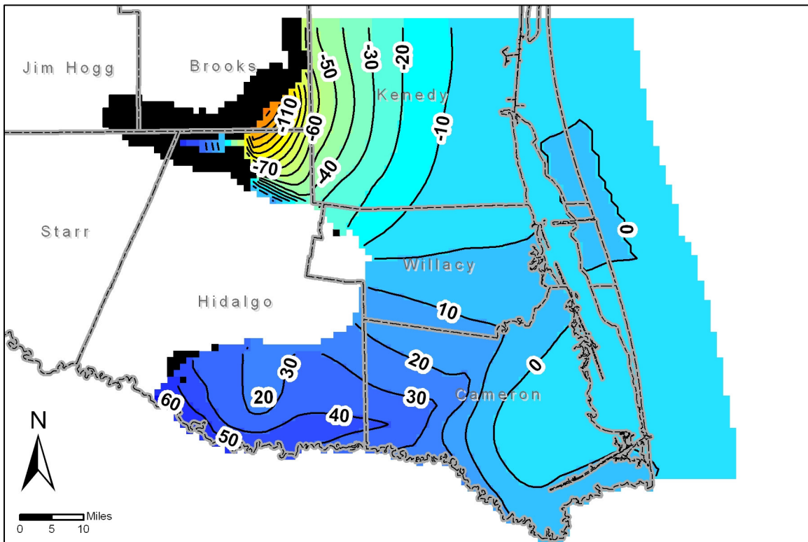
Figure 5. Water level elevations after 60 years using the specified pumpage in the Chicot Aquifer. Water level elevations are in feet above mean sea level. Contour interval is 10 feet. Dry cells are shown in black.
