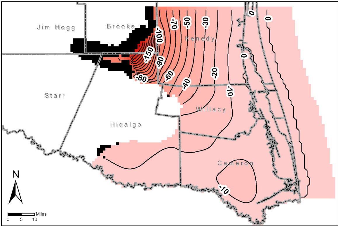
Figure 7. Water level changes (in feet) after 60 years using the specified pumpage in the Chicot Aquifer. Contour interval is 10 feet. Areas of decreasing water levels (drawdown) are shown in red. Dry cells are shown in black.
