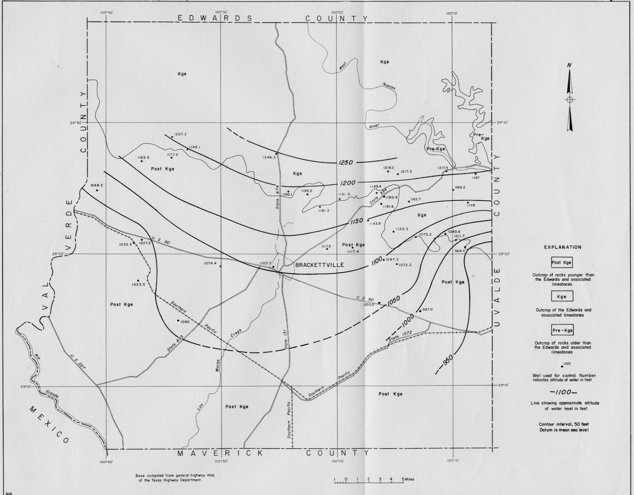
FIGURE 9.—Generalized geologic map of Kinney County, and configuration of the piezometric surface based on altitude of water levels in selected wells tapping the Edwards and associated limestones during the period 1937 - 40
