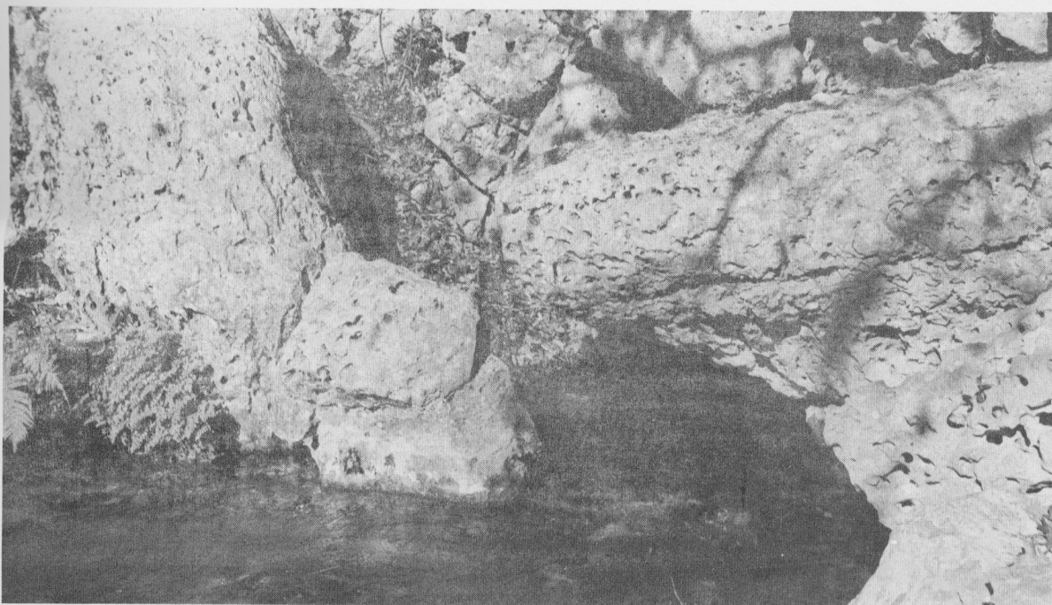
B. SCHWANDNER SPRING (F-1). WATER ISSUES FROM ONE LARGE OPENING IN THE EDWARDS LIMESTONE
