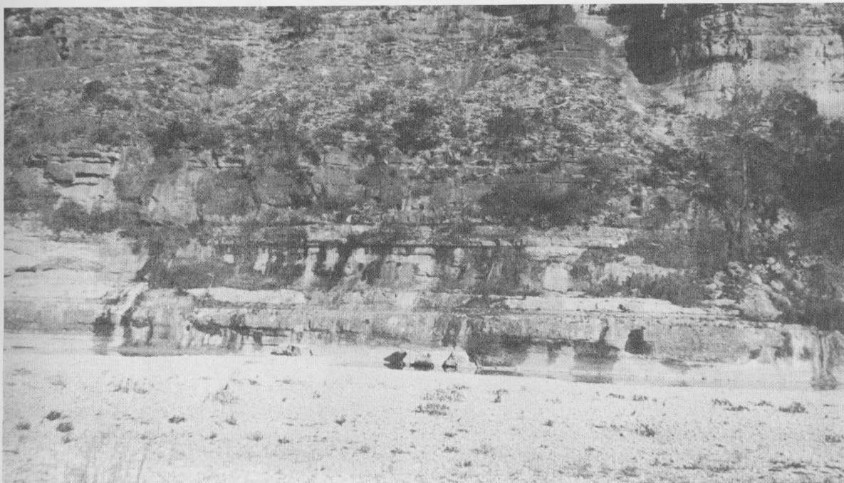
A. GRAVITY SPRINGS ISSUING FROM BASE OF EDWARDS LIMESTONE, EAST SIDE OF WEST NUECES RIVER, 5 MILES UPSTREAM FROM LAGUNA-BRACKETTVILLE ROAD
