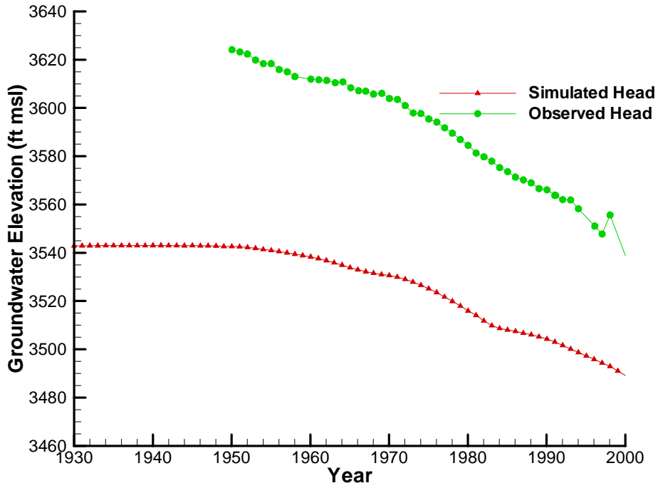
Simulated Head for GAINES1
