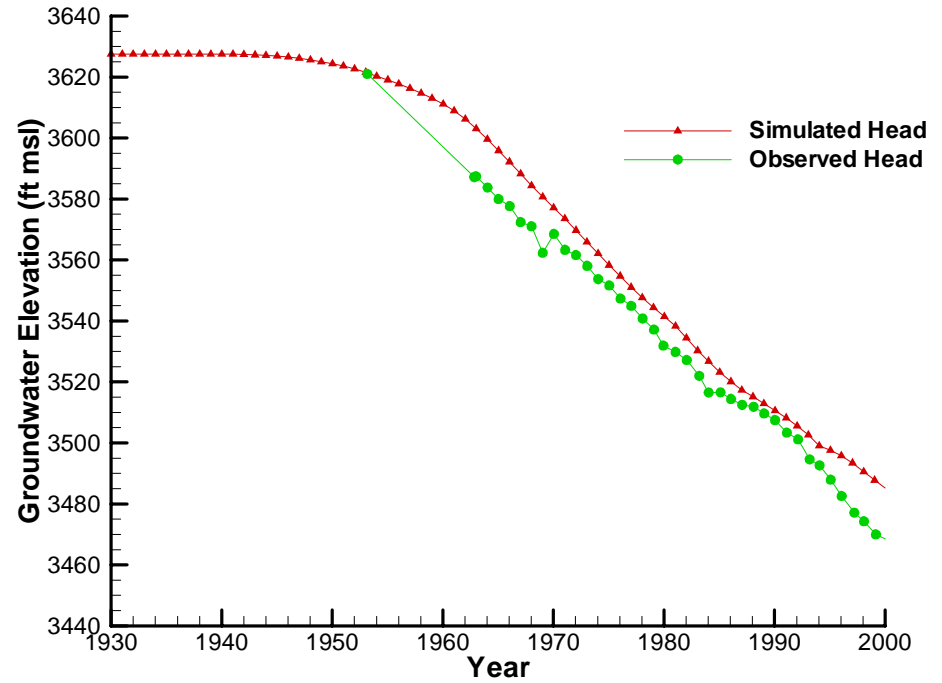
Simulated Head for CASTRO3
