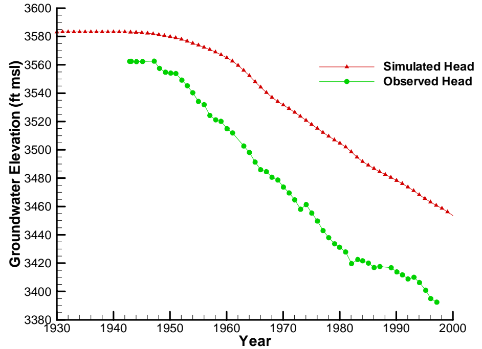
Simulated Head for LAMB2
