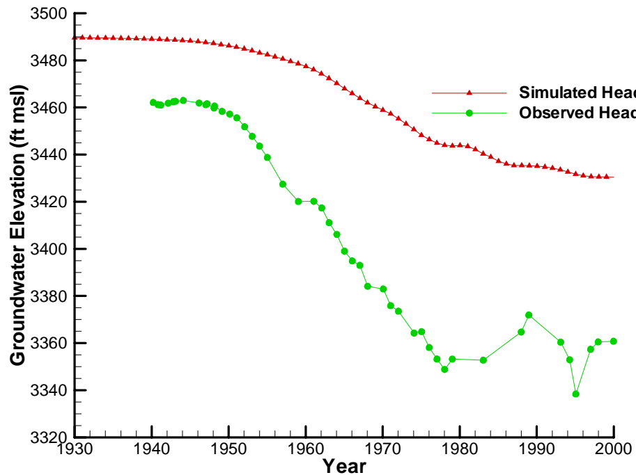
Simulated Head for SWISHER2
