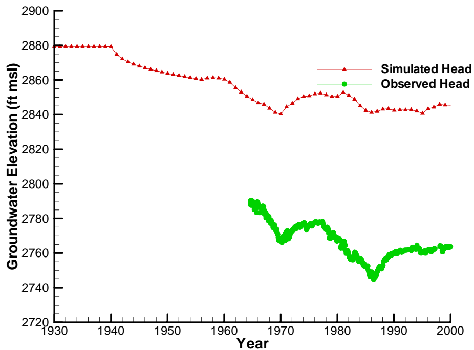
Simulated Head for MARTIN2
