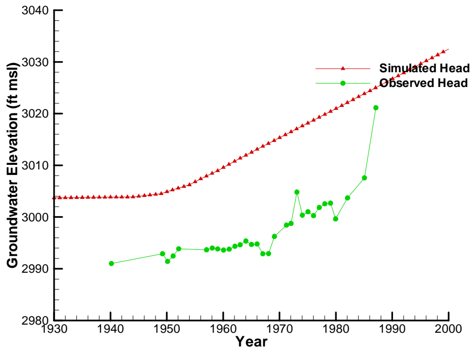
Simulated Head for LYNN1
