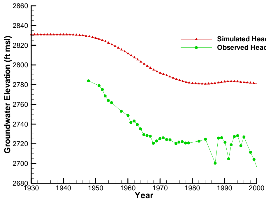
Simulated Head for MARTIN1
