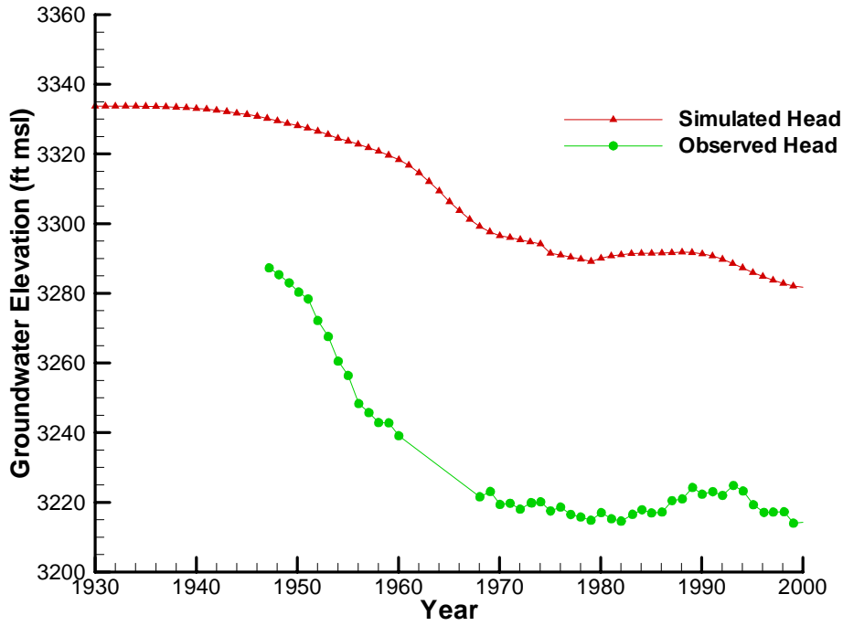
Simulated Head for HOCKLEY2
