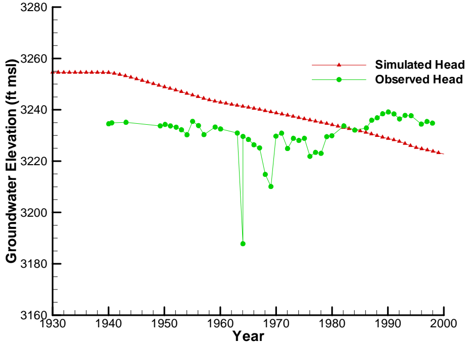
Simulated Head for GAINES3
