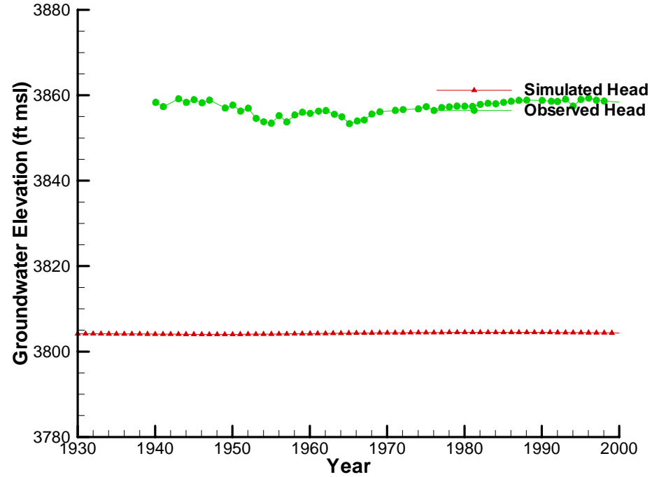
Simulated Head for LEA1
