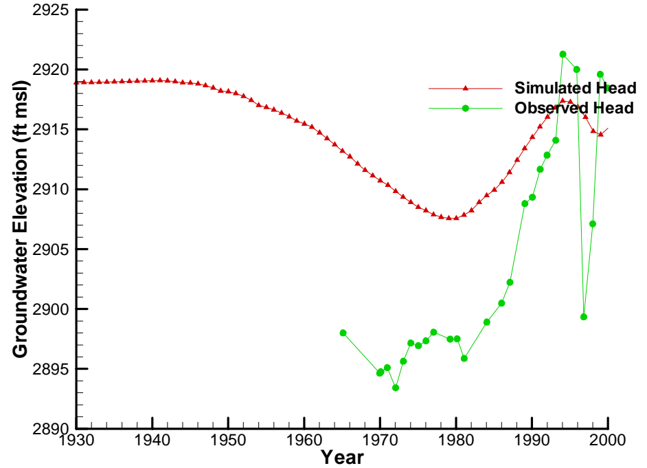
Simulated Head for GARZA1
