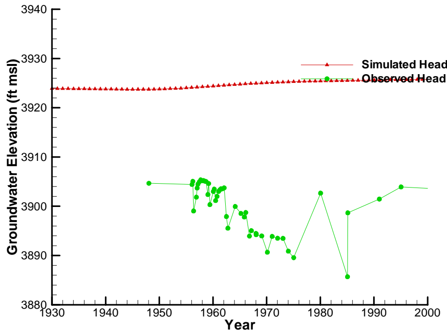
Simulated Head for ROOSEVELT3
