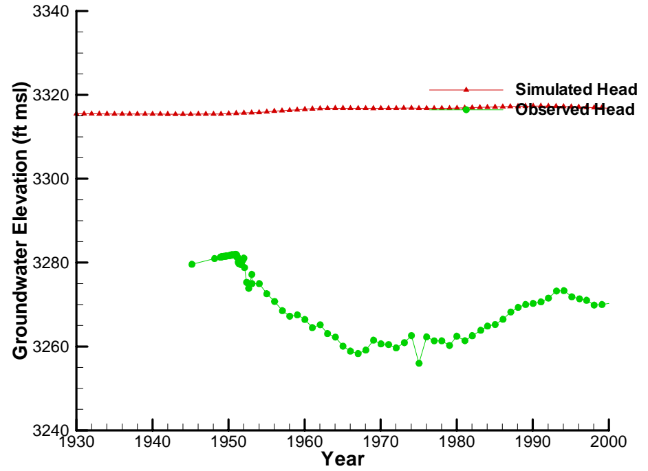
Simulated Head for HOCKLEY3
