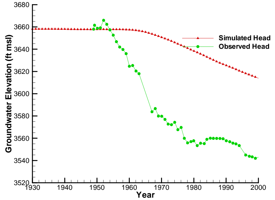
Simulated Head for CASTRO1
