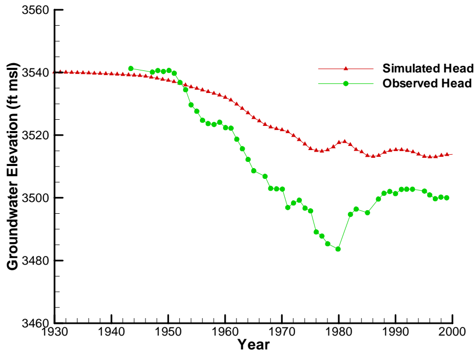
Simulated Head for SWISHER1
