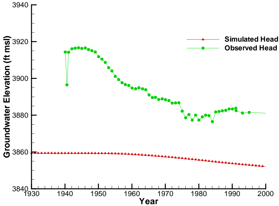
Simulated Head for LEA2
