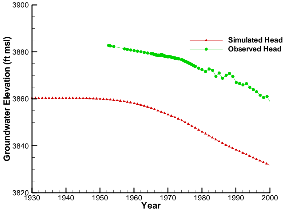
Simulated Head for BAILEY2
