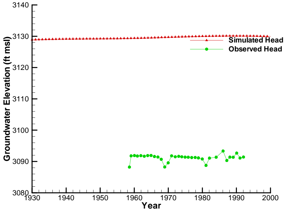
Simulated Head for ANDREWS1
