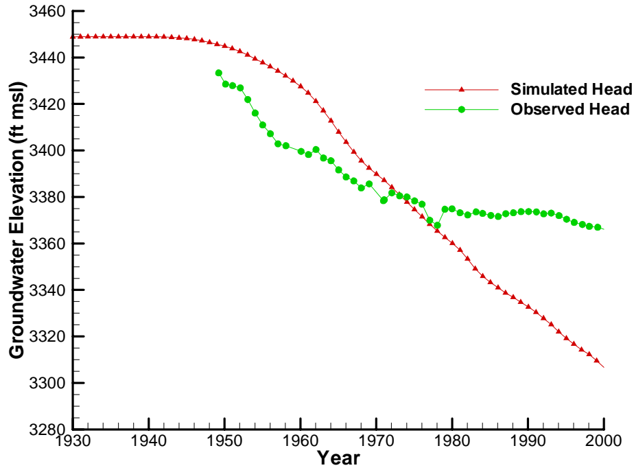
Simulated Head for LAMB3
