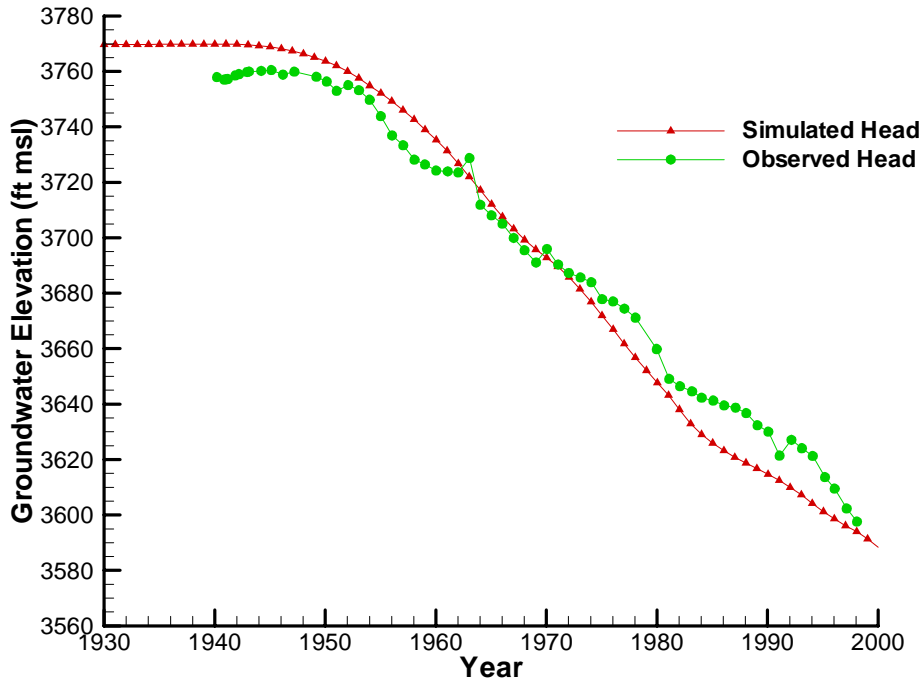
Simulated Head for LAMB1
