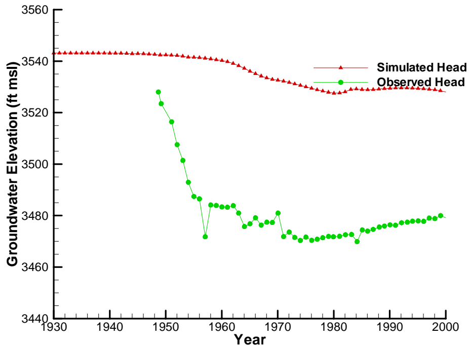
Simulated Head for RANDALL2
