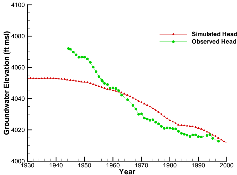
Simulated Head for ROOSEVELT1
