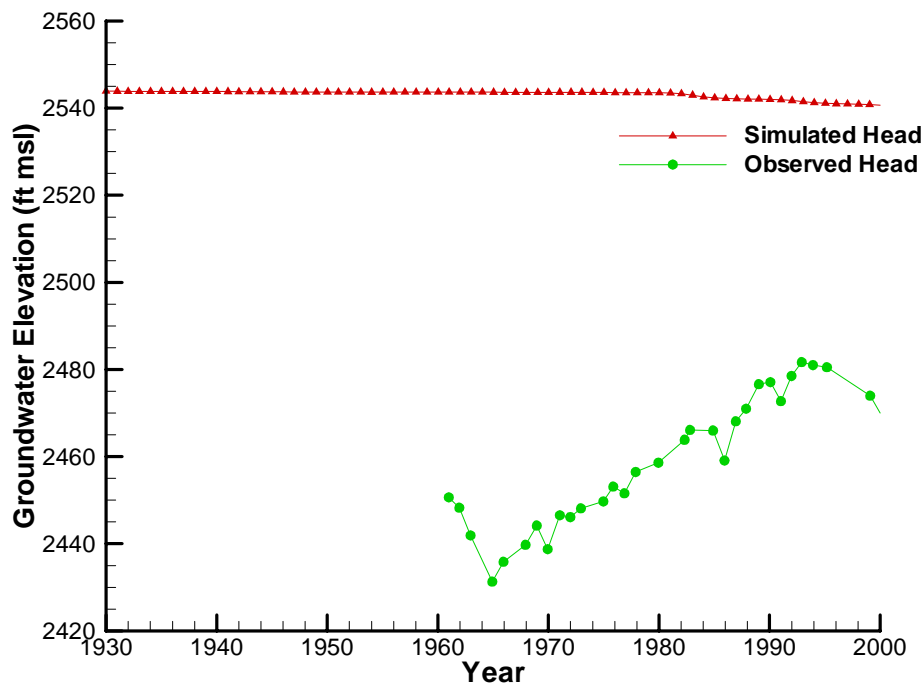
Simulated Head for GLASSCOCK2
