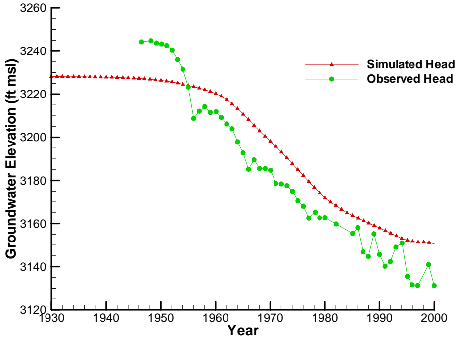
Simulated Head for BRISCOE3
