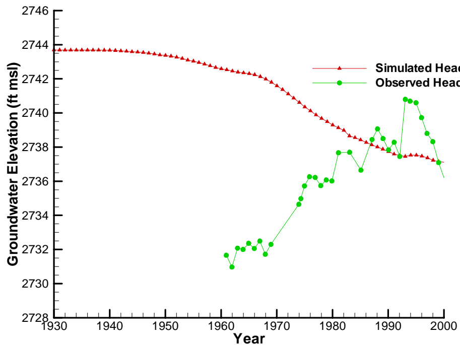
Simulated Head for MIDLAND1
