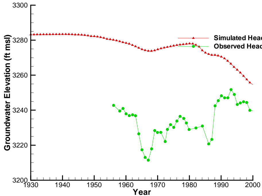
Simulated Head for TERRY1
