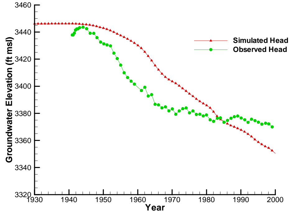
Simulated Head for LAMB4
