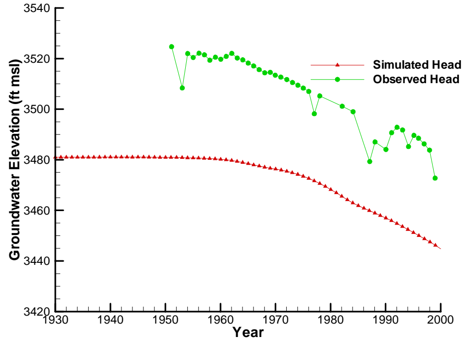
Simulated Head for GAINES2
