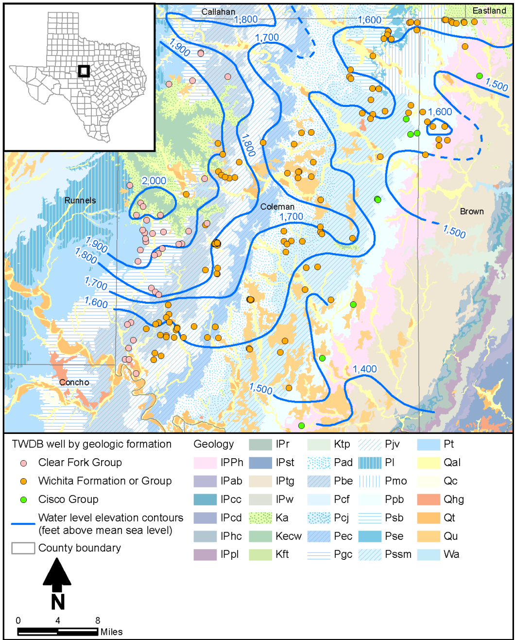
Figure 4-37. Cross Timbers Aquifer water level map for Coleman County based on 1960s water level data. See Appendix A, Figure A-1b for explanation of geologic symbols.
