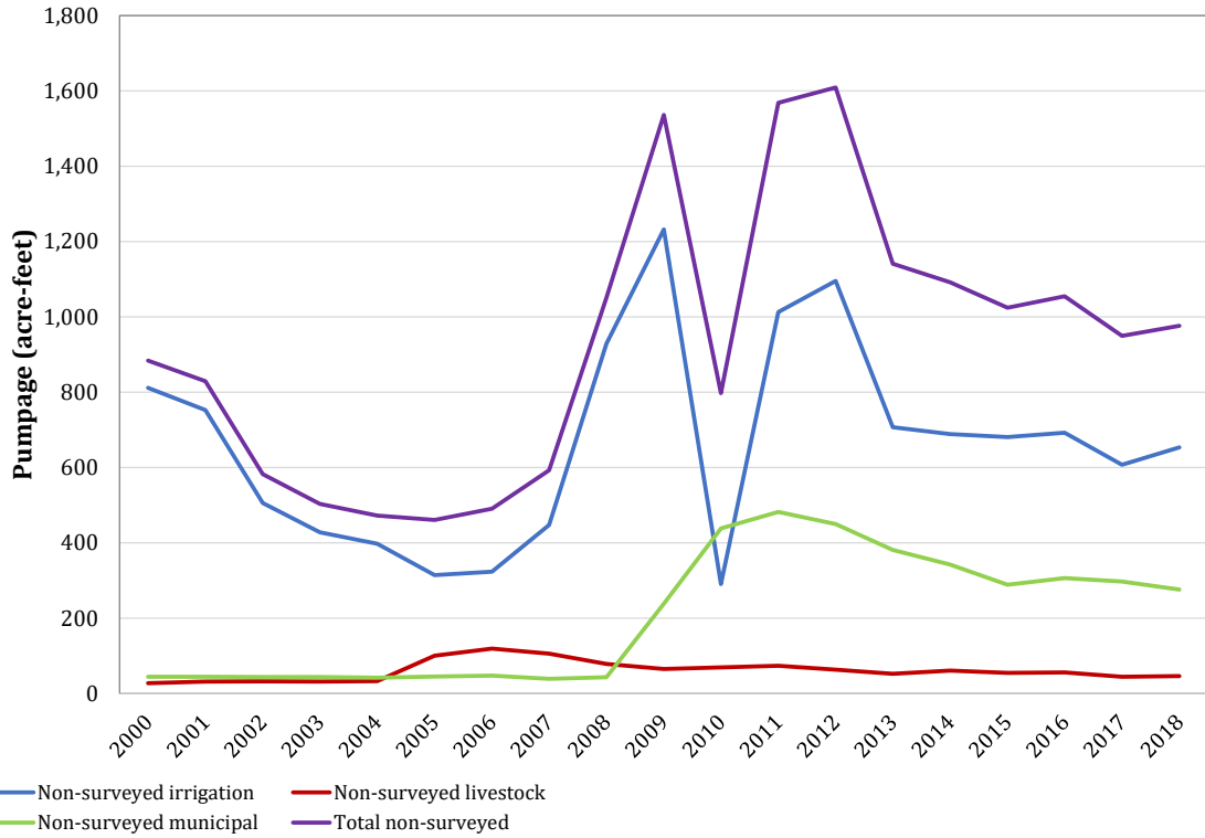
Figure 4-90. Estimated non-surveyed pumpage for the Cross Timbers Aquifer from 2000 to 2018 in Jones County.
