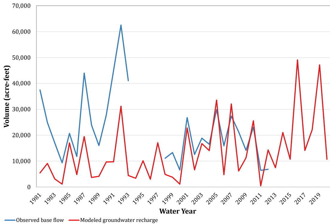
Figure C-20. Comparison of recharge simulation results to observed base flow for gauge 08144600 (San Saba).
