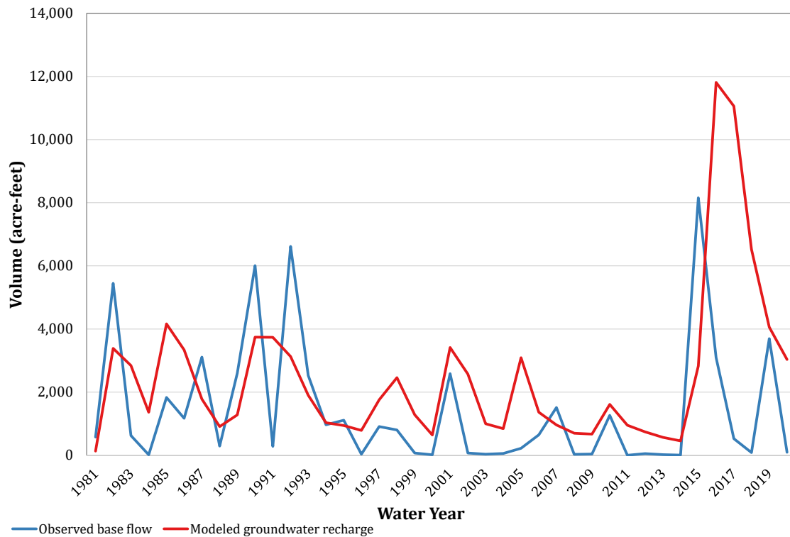
Figure C-4. Comparison of recharge simulation results to observed base flow for gauge 07315200 (Little Wichita).
