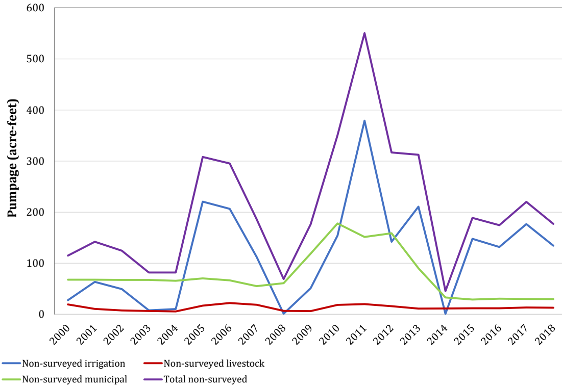
Figure 4-104. Estimated non-surveyed pumpage for the Cross Timbers Aquifer from 2000 to 2018 in Taylor County.
