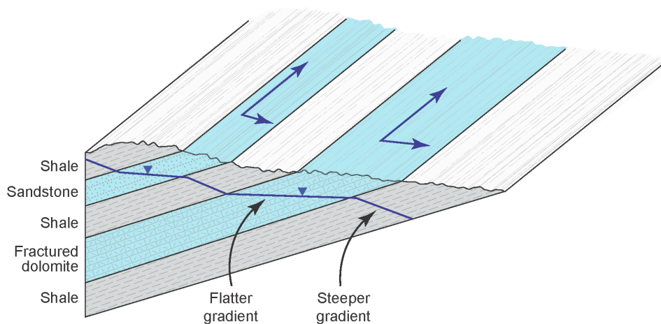
Figure 5-2. Illustration of regional-scale anisotropy within layered formation of alternating higher and lower hydraulic conductivity. Magnitudes of permeability indicated conceptually by the lengths of the arrows.
