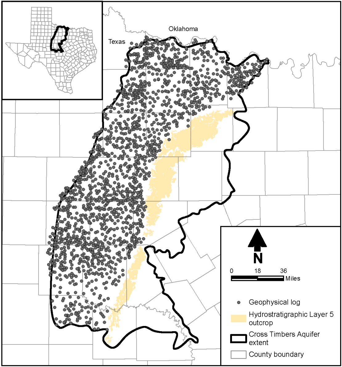
Figure 4-3. Layer 5 (Lower Cisco Group) top surface control points.
