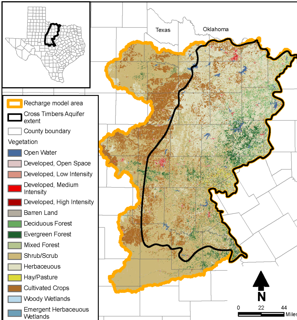
Figure 2-12. Distribution of vegetation across the study area.
