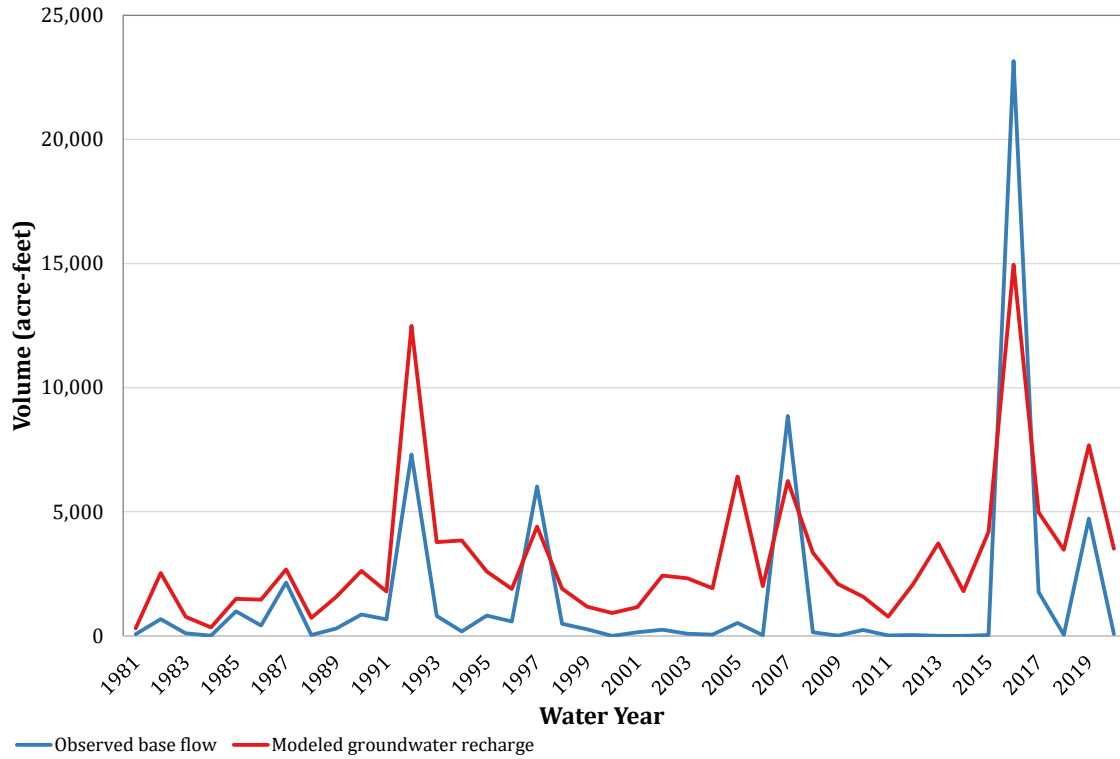
Figure C-15. Comparison of recharge simulation results to observed base flow for gauge 08086290 (Middle Brazos-Millers).
