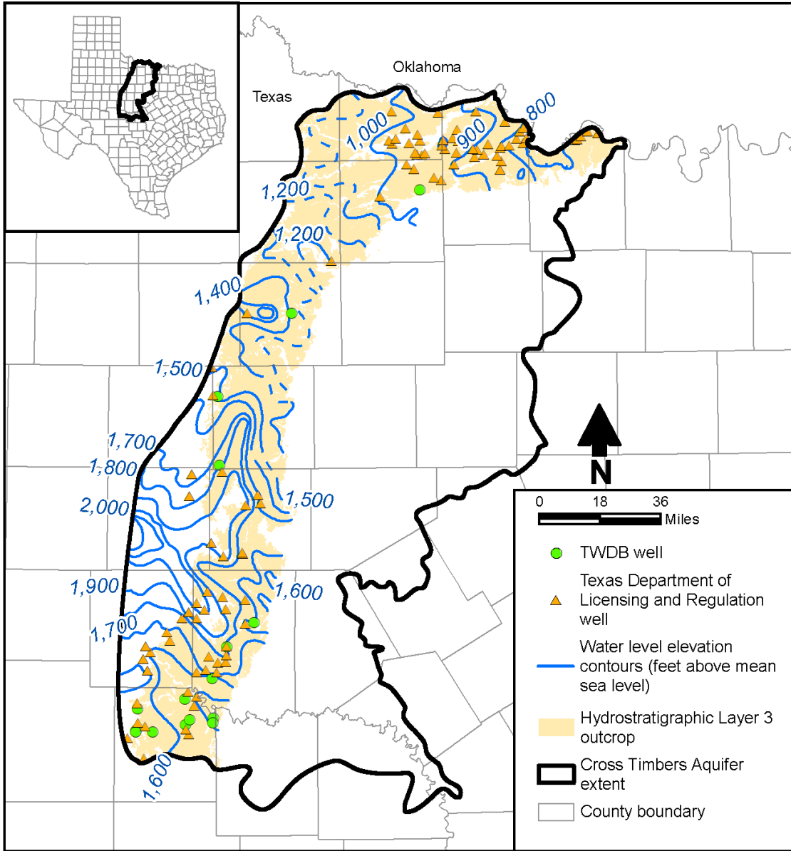
Figure 4-28. Water level contours and observed data points for 2010 through 2018 for hydrostratigraphic Layer 3 (Wichita-Albany Group).
