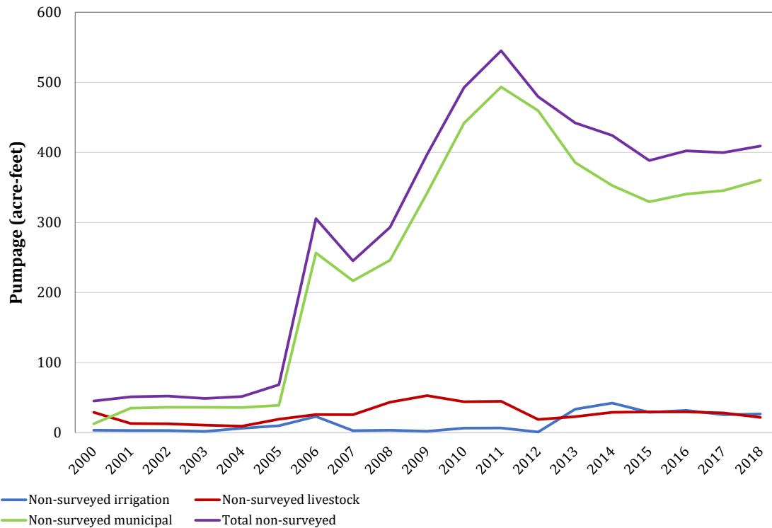
Figure 4-98. Estimated non-surveyed pumpage for the Cross Timbers Aquifer from 2000 to 2018 in Parker County.
