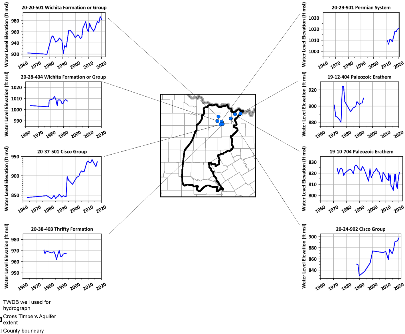
Figure 4-26. Hydrographs for selected wells in the northern portion of the Cross Timbers Aquifer.
