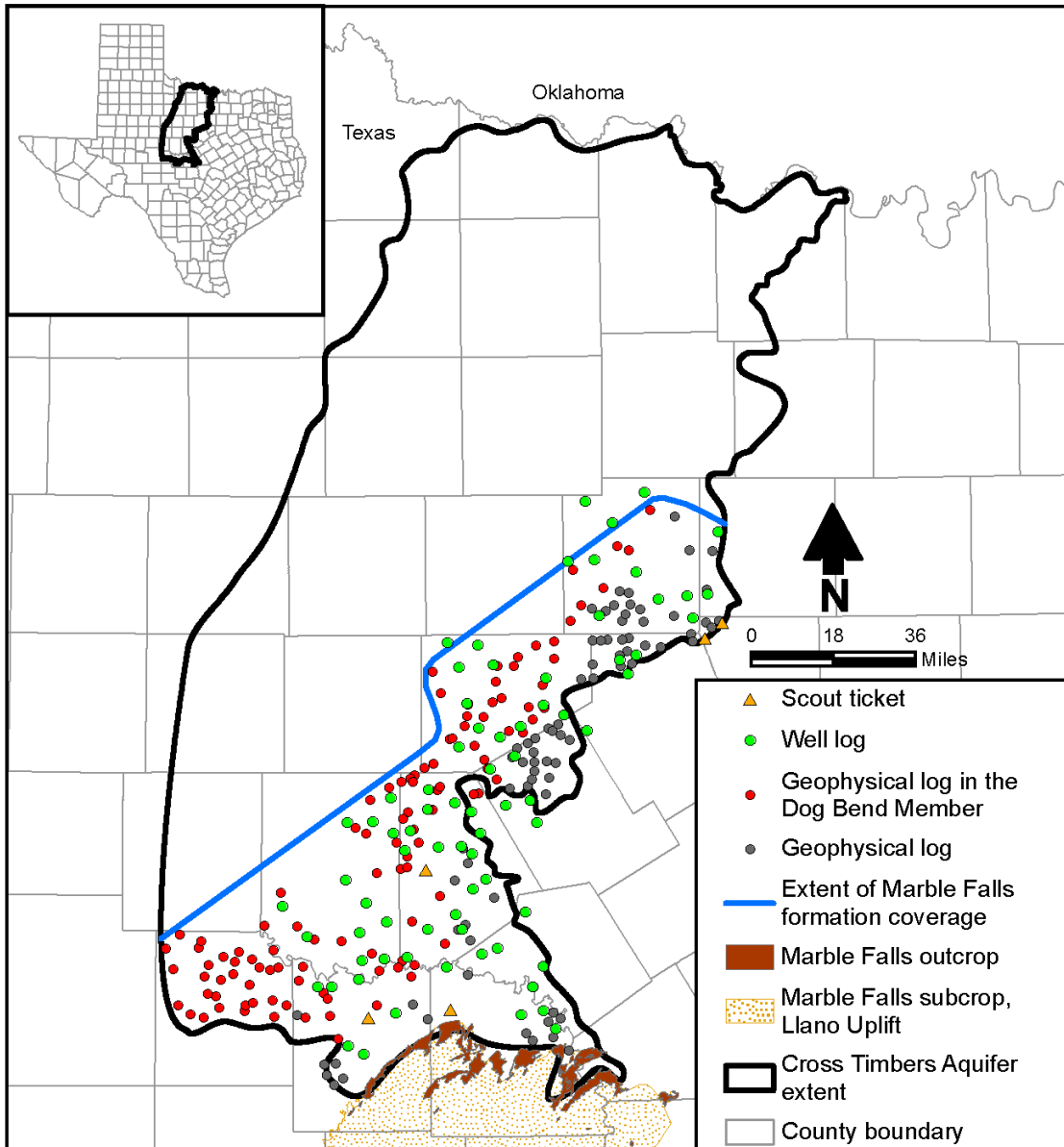
Figure 4-7. Layer 9 (Marble Falls Formation) top surface control points.
