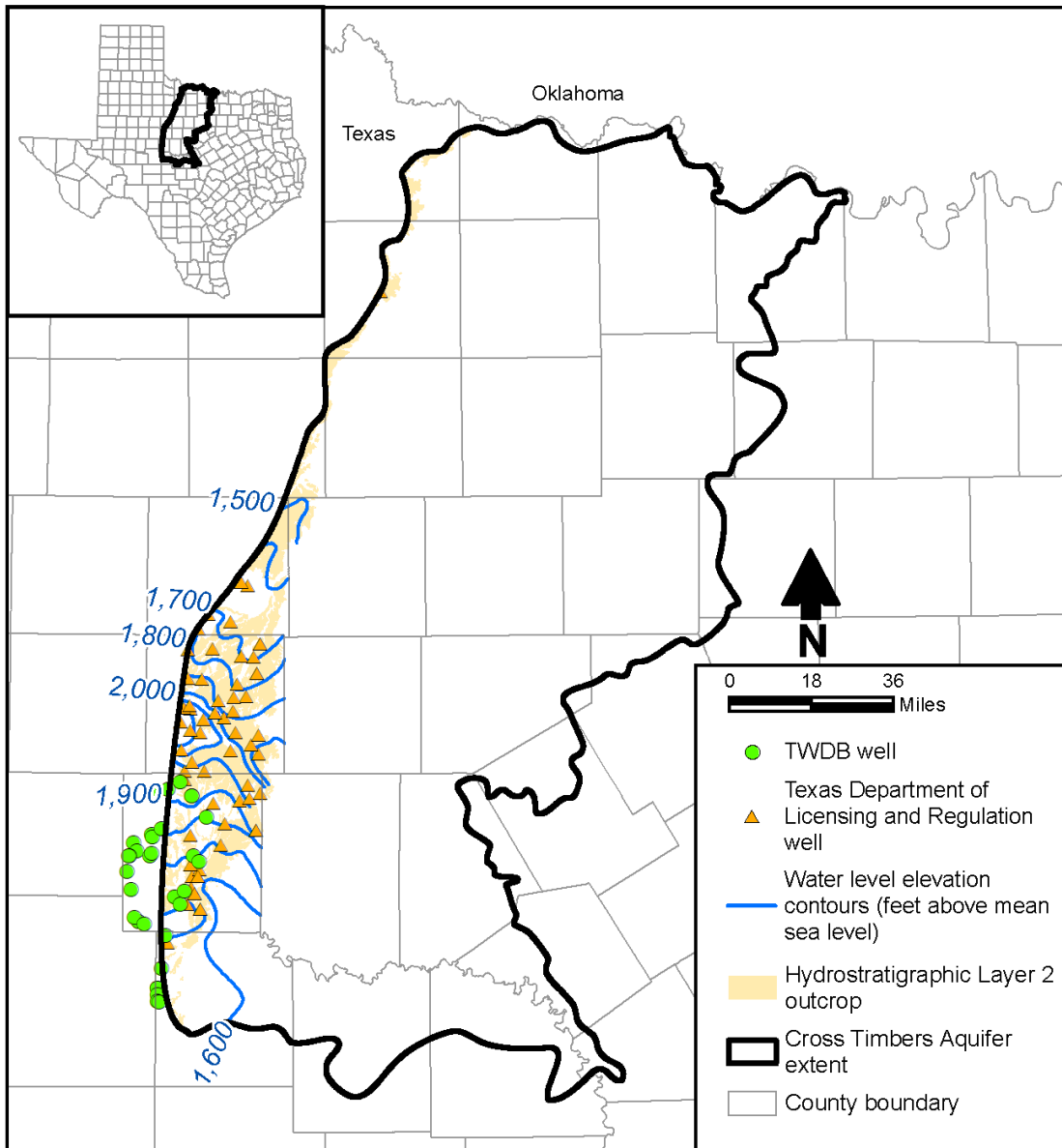
Figure 4-27. Water level contours and observed data points for 2010 through 2018 for hydrostratigraphic Layer 2 (Clear Fork Group).
