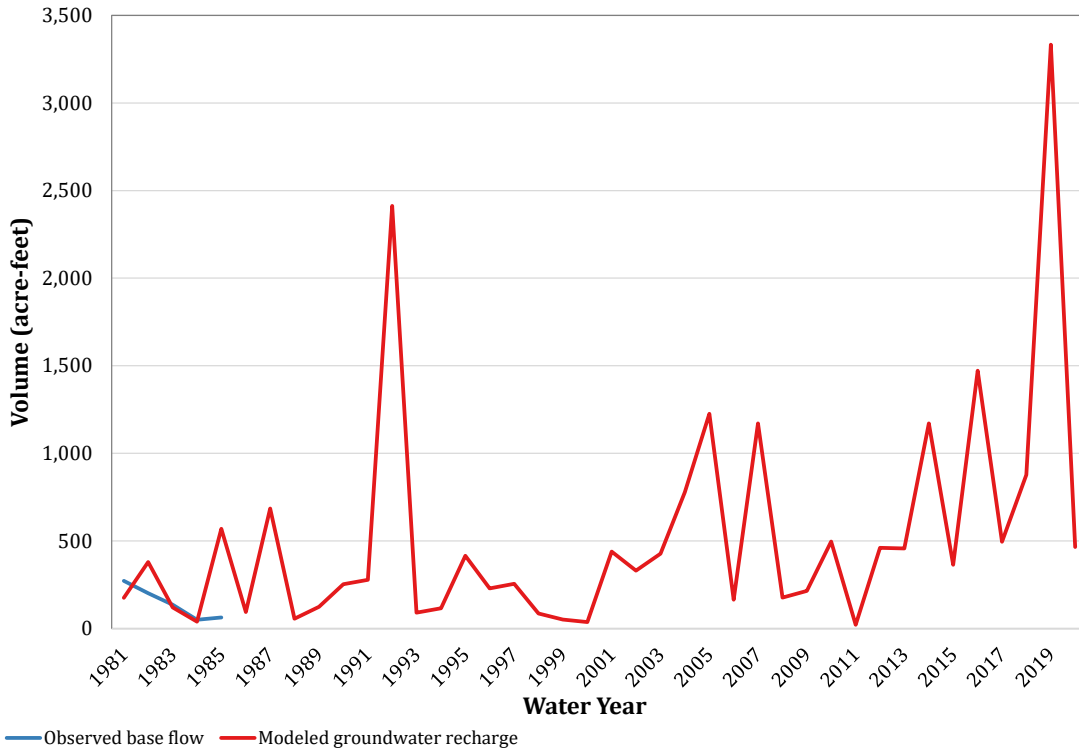
Figure C-21. Comparison of recharge simulation results to observed base flow for gauge 08144800 (San Saba).
