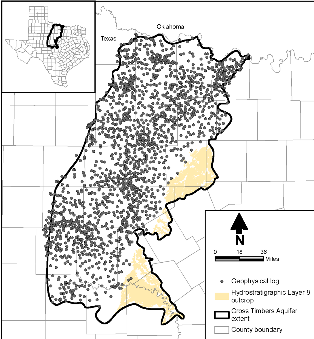
Figure 4-6. Layer 8 (Strawn and Atoka groups) top surface control points.
