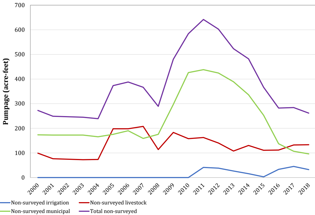
Figure 4-109. Estimated non-surveyed pumpage for the Cross Timbers Aquifer from 2000 to 2018 in Young County.
