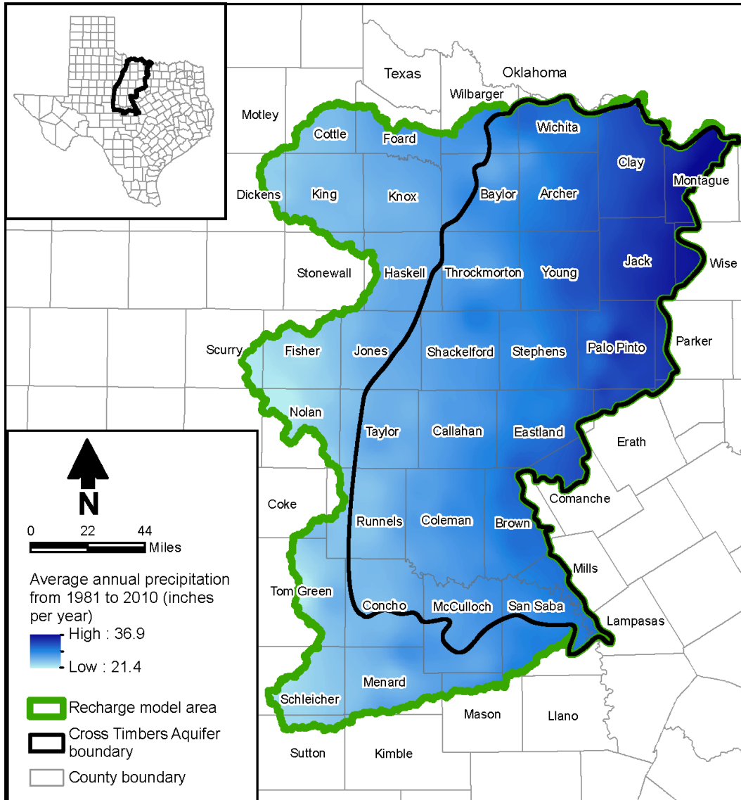
Figure 2-8. Average annual precipitation, 1981 to 2010, based on the Parameter Elevation Regression on Independent Slopes Model (PRISM).
