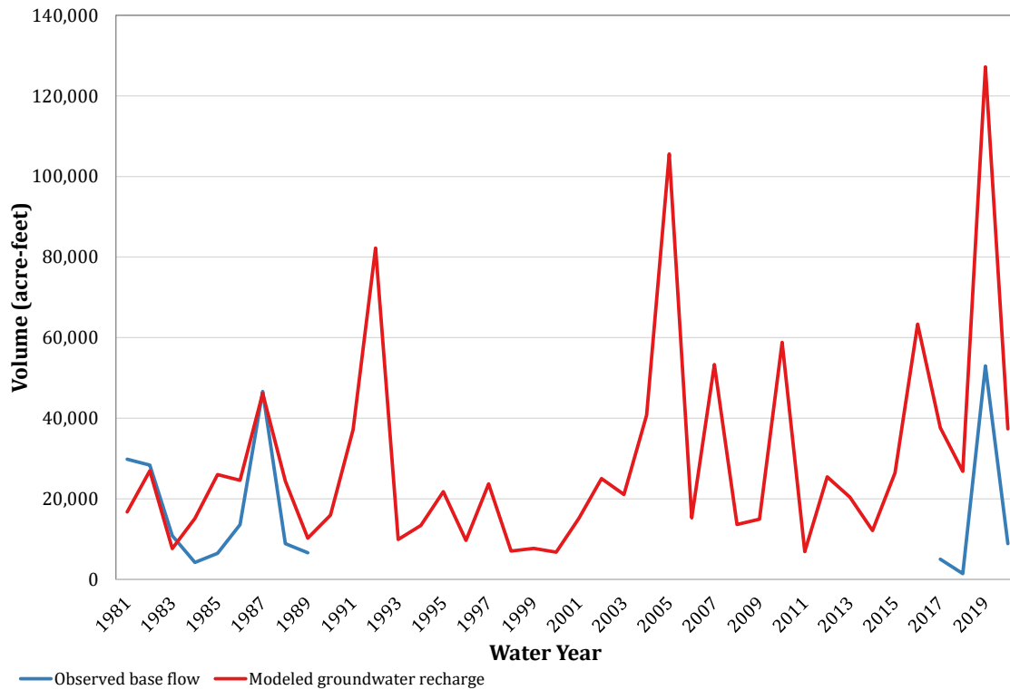
Figure C-10. Comparison of recharge simulation results to observed base flow for gauge 08083240 (Upper Clear Fork-Brazos).
