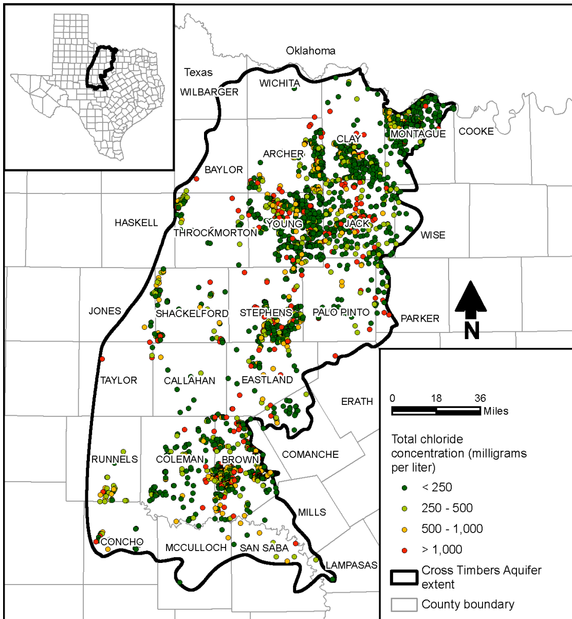
Figure 4-111. Total chloride concentration for Cross Timbers Aquifer wells.
