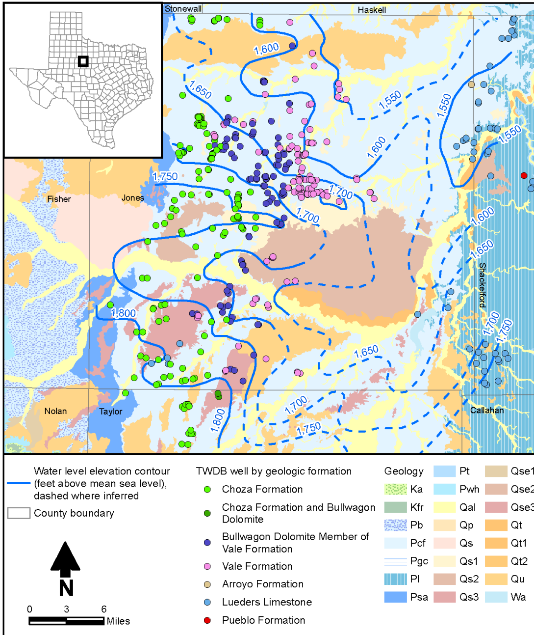
Figure 4-38. Cross Timbers Aquifer water level map for Jones County based on 1960s water level data. See Appendix A, Figure A-1b for explanation of geologic symbols.
