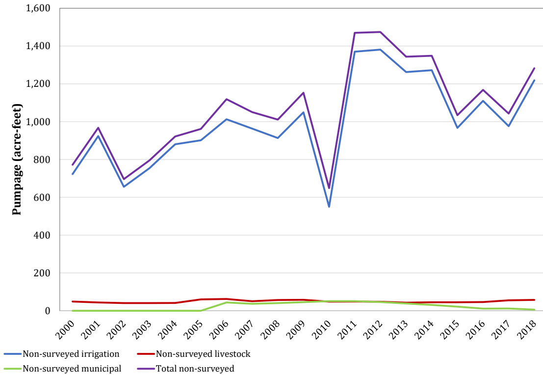
Figure 4-85. Estimated non-surveyed pumpage for the Cross Timbers Aquifer from 2000 to 2018 in Comanche County.
