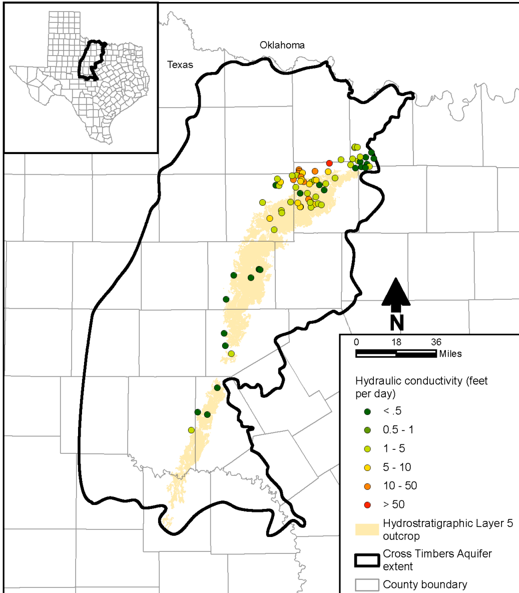
Figure 4-66. Estimated hydrostratigraphic Layer 5 (Lower Cisco Group) hydraulic conductivity from Texas Department of Licensing and Regulation specific capacity data.
