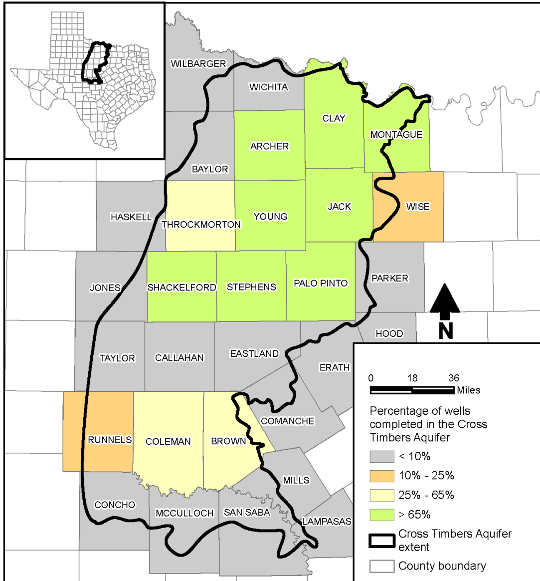
Figure 4-71. Percentage of total wells completed in the Cross Timbers Aquifer based on Ballew and French (2019).
