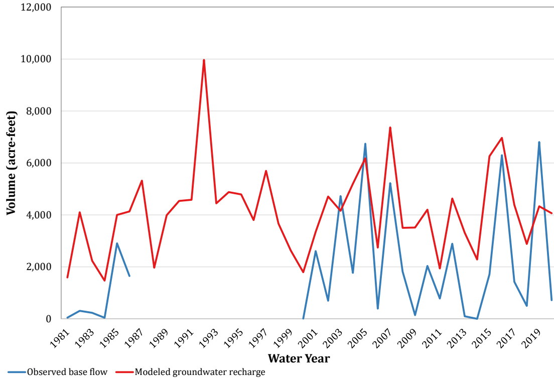
Figure C-17. Comparison of recharge simulation results to observed base flow for gauge 08099300 (Middle Brazos-Palo Pinto).
