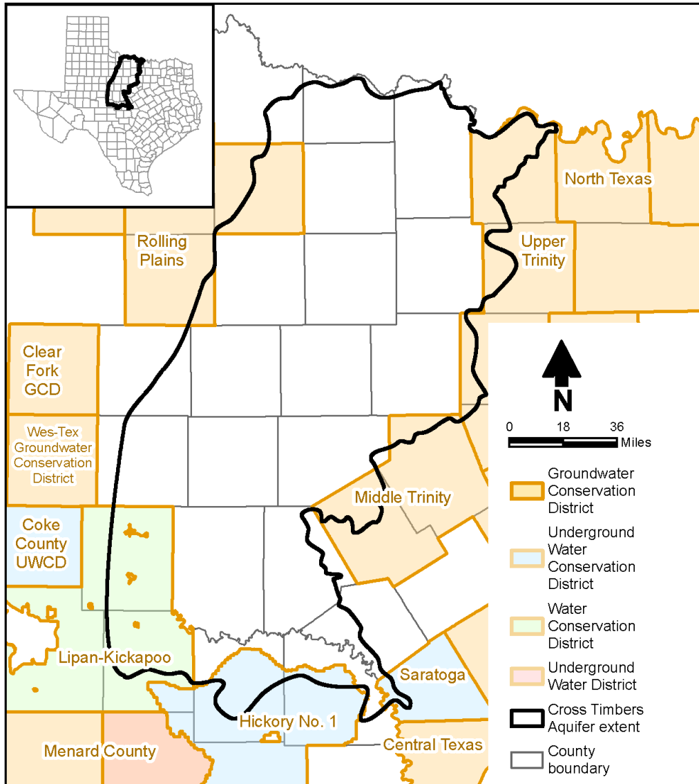
Figure 2-2. Groundwater conservation districts that encompass portions of the Cross Timbers Aquifer.
