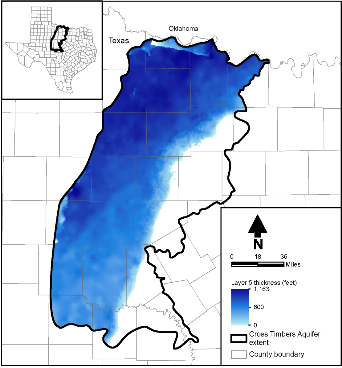
Figure 4-19. Thickness of Layer 5 (Lower Cisco Group) from Leapfrog.
