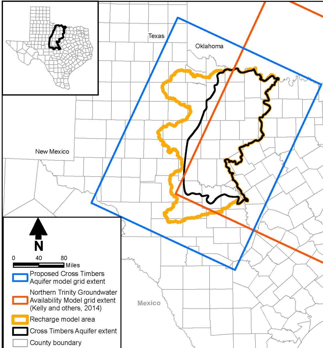
Figure 5-3. Proposed grid for Cross Timbers Aquifer groundwater modeling.
