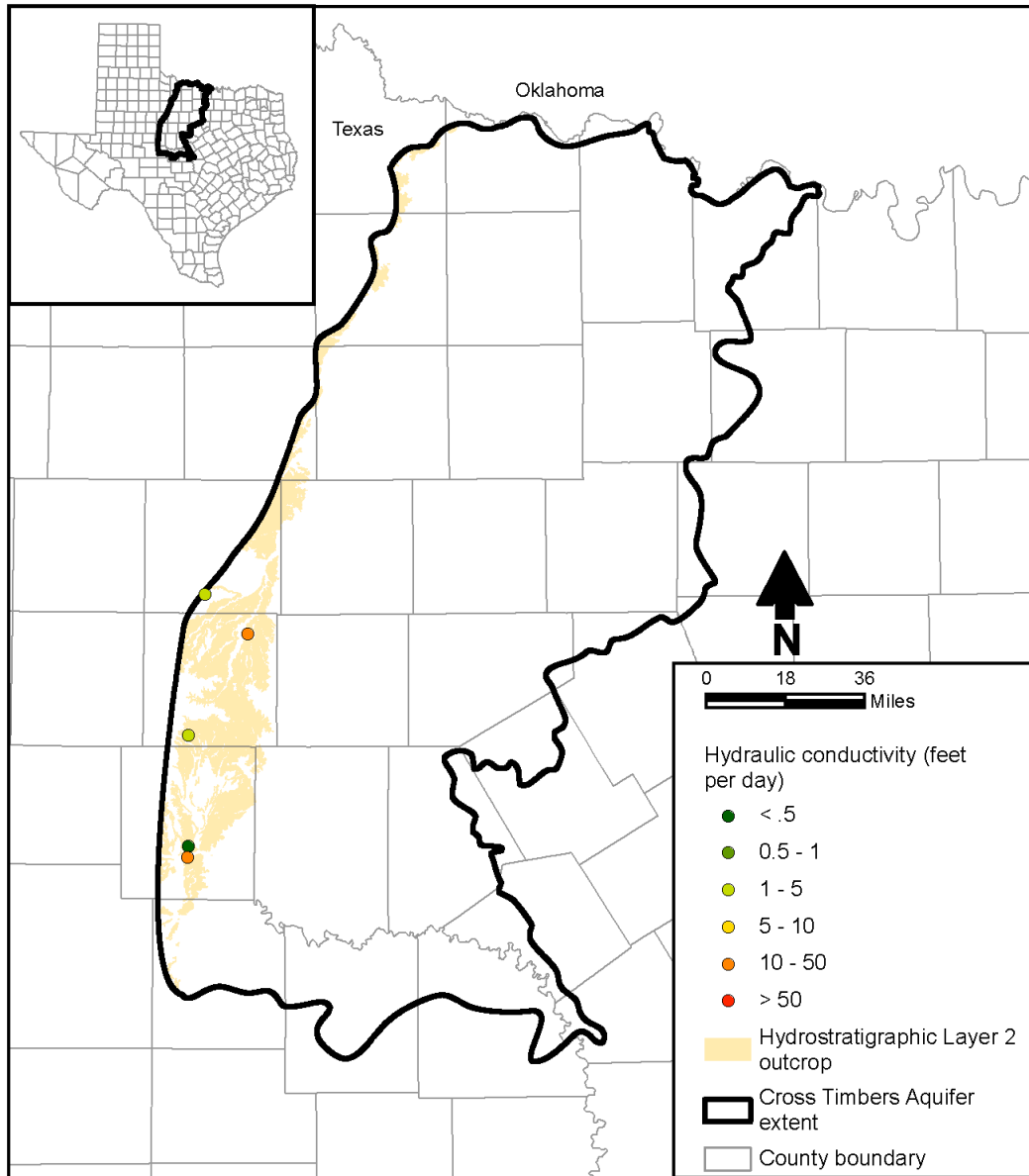
Figure 4-63. Estimated hydrostratigraphic Layer 2 (Clear Fork Group) hydraulic conductivity from Texas Department of Licensing and Regulation specific capacity data.
