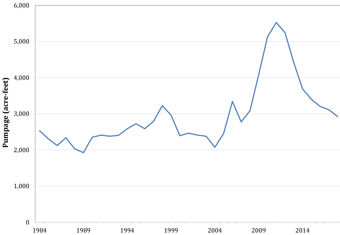
Figure 4-74. Estimated annual municipal pumpage from the Cross Timbers Aquifer.
