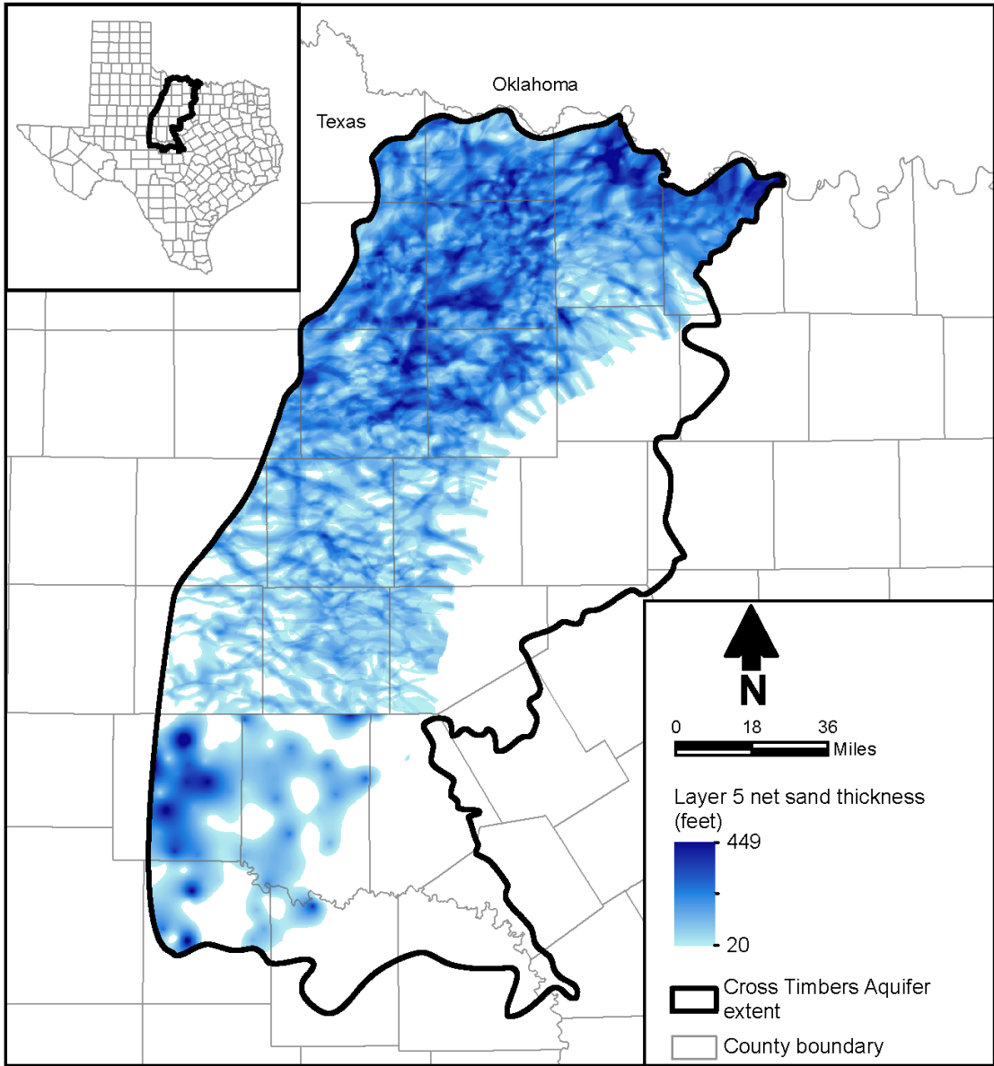
Figure 4-11. Layer 5 (Lower Cisco Group) net sand isopach.
