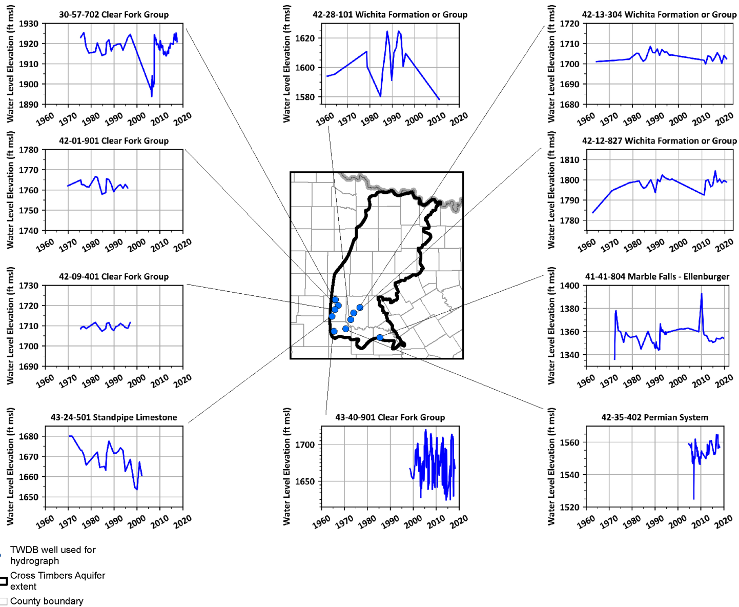
Figure 4-23. Hydrographs for selected wells in the southern portion of the Cross Timbers Aquifer.
