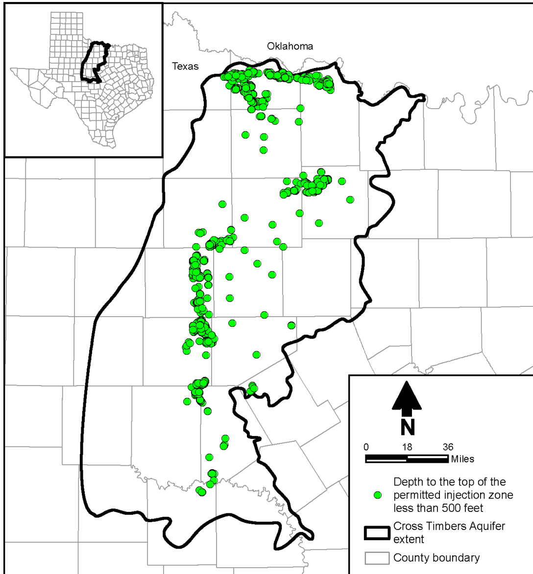
Figure 4-35. Petroleum industry injection wells with the shallowest injection zone less than 500 feet below land surface.
