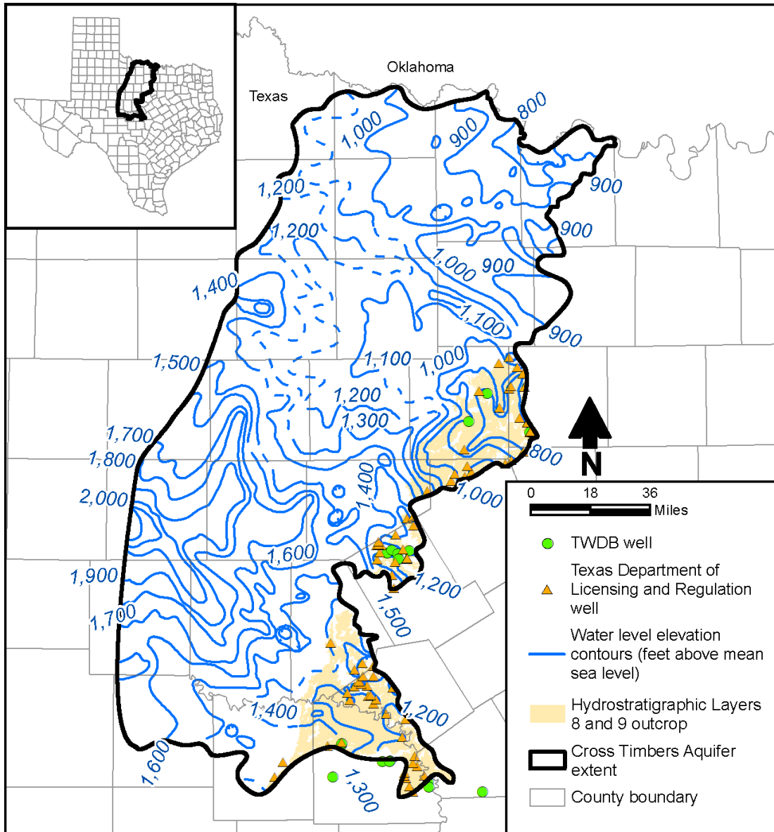
Figure 4-33. Water level contours and observed data points for 2010 through 2018 for hydrostratigraphic Layers 8 and 9 (Strawn, Atoka, and Morrow groups).
