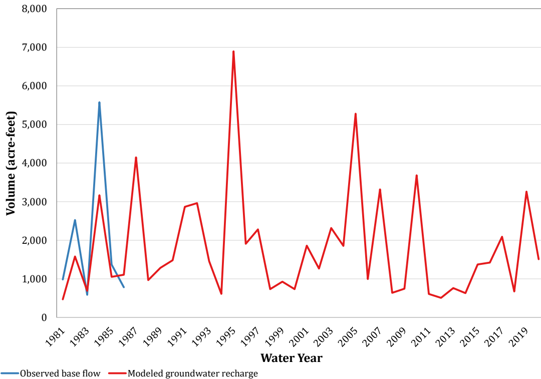
Figure C-6. Comparison of recharge simulation results to observed base flow for gauge 08082180 (Middle Brazos-Millers).
