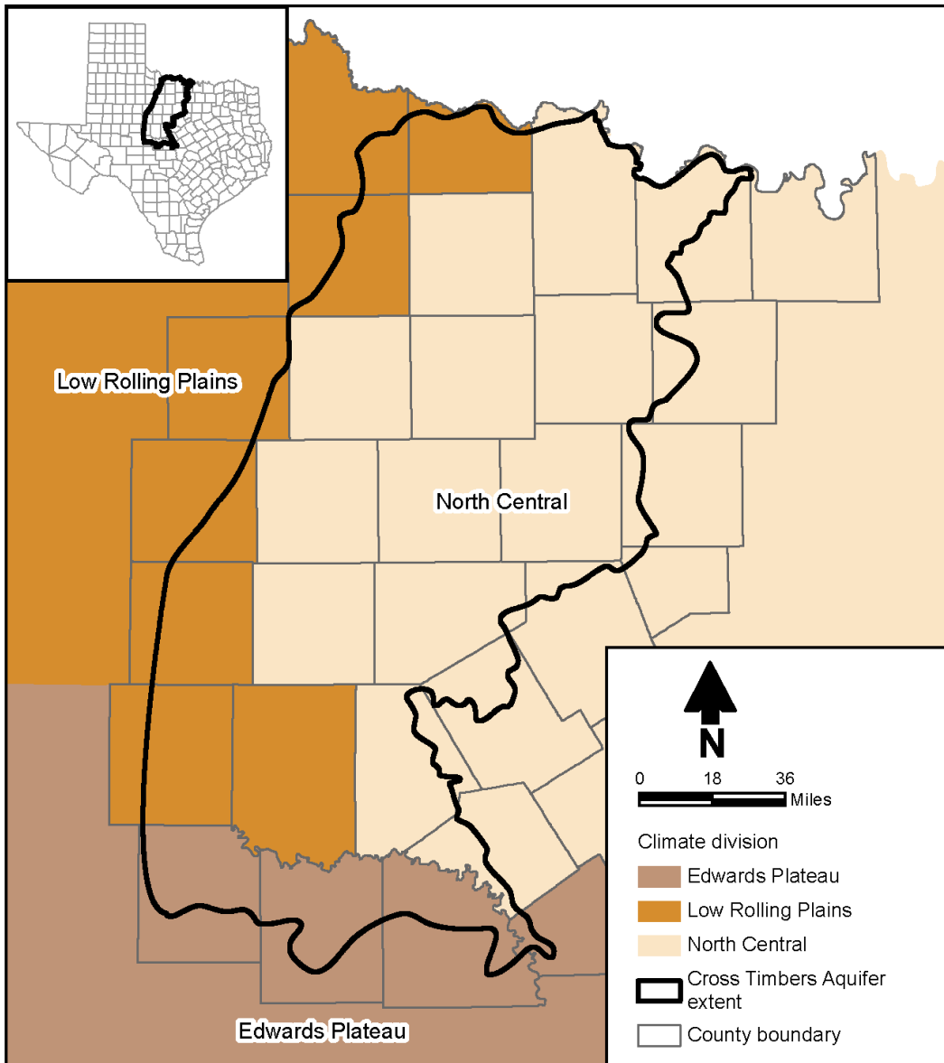
Figure 2-7. Climate divisions as delineated by the National Climatic Data Center.
