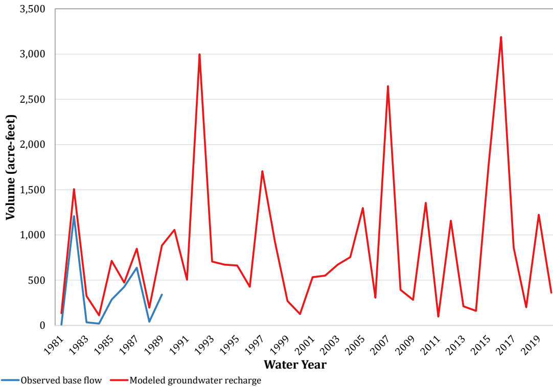
Figure C-16. Comparison of recharge simulation results to observed base flow for gauge 08088450 (Middle Brazos-Palo Pinto).
