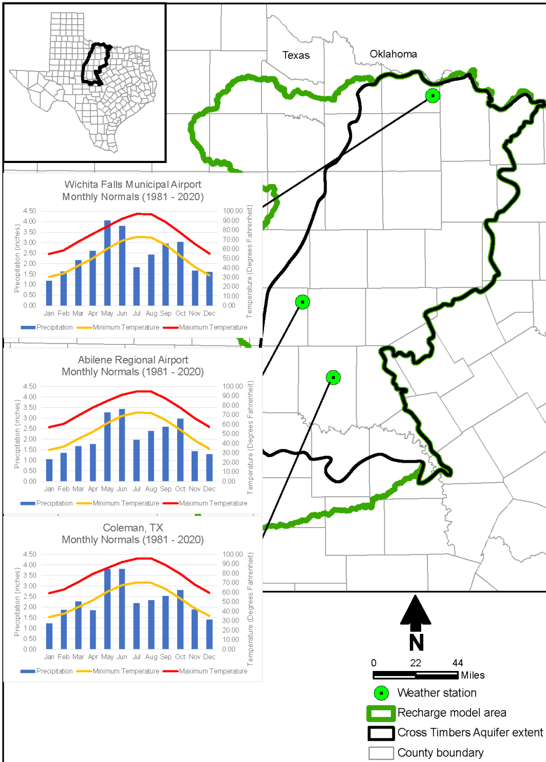
Figure 2-10. Mean monthly precipitation and temperature for selected weather stations.
