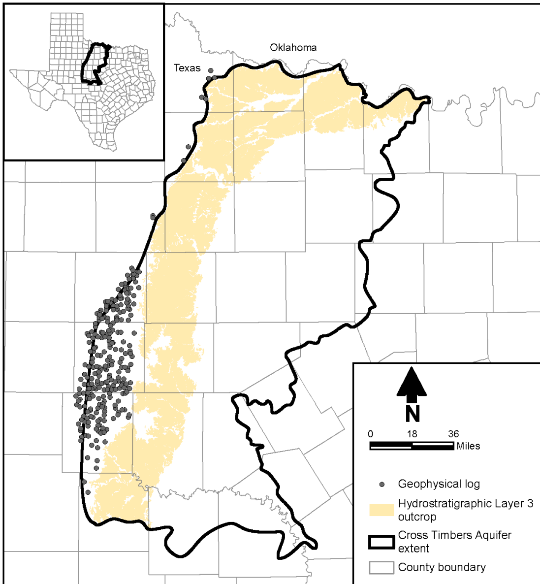
Figure 4-1. Layer 3 (Wichita-Albany Group) top surface control points.
