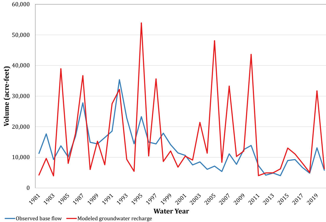
Figure C-1. Comparison of recharge simulation results to observed base flow for gauge 07311700 (Little Wichita).
