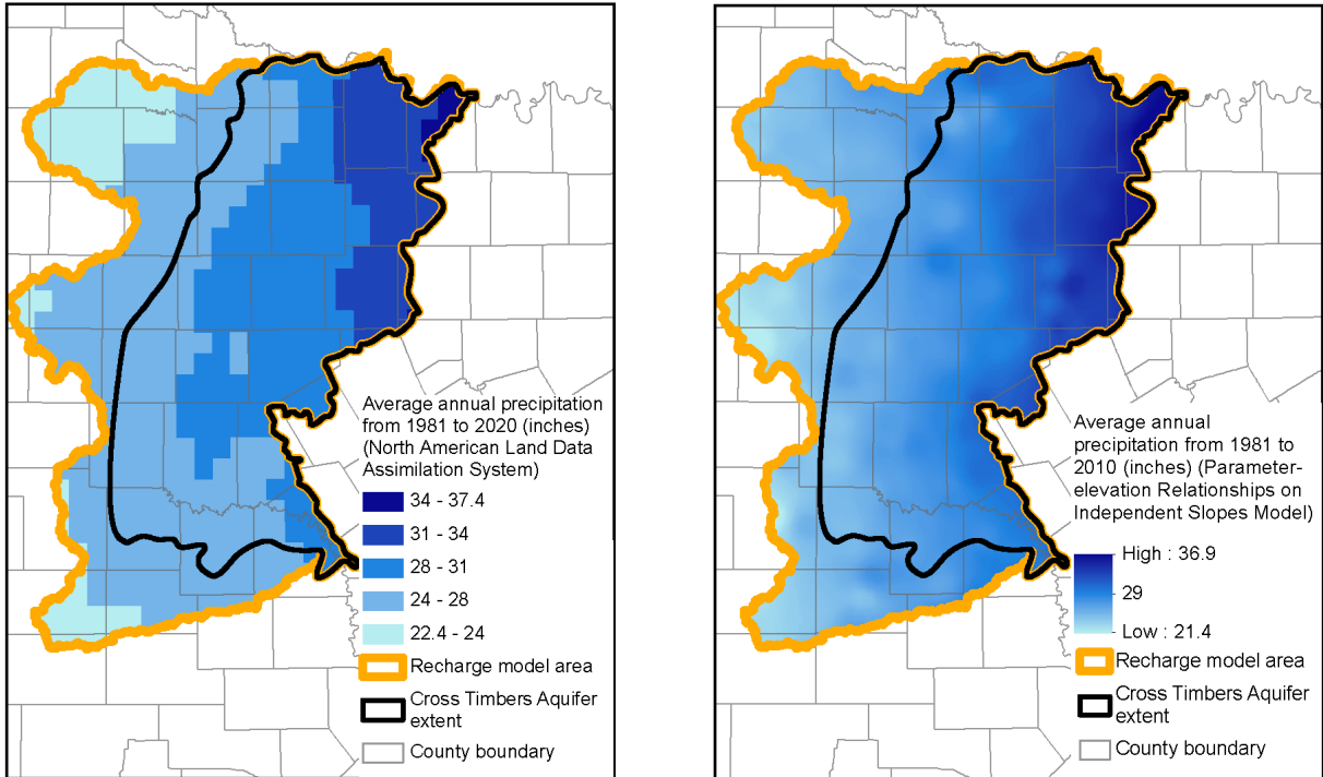
Figure 4-42. Comparison of Parameter Elevation Regression on Independent Slopes Model (PRISM) and North American Land Data Assimilation System precipitation across the watershed model area.
