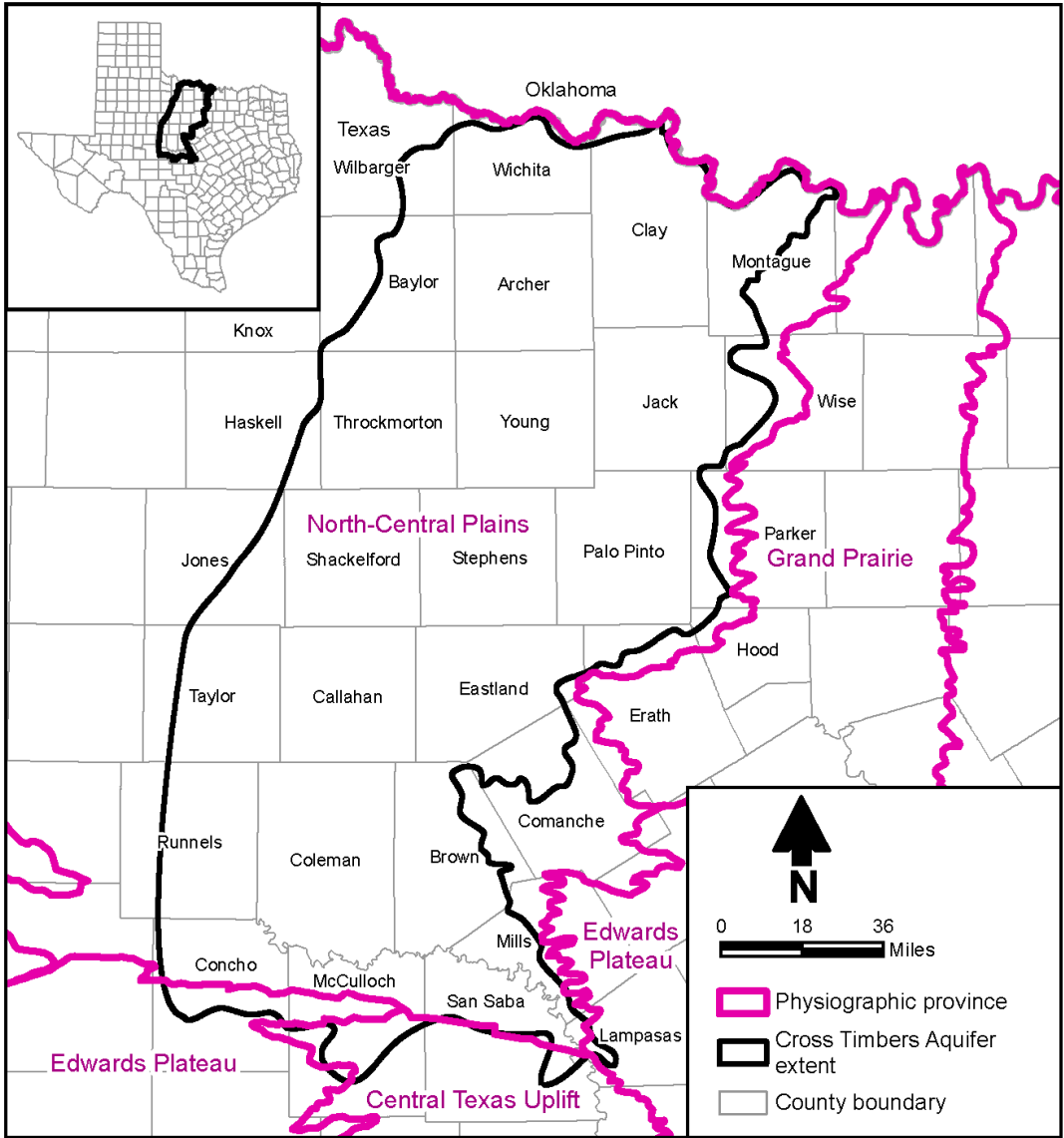
Figure 2-6. Physiographic provinces.
