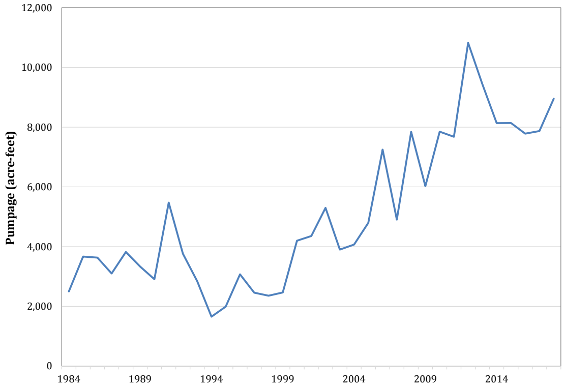
Figure 4-76. Estimated annual irrigation pumpage from the Cross Timbers Aquifer.
