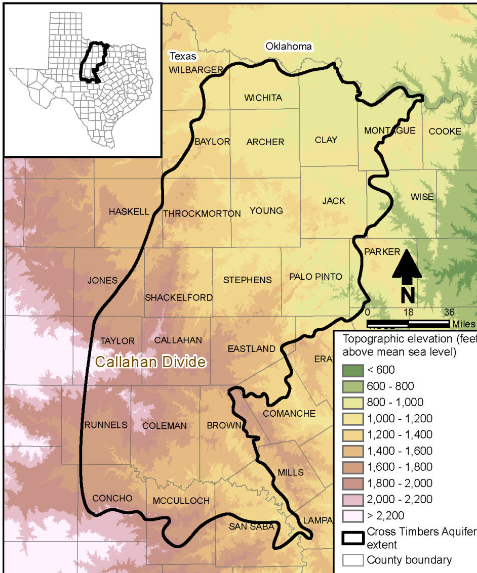
Figure 2-5. Land surface topography based on United States Geological Survey 1 arc-second (30-meter) digital elevation model.
