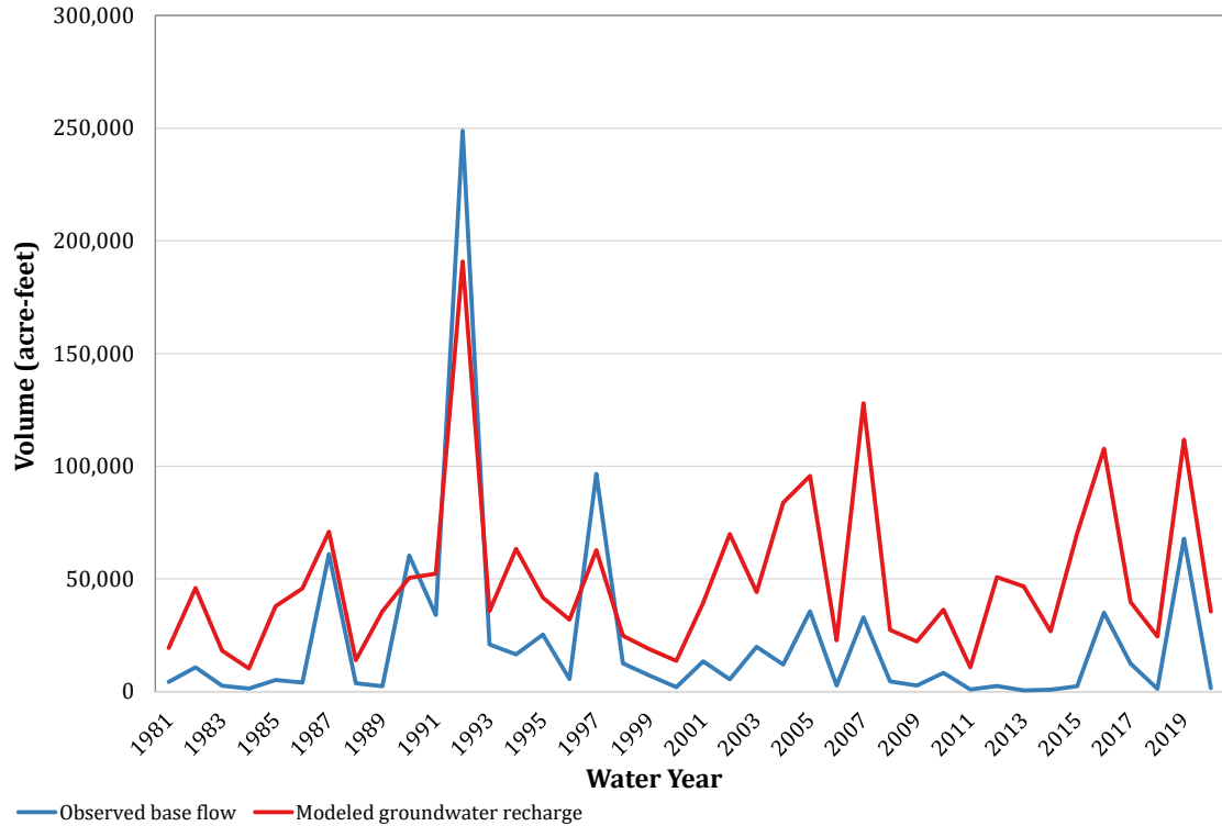
Figure C-19. Comparison of recharge simulation results to observed base flow for gauge 08143600 (Middle Colorado).
