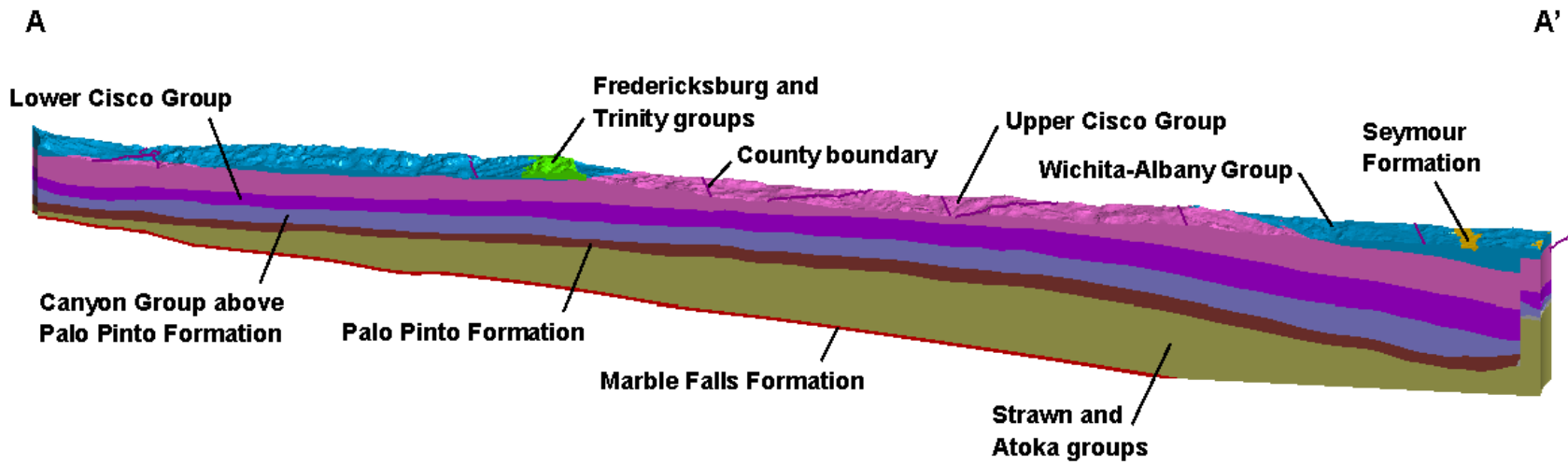
Figure 2-16. South to north geologic cross section A-A'. Location of section provided on Figure 2-15.
