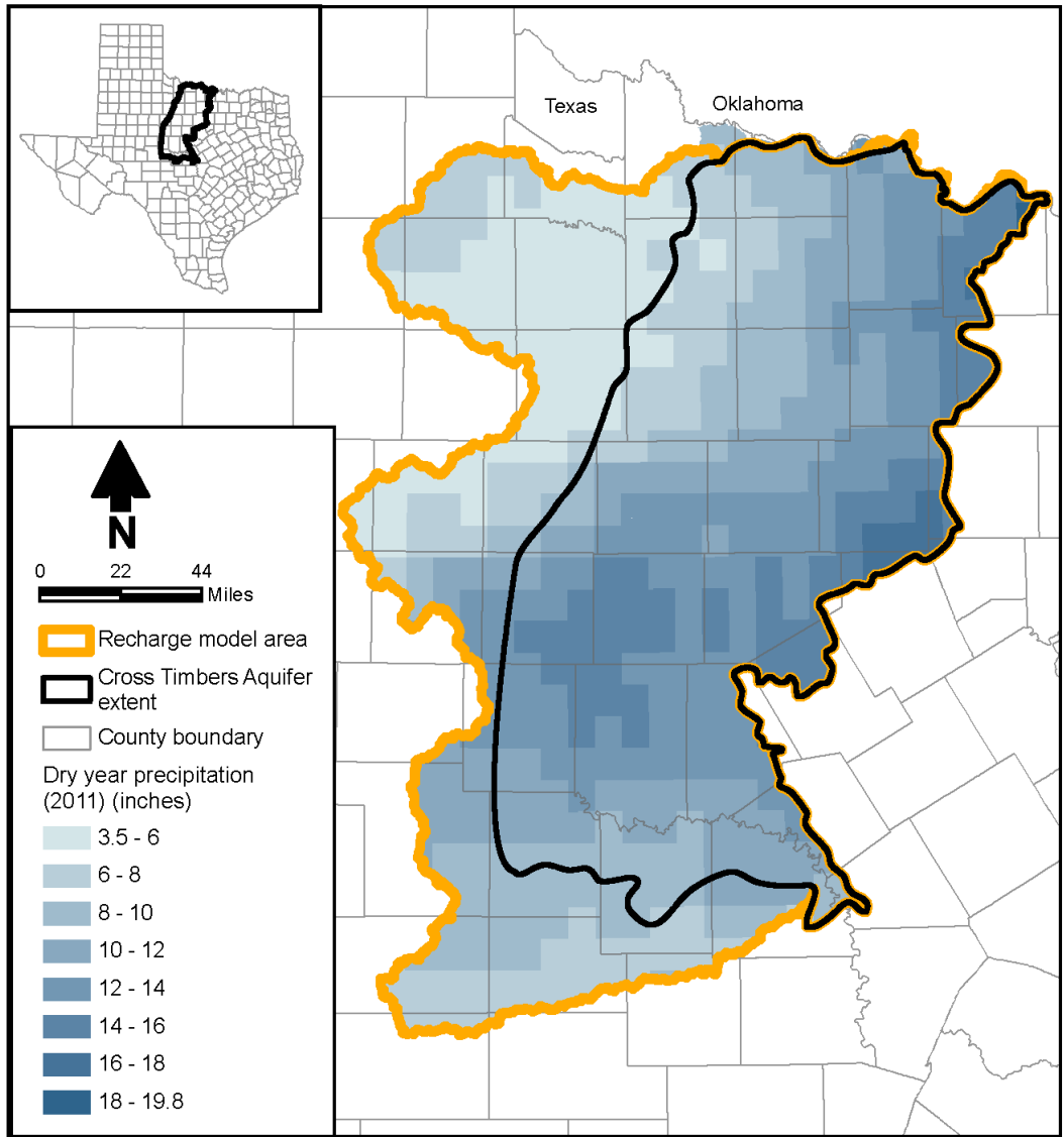
Figure 4-52. Dry year (2011) annual precipitation used in Distributed Parameter Watershed Model simulations.
