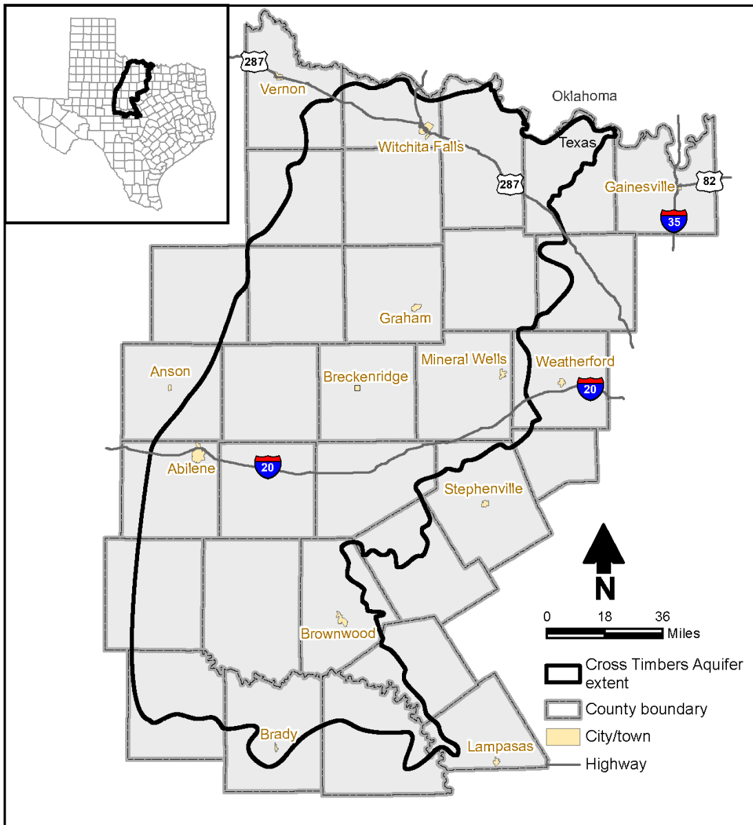
Figure 1-1. Study area with major roads, cities, and towns.
