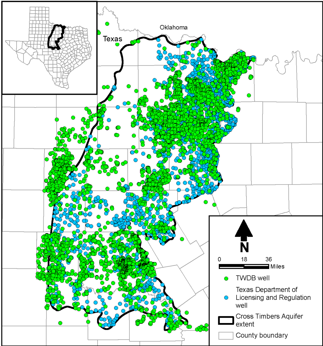
Figure 4-14. Selected TWDB groundwater database and Texas Department of Licensing and Regulation water wells.
