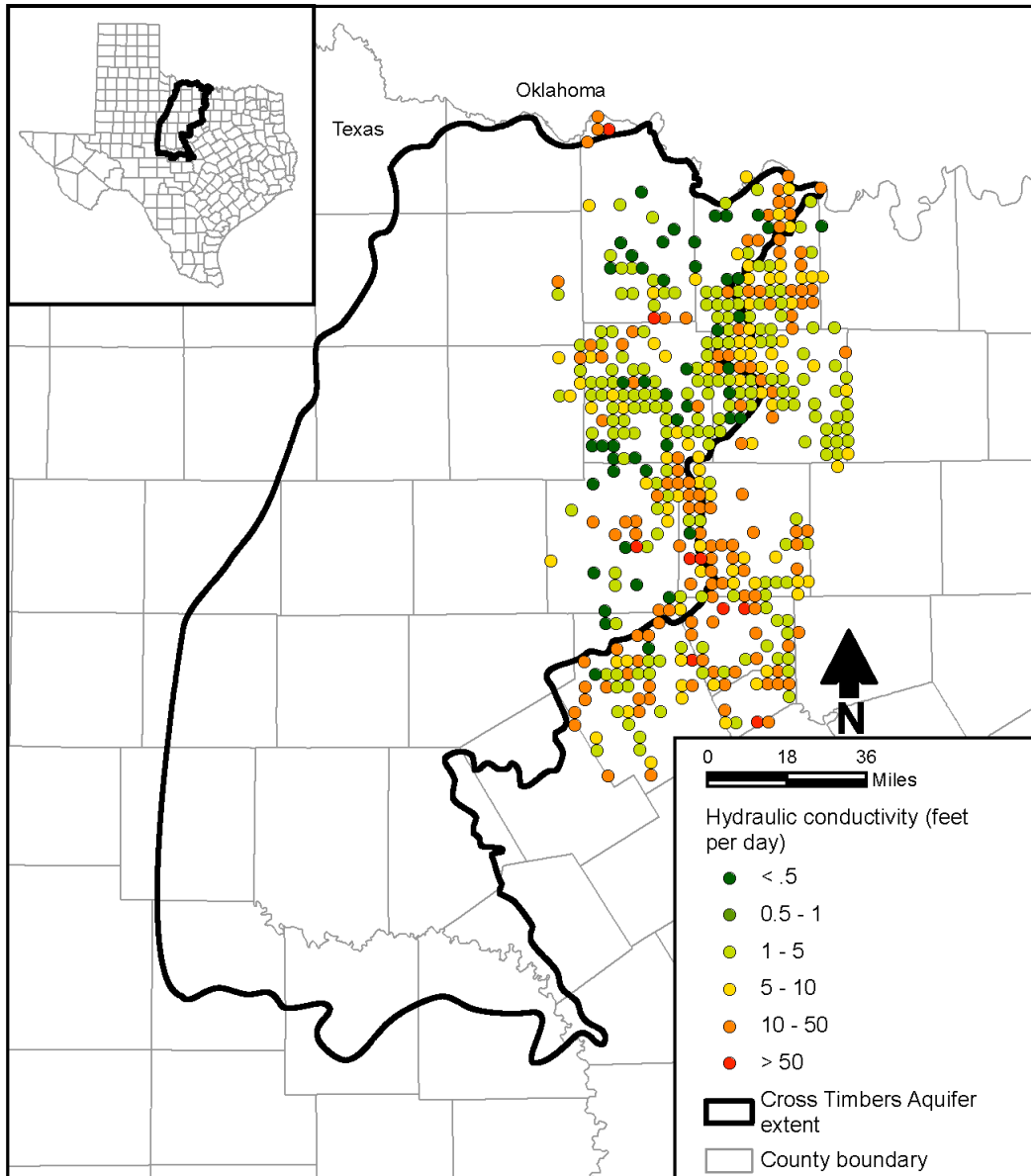
Figure 4-70. Estimated Cross Timbers Aquifer hydraulic conductivity from Texas Department of Licensing and Regulation specific capacity data compiled by Nicot and others (2013).
