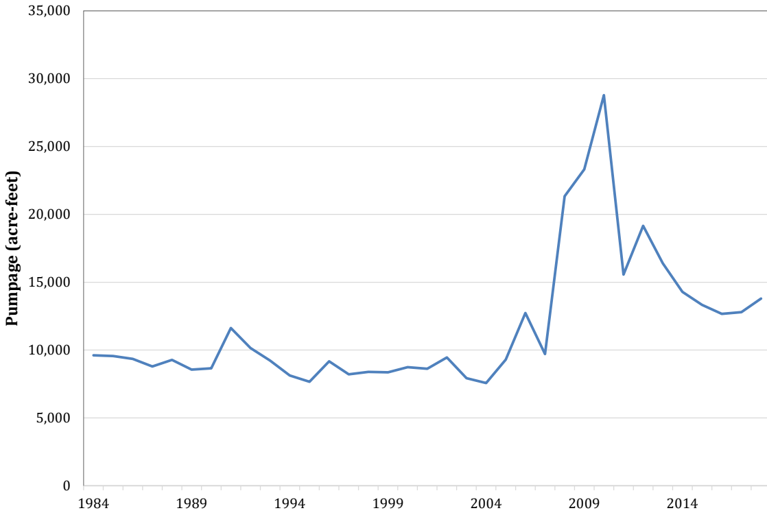
Figure 4-73. Estimated total annual pumpage from the Cross Timbers Aquifer.
