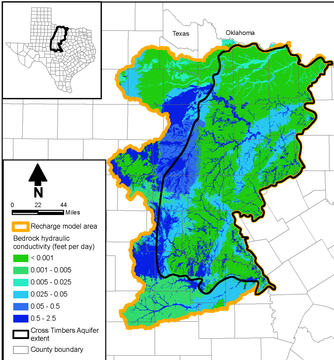
Figure 4-45. Final bedrock vertical hydraulic conductivity used the Distributed Parameter Watershed Model simulations.
