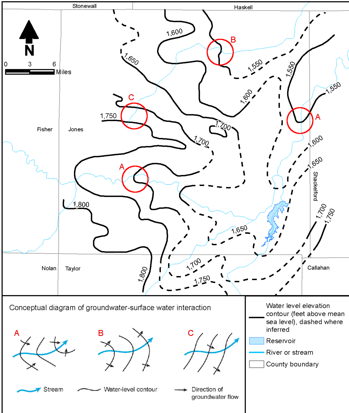
Figure 4-60. Example of using water level contour maps to interpret where base flow occurs to streams. Diagram A illustrates groundwater inflow to a stream. Diagram B illustrates surface water flowing from the stream to the adjacent groundwater. Diagram C illustrates a case of no apparent hydraulic connection.
