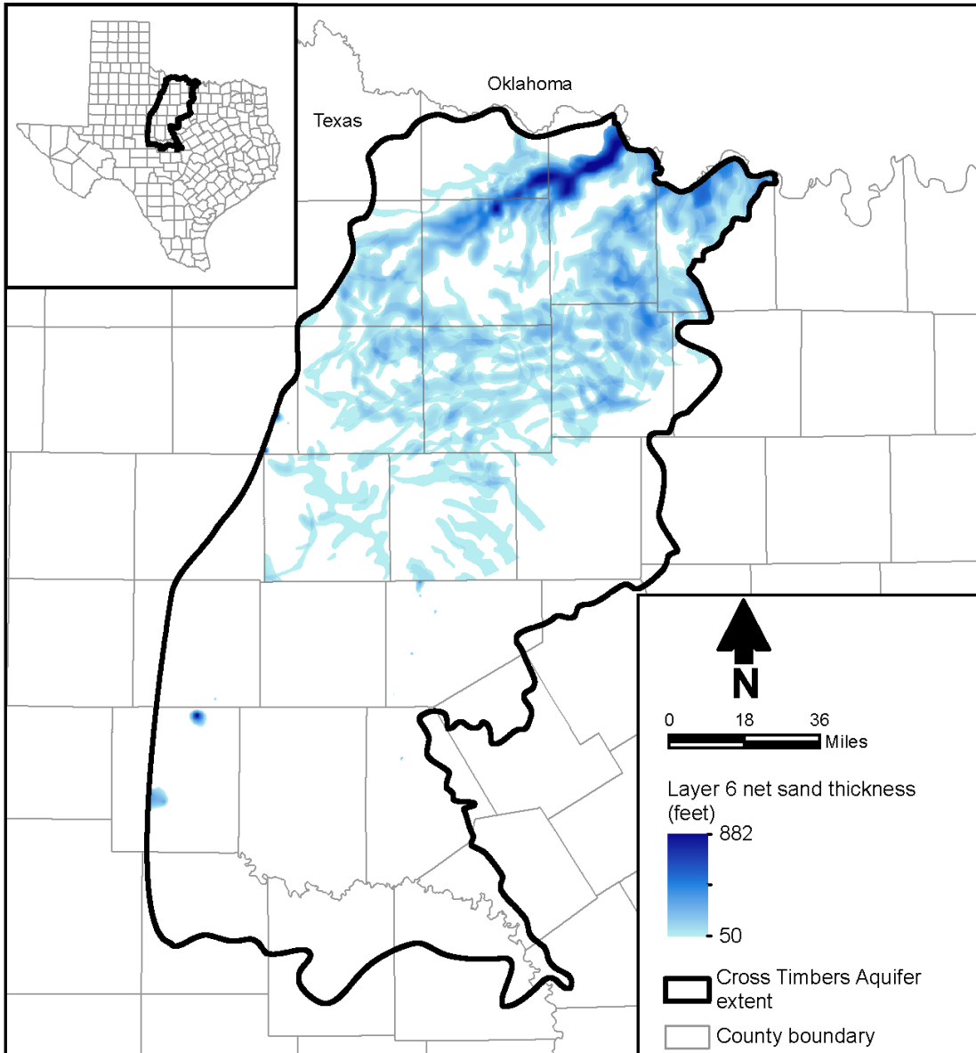
Figure 4-12. Layer 6 (Canyon Group above the Palo Pinto Formation) net sand isopach.
