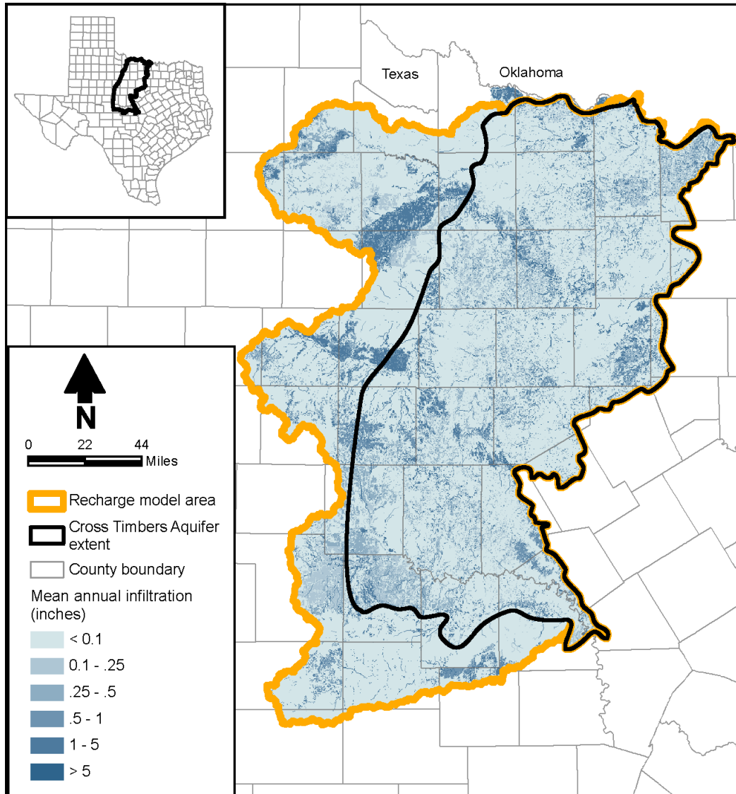
Figure 4-51. Mean annual simulated recharge, 1981 through 2020.
