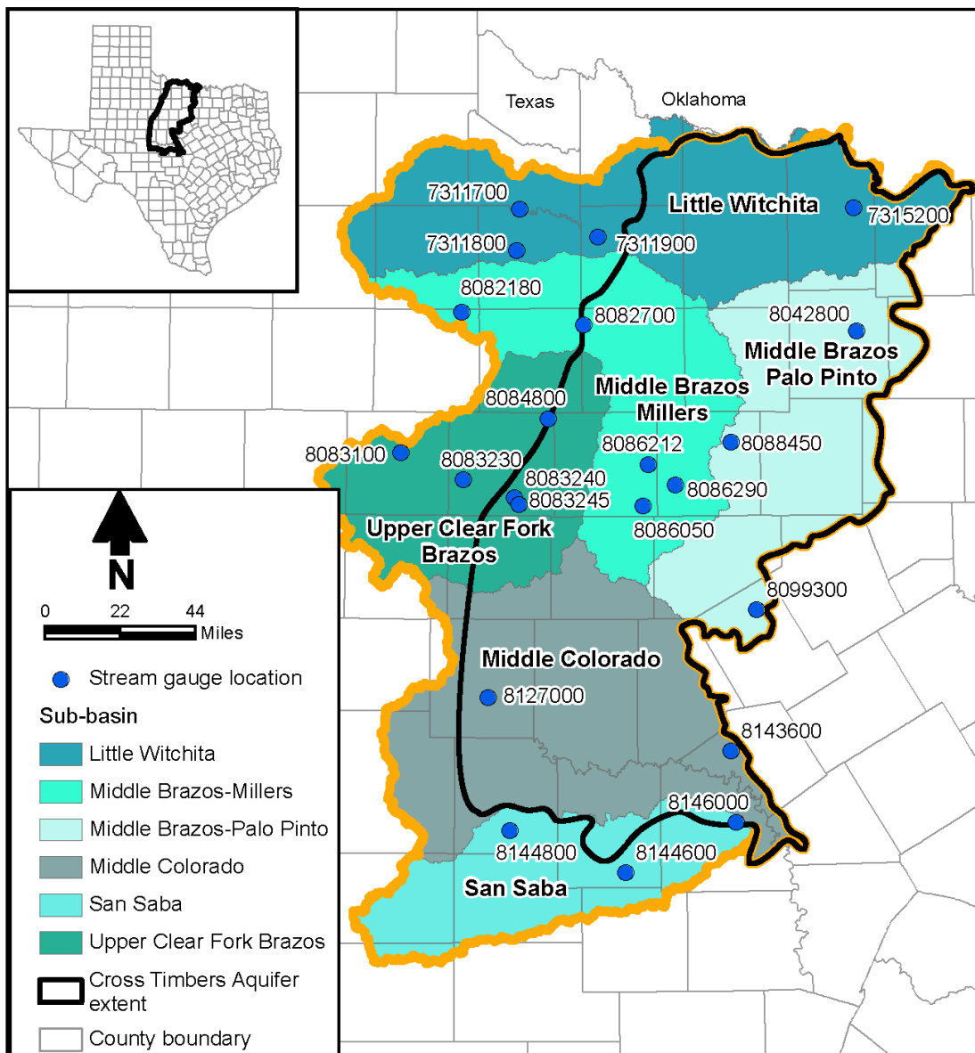
Figure 4-41. Distributed Parameter Watershed Model sub-basin simulation domains and gauges used for base flow estimation.
