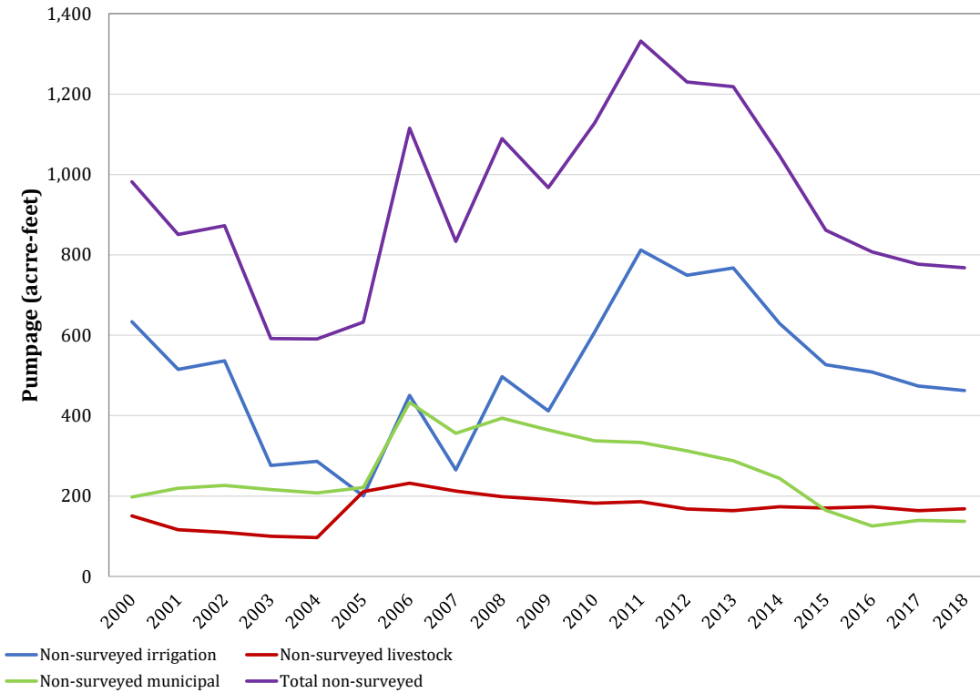
Figure 4-83. Estimated non-surveyed pumpage for the Cross Timbers Aquifer from 2000 to 2018 in Clay County.
