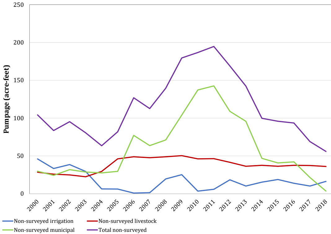
Figure 4-81. Estimated non-surveyed pumpage for the Cross Timbers Aquifer from 2000 to 2018 in Brown County.
