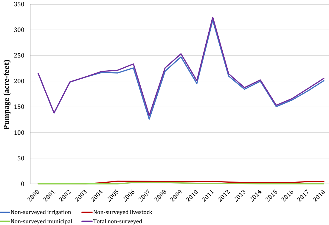
Figure 4-107. Estimated non-surveyed pumpage for the Cross Timbers Aquifer from 2000 to 2018 in Wilbarger County.
