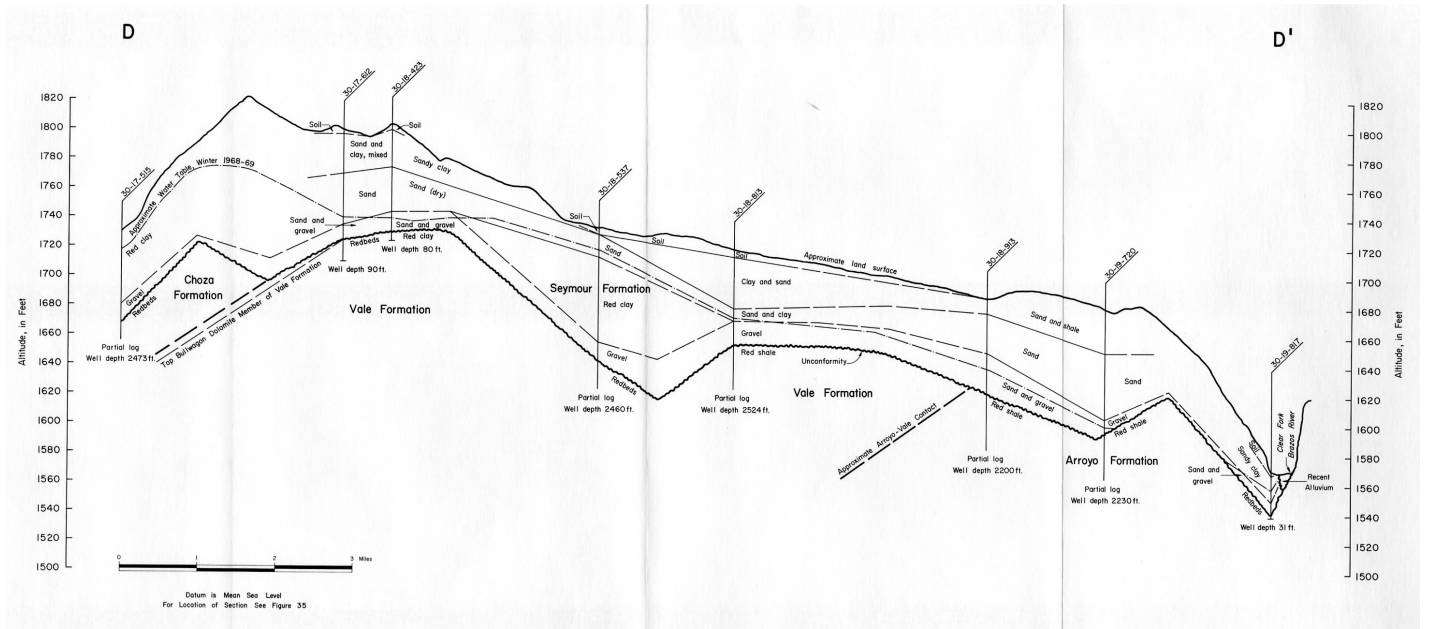
Figure B-1. Cross section D-D' from Price (1978). Cross section location is shown on Figure 4-39. Note that the image is the best available.
