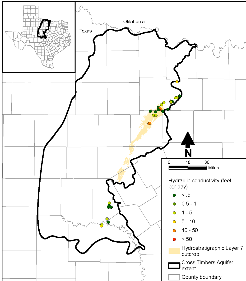
Figure 4-68. Estimated hydrostratigraphic Layer 7 (Palo Pinto Formation) hydraulic conductivity from Texas Department of Licensing and Regulation specific capacity data.
