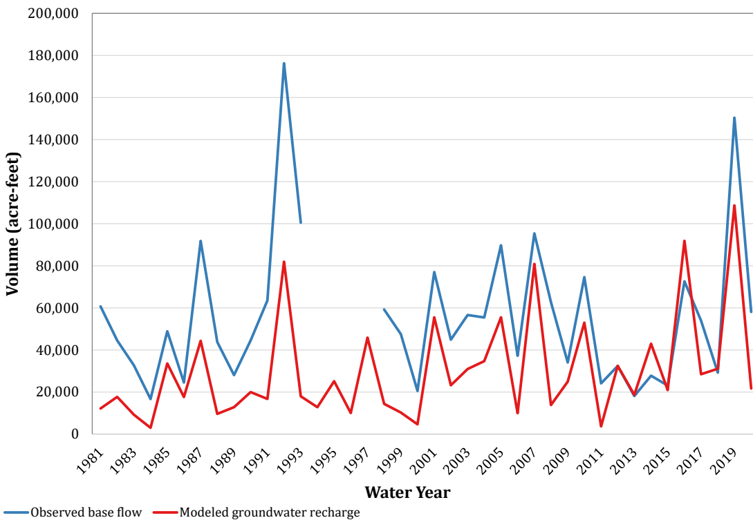
Figure C-22. Comparison of recharge simulation results to observed base flow for gauge 08146000 (San Saba).
