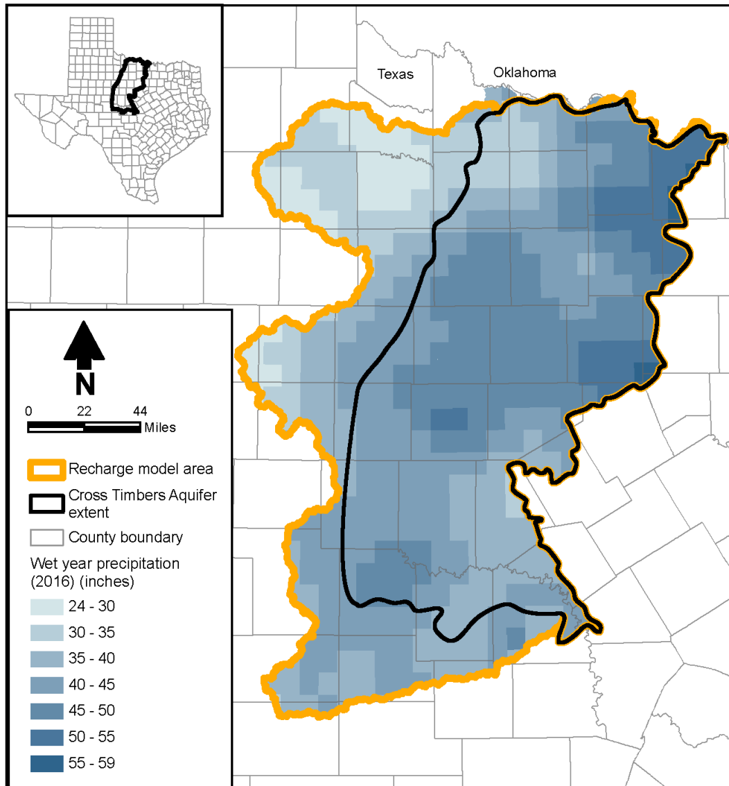
Figure 4-54. Wet year (2016) annual precipitation used in Distributed Parameter Watershed Model simulations.
