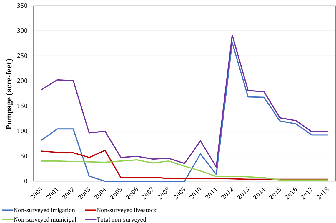
Figure 4-102. Estimated non-surveyed pumpage for the Cross Timbers Aquifer from 2000 to 2018 in Shackelford County.
