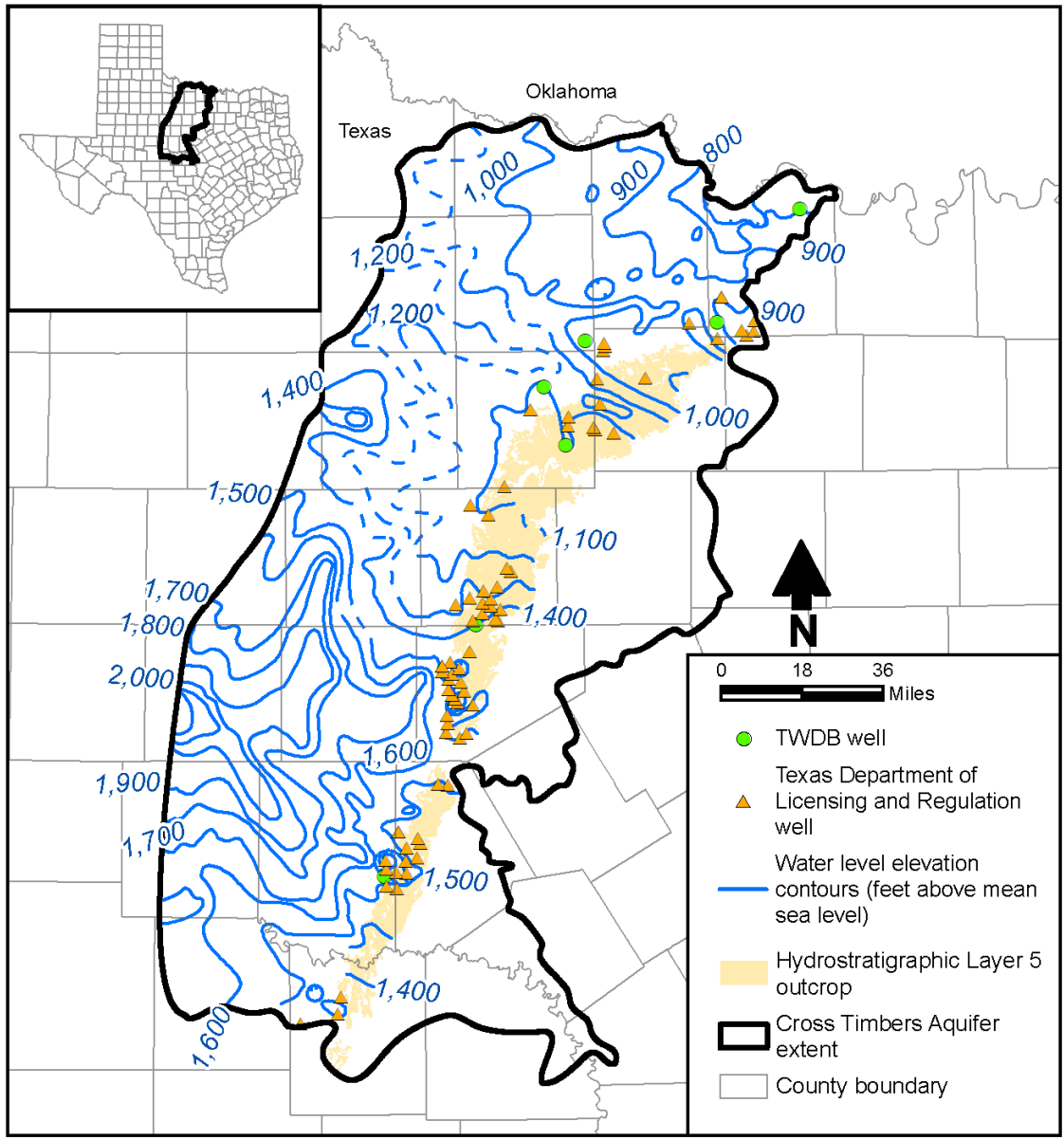
Figure 4-30. Water level contours and observed data points for 2010 through 2018 for hydrostratigraphic Layer 5 (Lower Cisco Group).
