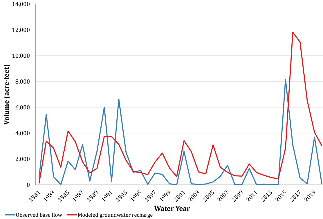
Figure 4-46. Comparison of recharge simulation results to observed base flow for gauge 07315200 (Little Wichita).
