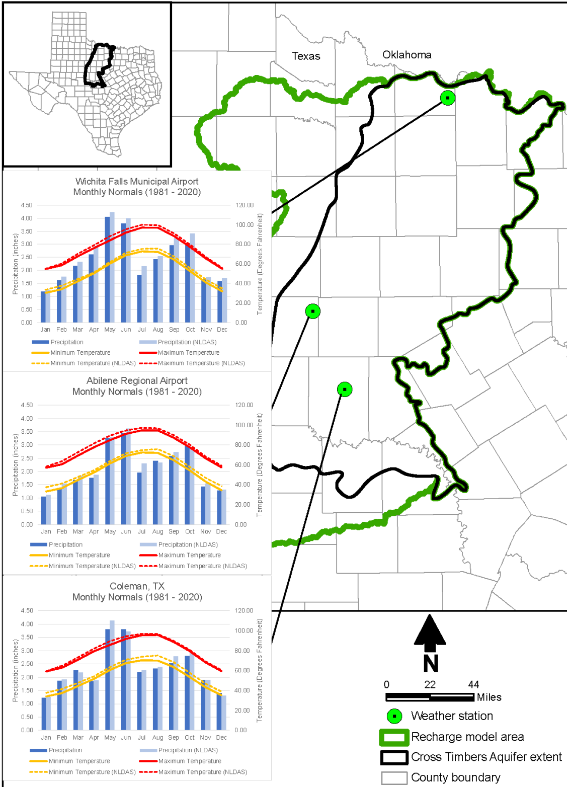
Figure 4-43. Comparison of North American Land Data Assimilation System precipitation and temperature with observed data at selected weather stations.
