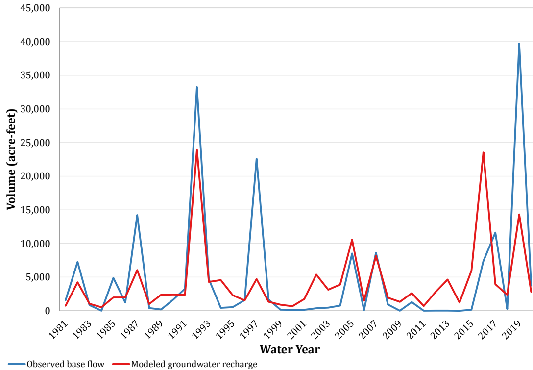
Figure C-14. Comparison of recharge simulation results to observed base flow for gauge 08086212 (Middle Brazos-Millers).
