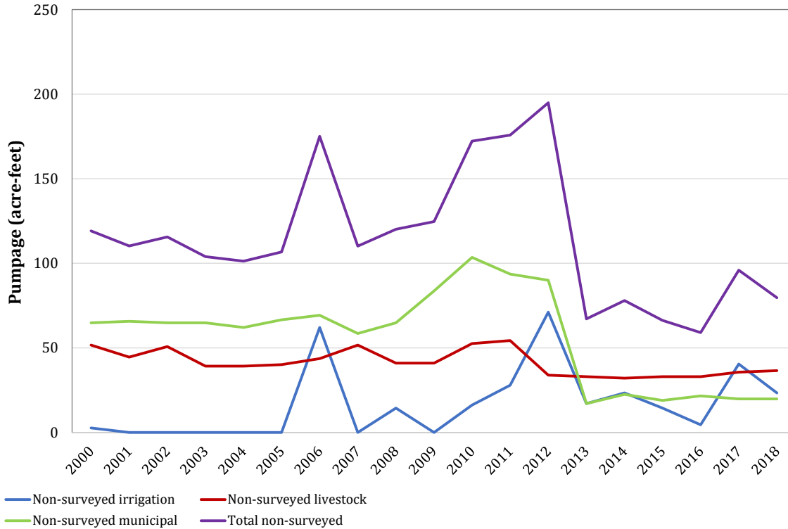
Figure 4-103. Estimated non-surveyed pumpage for the Cross Timbers Aquifer from 2000 to 2018 in Stephens County.
