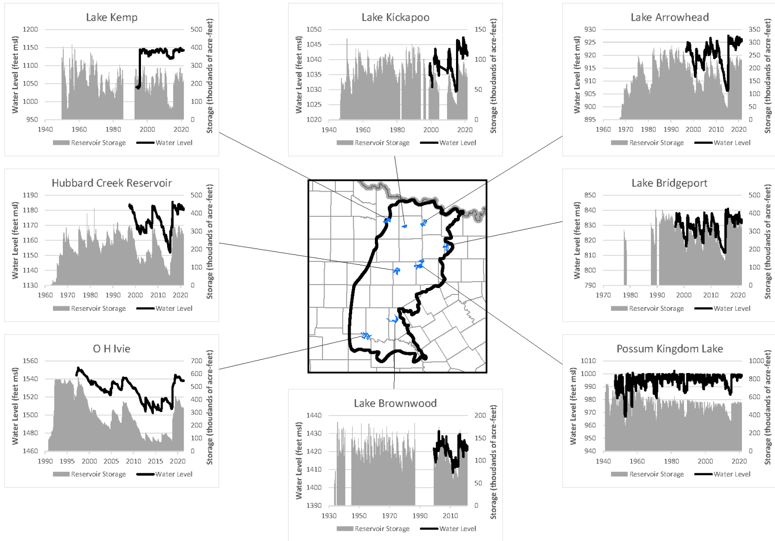
Figure 4-57. Change in volume and stage for selected reservoirs in the region.
