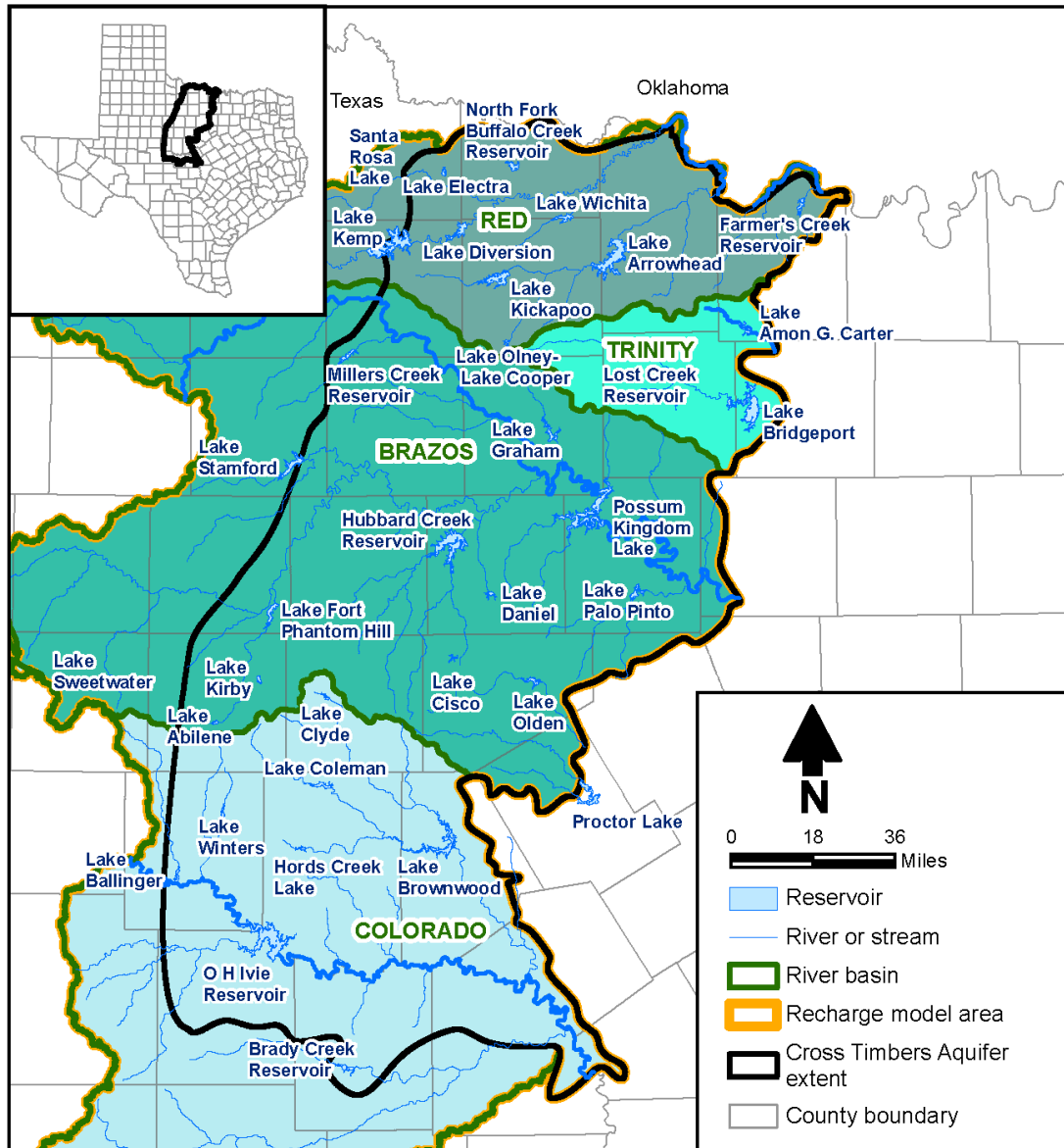
Figure 2-4. Major river basins and surface water features. Major river basin were downloaded from TWDB. Streams were downloaded from the United States Geological Survey National Hydrography Dataset.
