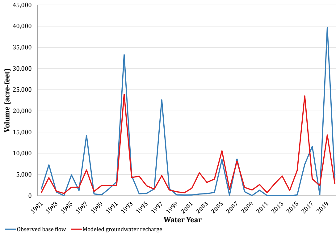
Figure 4-47. Comparison of recharge simulation results to observed base flow for gauge 08086212 (Middle Brazos-Millers).
