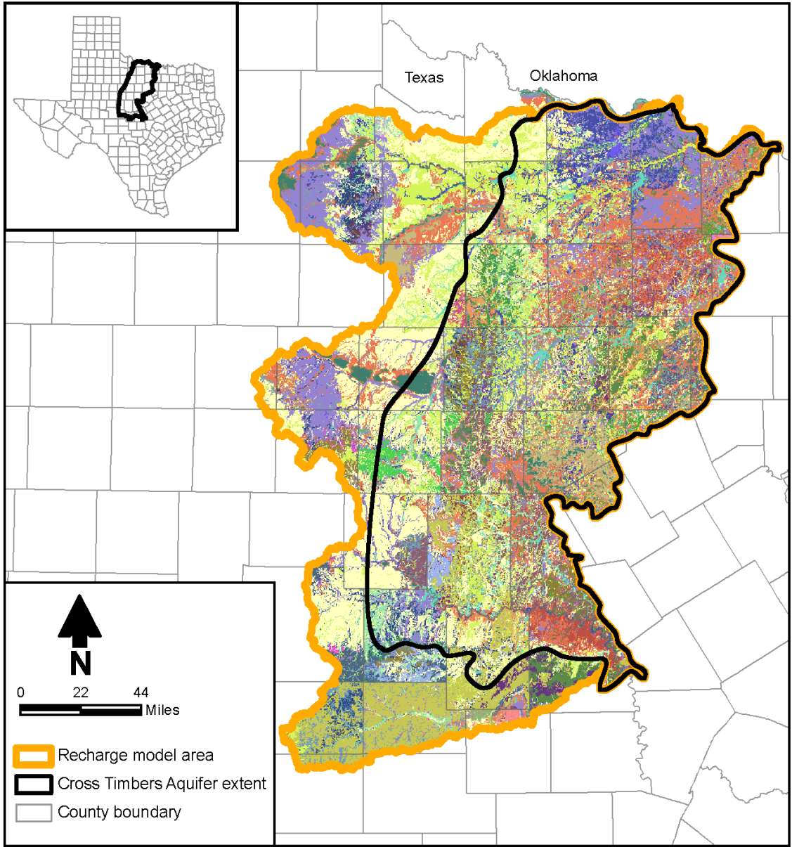
Figure 2-13a. Distribution of soil texture across the study area (soil texture legend provided as Figure 2-13b).
