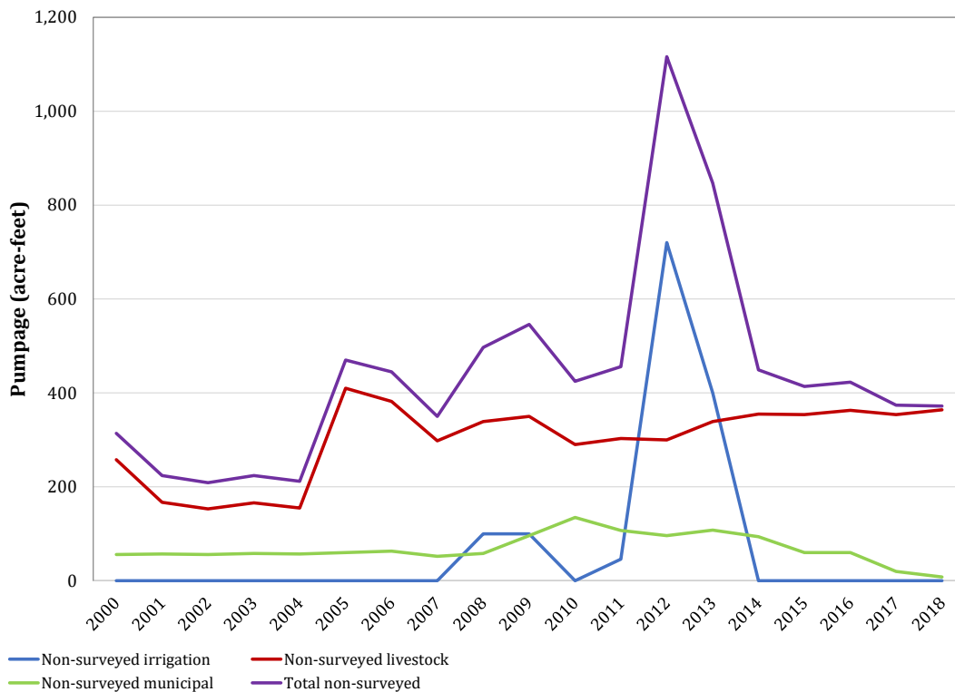
Figure 4-79. Estimated non-surveyed pumpage for the Cross Timbers Aquifer from 2000 to 2018 in Archer County.
