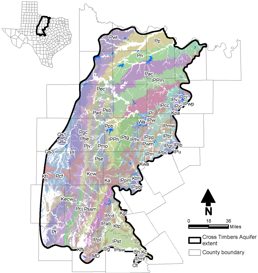
Figure A-1a. Geology used for Distributed Parameters Watershed Model.
