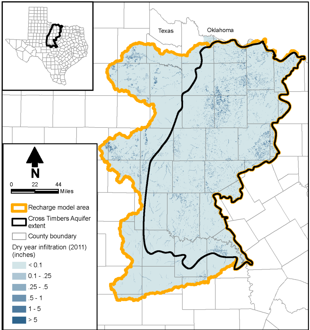
Figure 4-53. Dry year (2011) simulated annual recharge.
