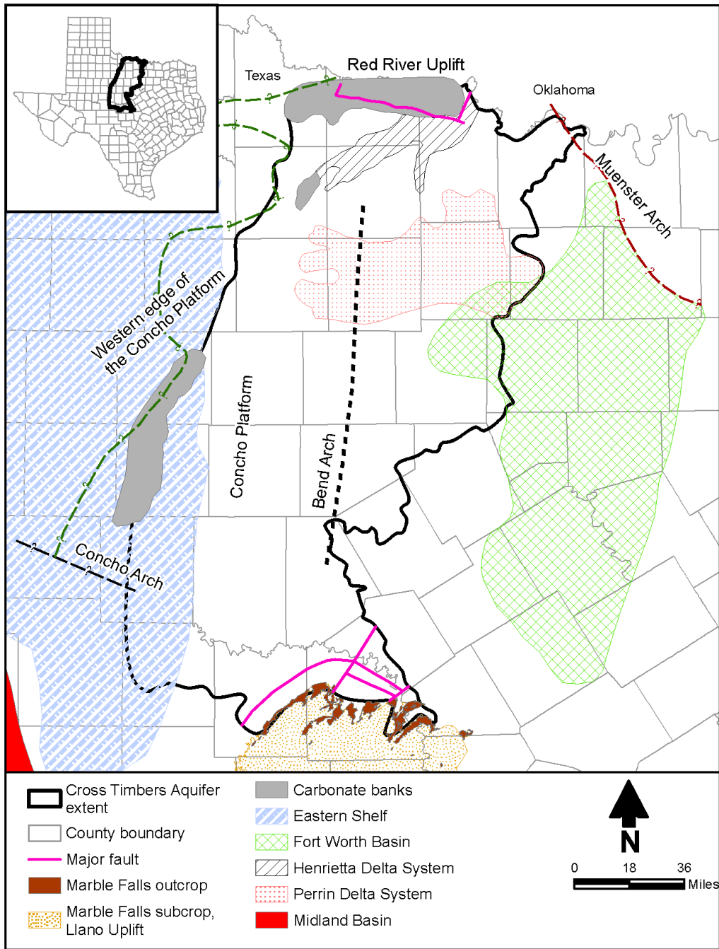
Figure 2-19. Geologic structure features within and adjacent to the study area.
