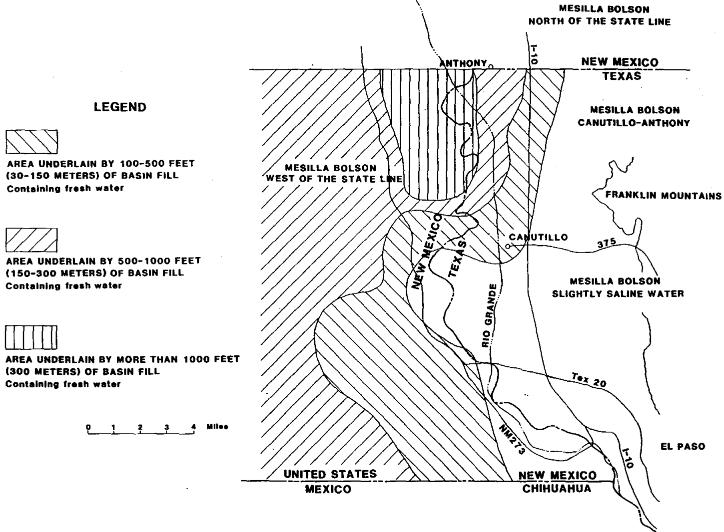
FIGURE No. 6 Quality of Potential Available Groundwater for the Mesilla Bolson
