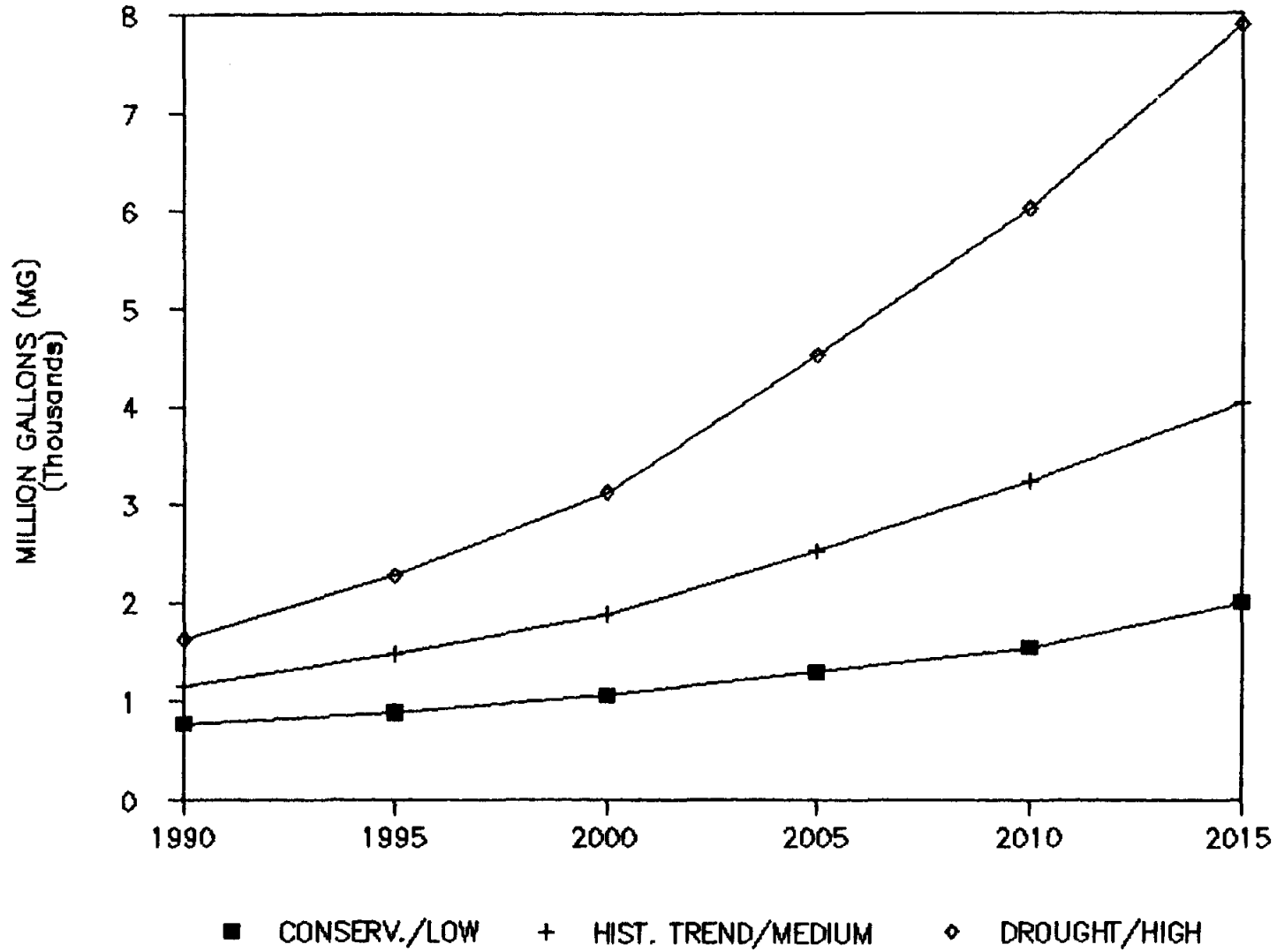
FIGURE 2.5-1 ALTERNATIVE ANNUAL TOTAL WATER DEMAND
