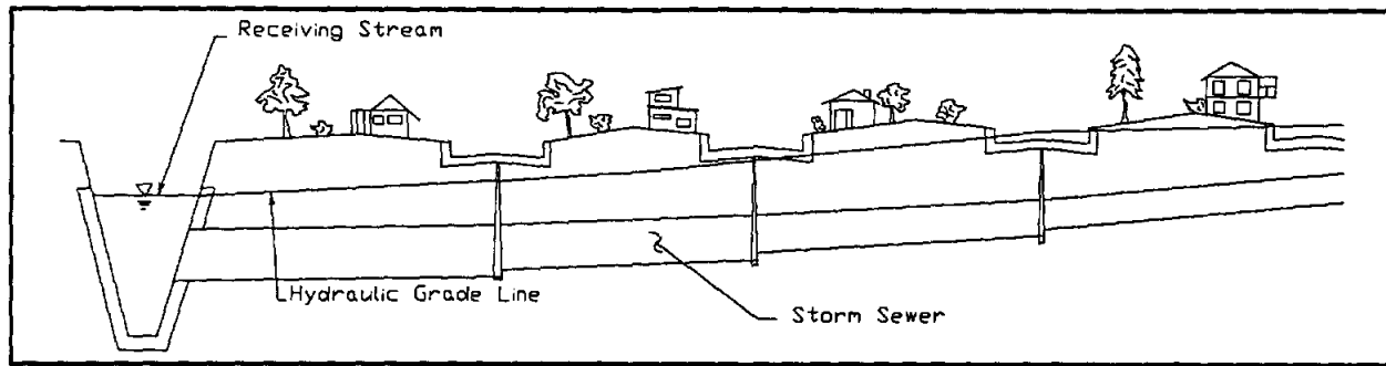
FIGURE 5.2 Effect of Medium Starting Elevation on Storm Sewers
