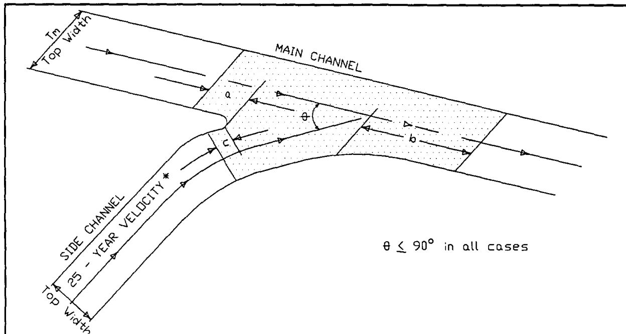
FIGURE 6.1 Typical Channel Confluence
