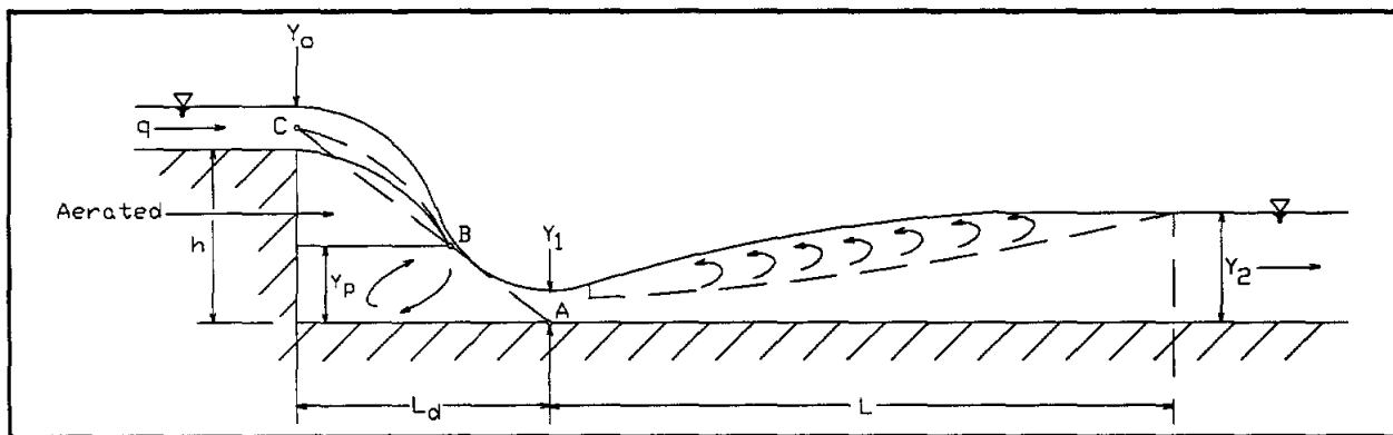
FIGURE 6.6 Flow Geometry of Straight Drop Spillway
