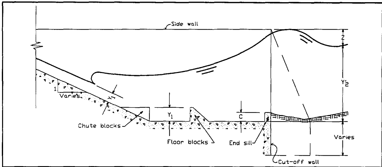
FIGURE 6.11 Center-Line Section of Rectangular SAF-Type Stilling Basin
