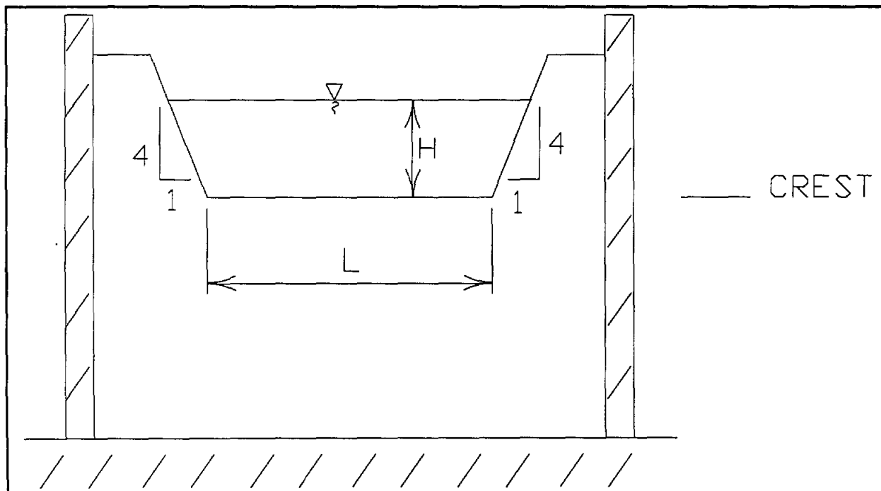
FIGURE 7.7 Sharp-Crested Rectangular Weir
