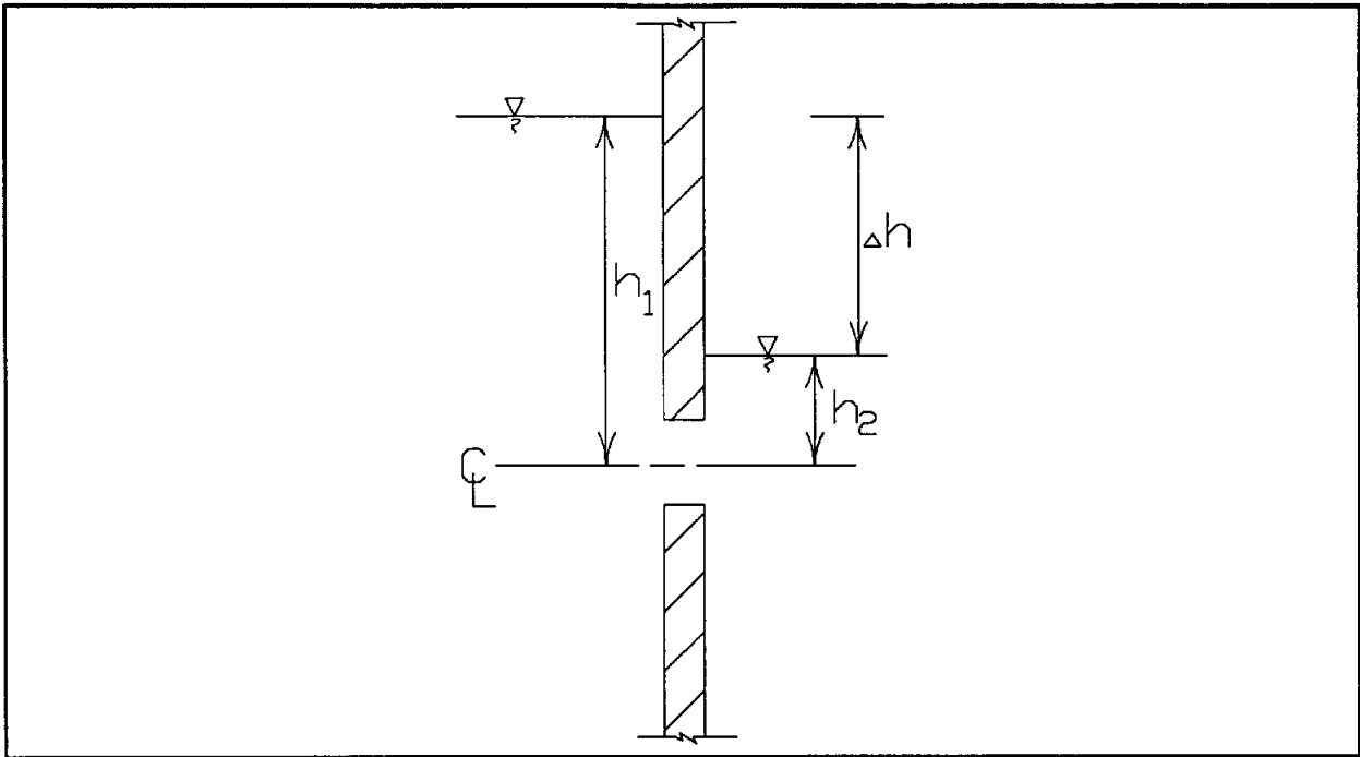
FIGURE 7.14 Submerged Orifice
