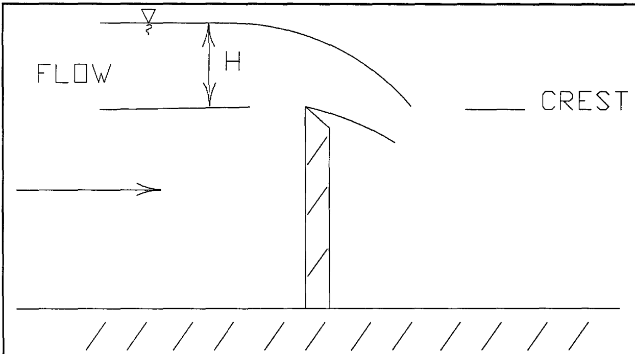
FIGURE 7.8 Section Through Sharp-Crested Weir
