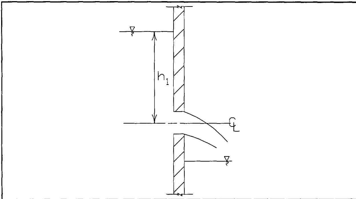
FIGURE 7.13 Unsubmerged Orifice
