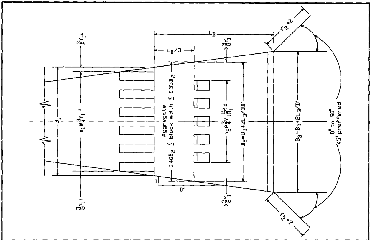
FIGURE 6.13 Plan View of Trapezoidal SAF-Type Stilling Basin
