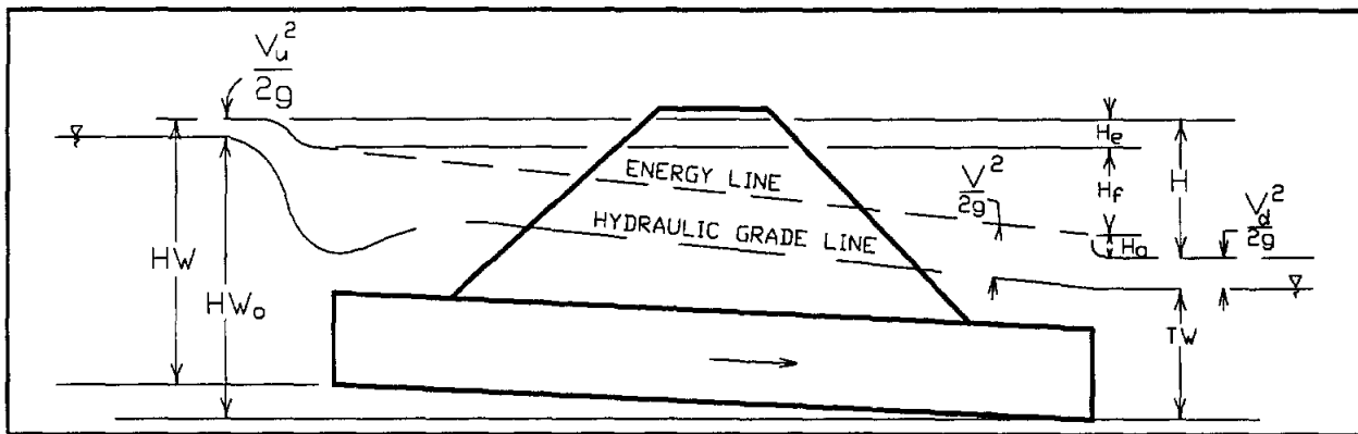
FIGURE 4.4 Hydraulic Elements of Pressure Flow Through Culverts (Source: (FHWA, 1985))
