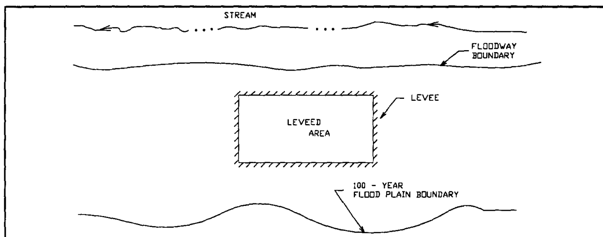
FIGURE 8.1 Typical Layout of Levee Entirely Within Flood Plain
