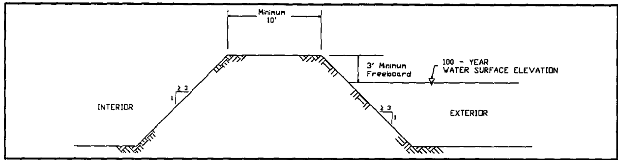
FIGURE 8.3 Typical Levee Cross-Section
