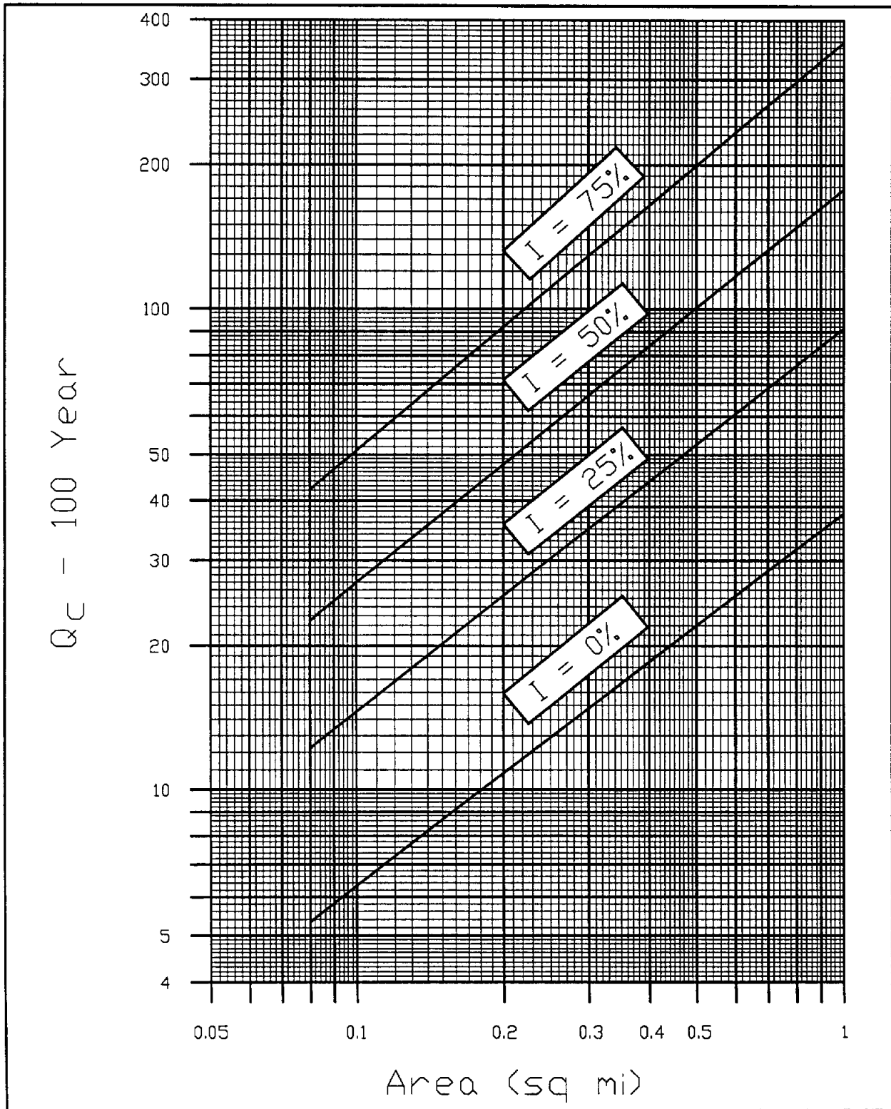
FIGURE 2.4 Montgomery County Runoff Rate Curves for 100-Year Storm
