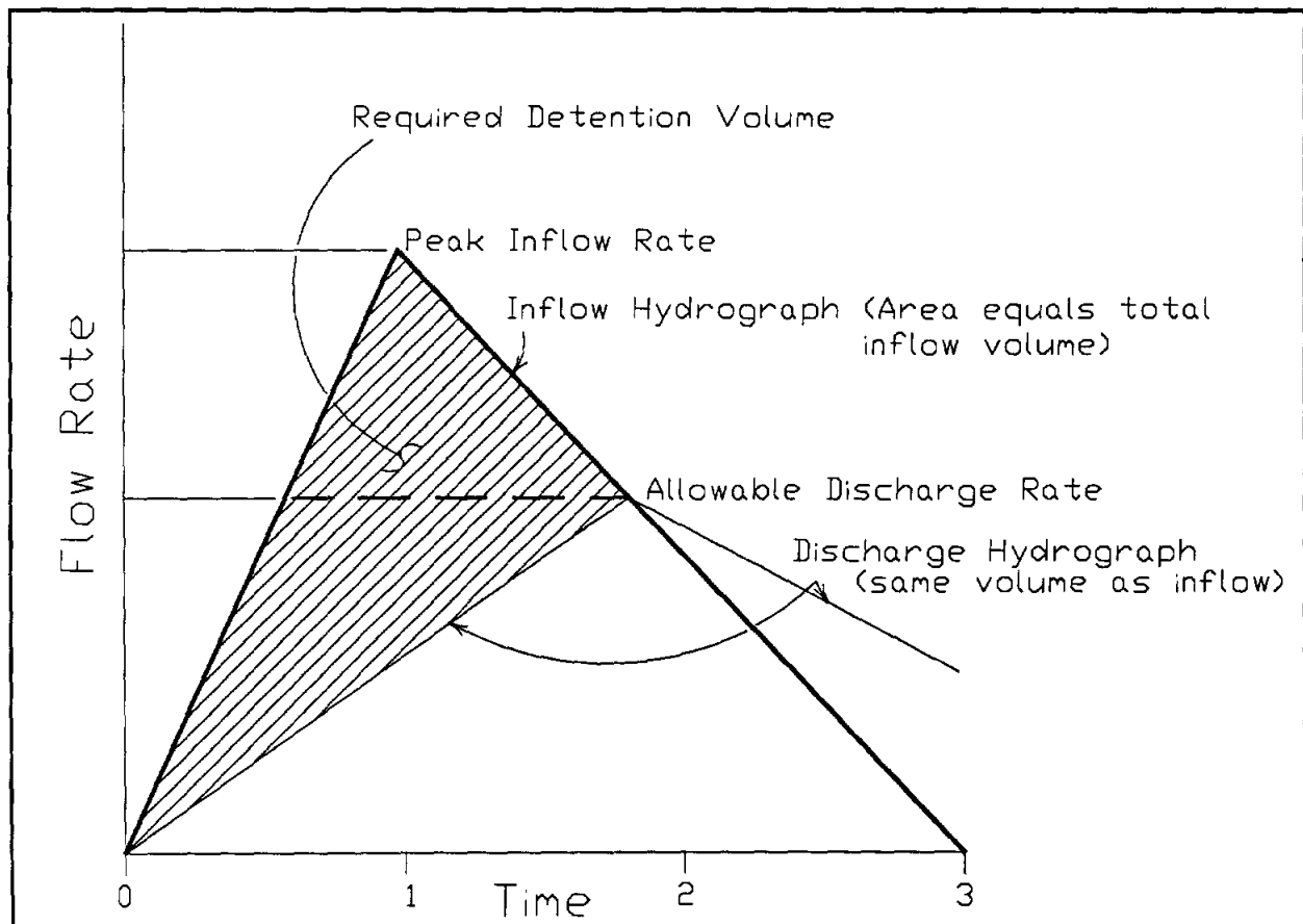
FIGURE 7.5 Required Detention Volume for Less Than 50 Acres
