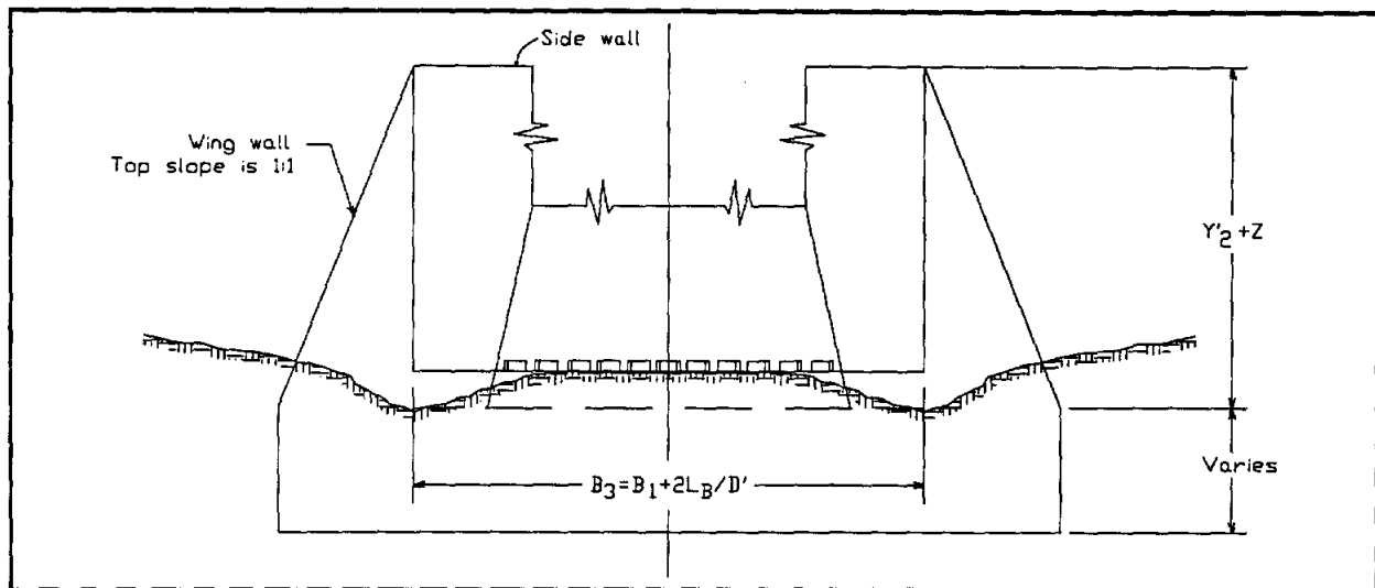
FIGURE 6.15 Downstream Elevation of Trapezoidal SAF-Type Stilling Basin
