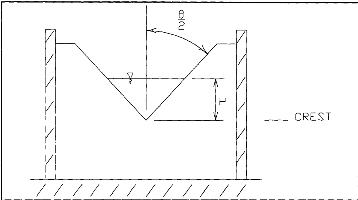
FIGURE 7.10 Sharp-Crested V-Notch Weir
