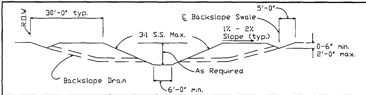
FIGURE 3.1 Typical Section - Grass-Lined Trapezoidal Channel
