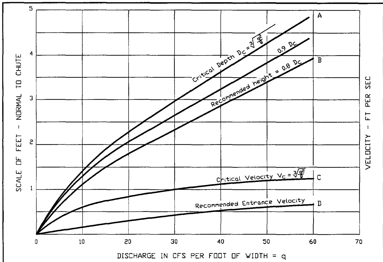
FIGURE 6.9 Recommended Baffle Pier Heights and Allowable Velocities (Source: (USBUREC, 1961))
