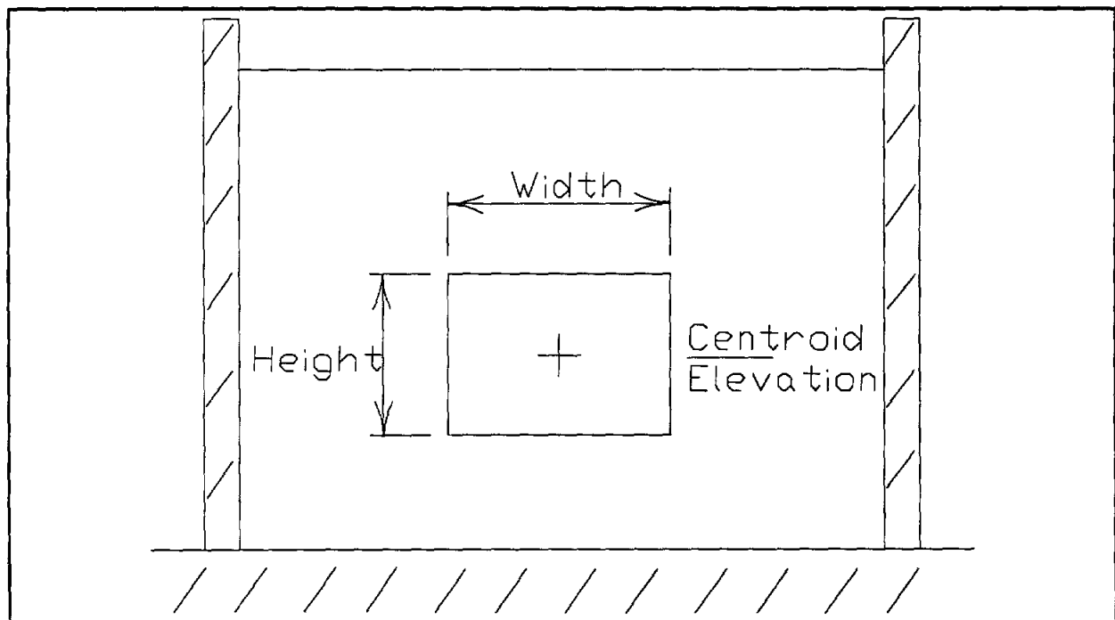
FIGURE 7.12 Rectangular Orifice
