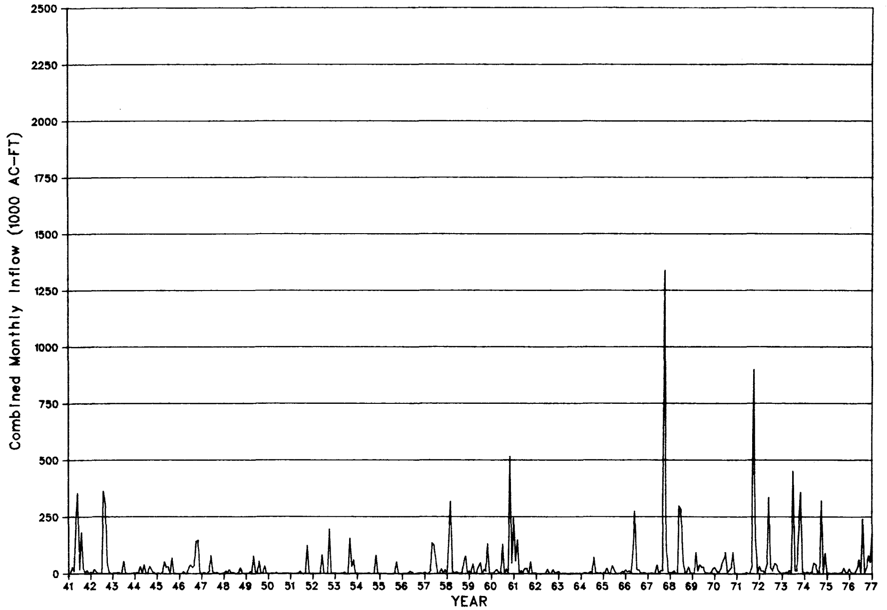
Figure III-9. Combined Monthly Inflow to the Mission-Aransas Estuary, 1941-1976
