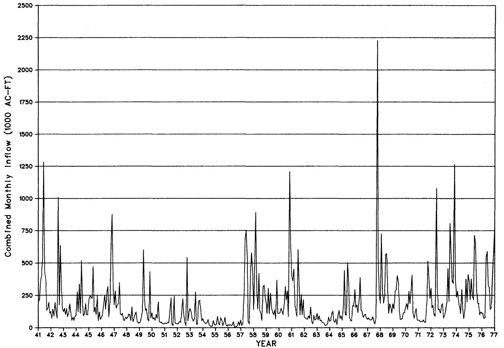
Figure III-7. Combined Monthly Inflow to the Guadalupe Estuary, 1941-1976
