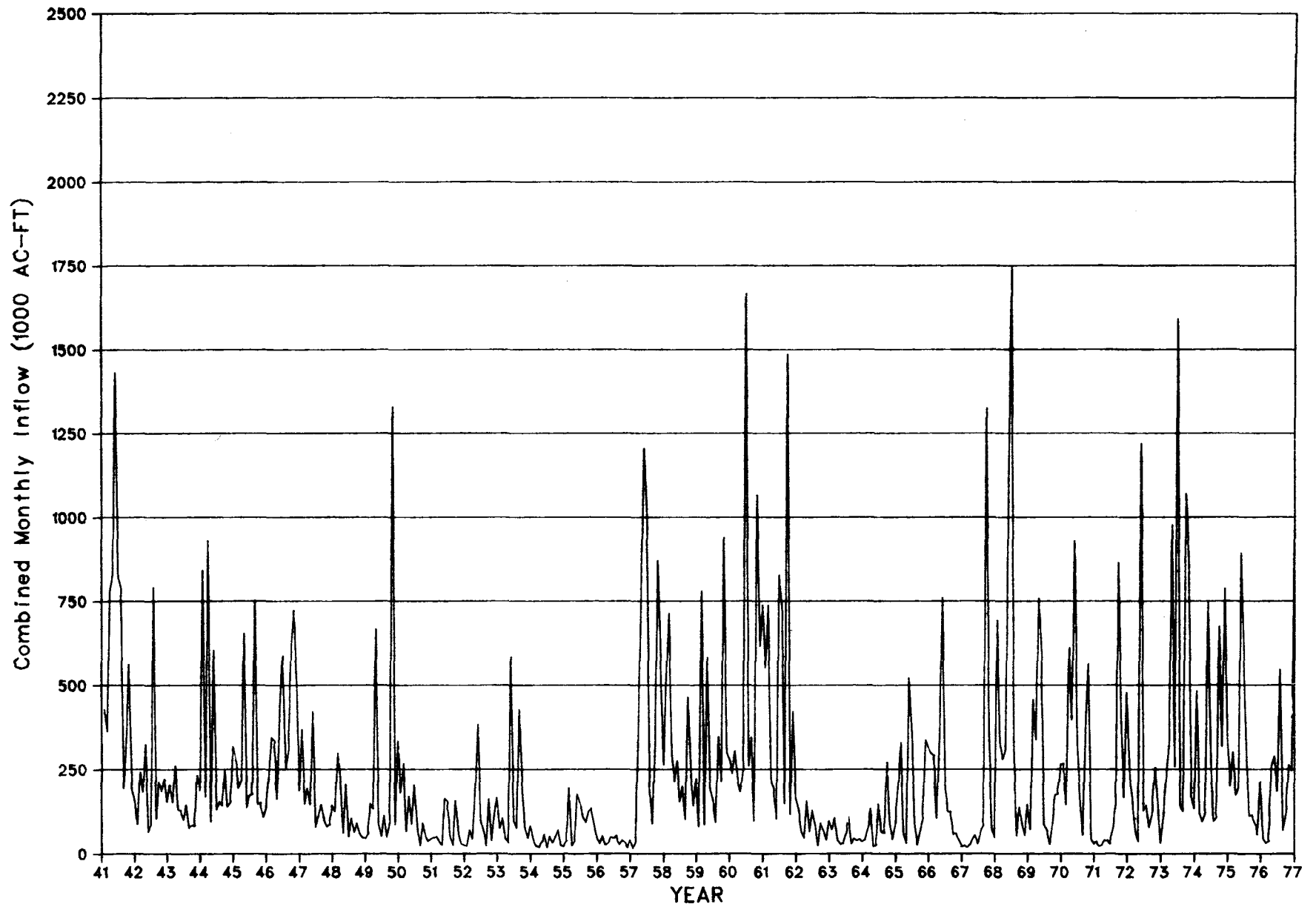
Figure III-5. Combined Monthly Inflow to the Lavaca-Tres Palacios Estuary, 1941-1976
