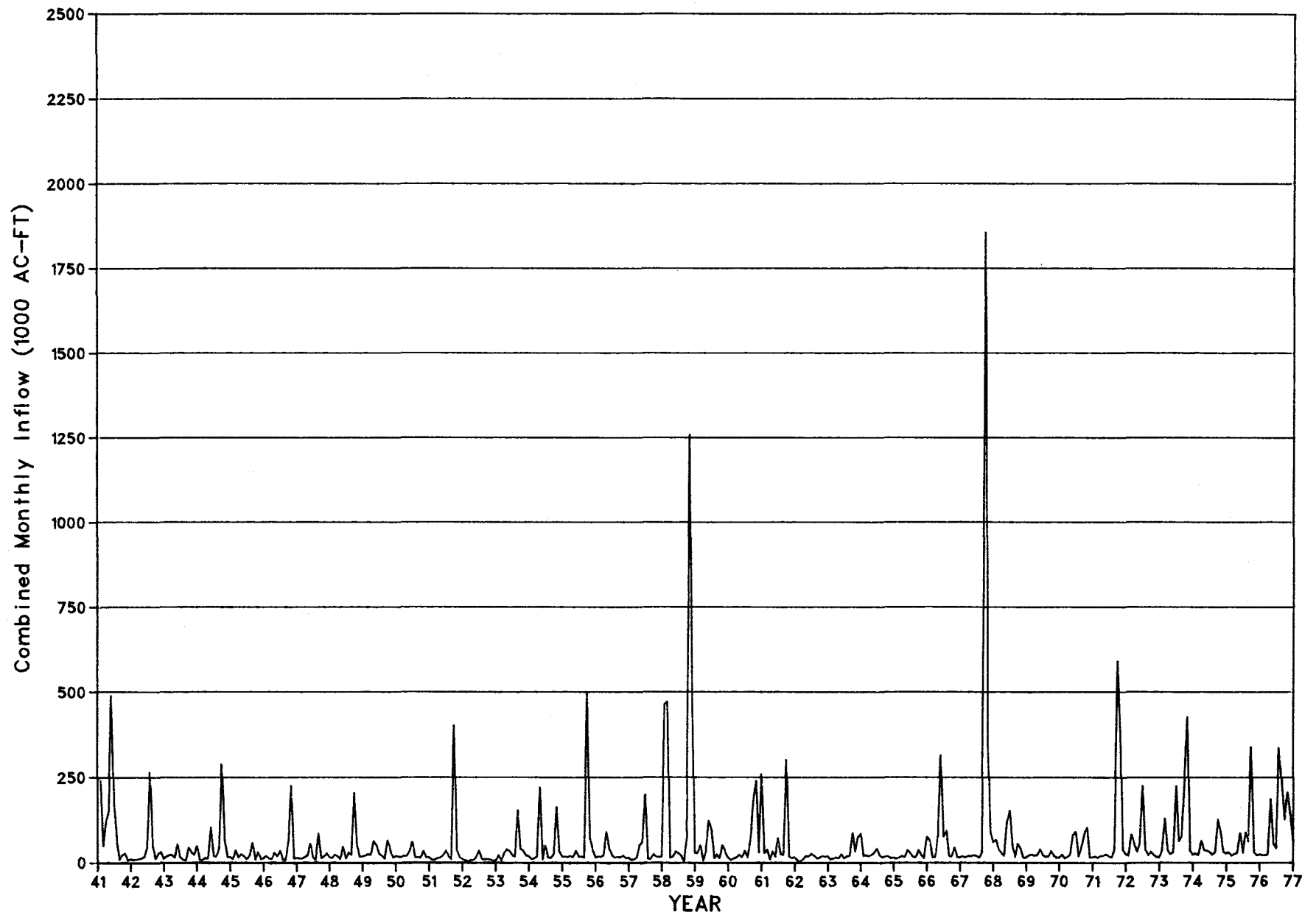
Figure III-13. Combined Monthly Inflow to the Laguna Madre Estuary, 1941-1976
