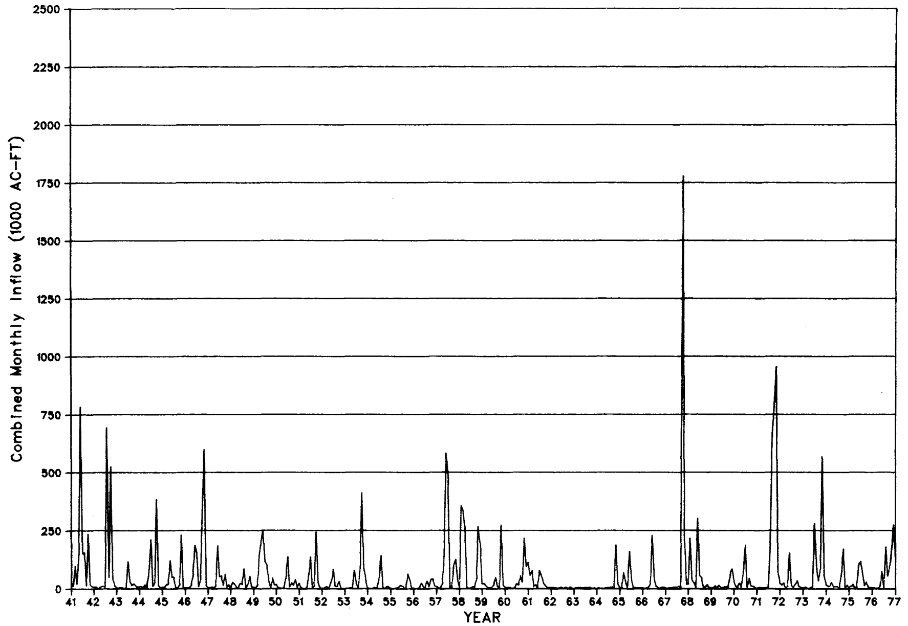
Figure III-11. Combined Monthly Inflow to the Nueces Estuary, 1941-1976
