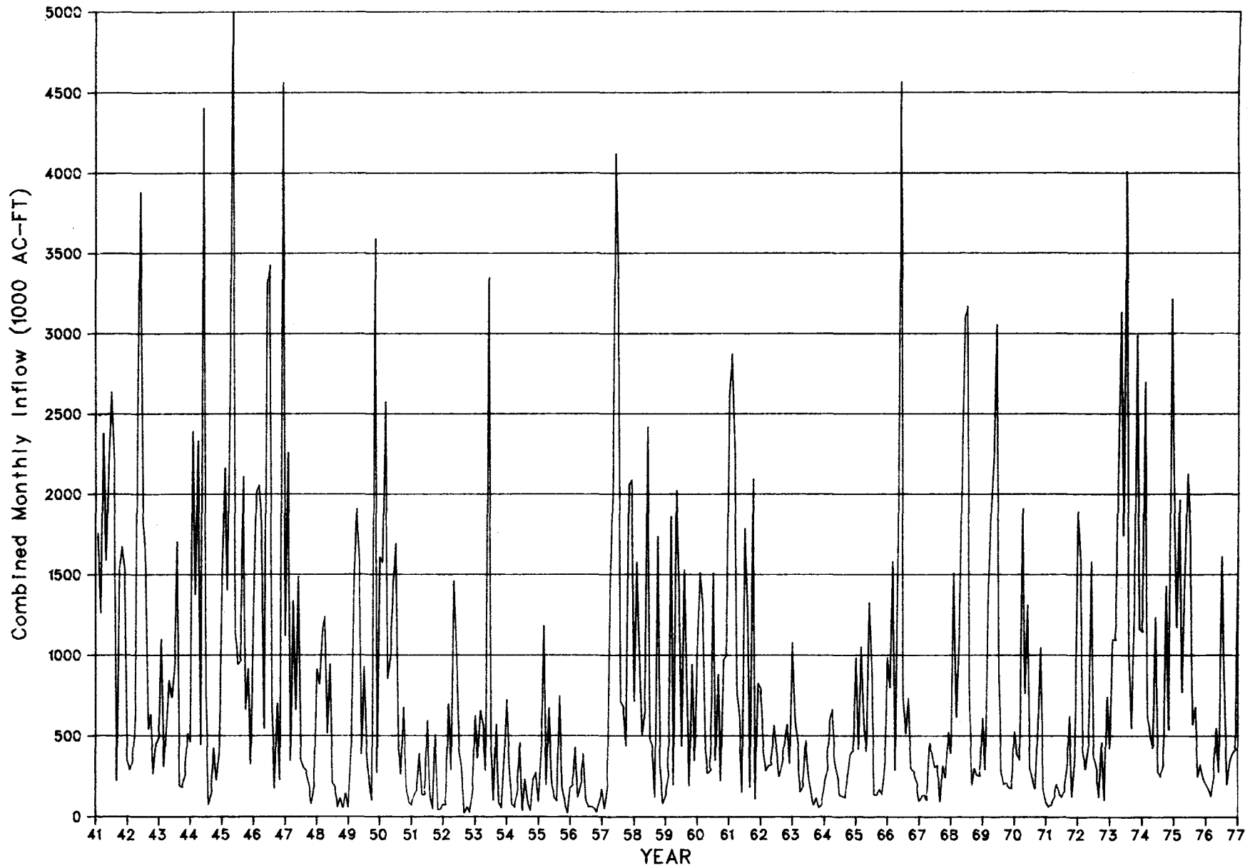
Figure III-3. Combined Monthly Inflow to the Trinity-San Jacinto Estuary, 1941-1976
