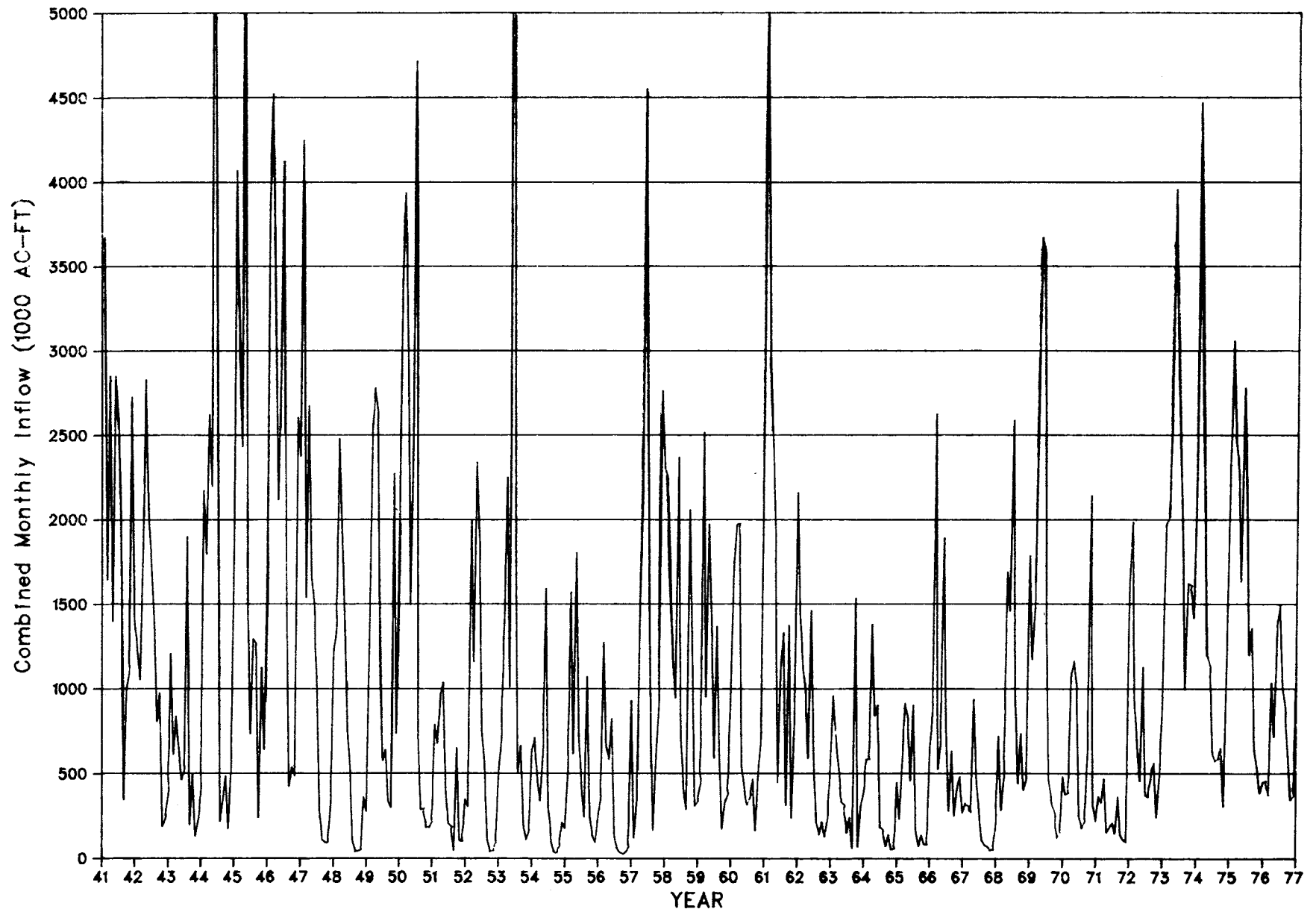
Figure III-1. Combined Monthly Inflow to the Sabine-Neches Estuary, 1941-1976
