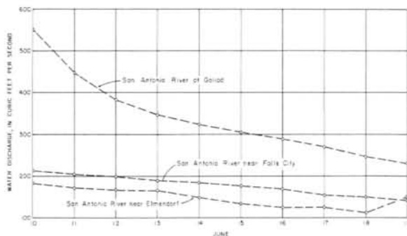
Figure 2.—Hydrographs of Flow Recession for Selected Sites on the San Antonio River
