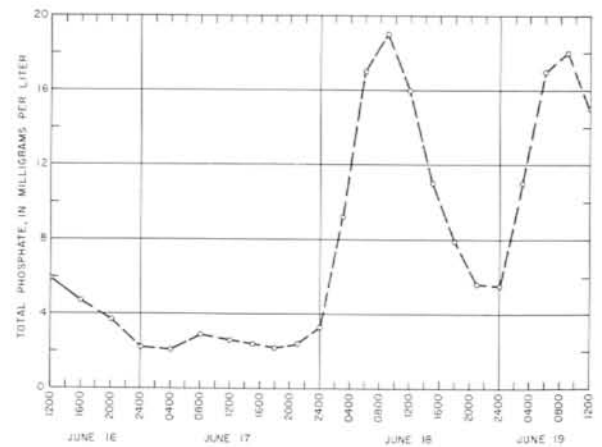
Figure 8.—Diurnal Variations of Total Phosphate, San Antonio River at Farm Road 1518 near Elmendorf
