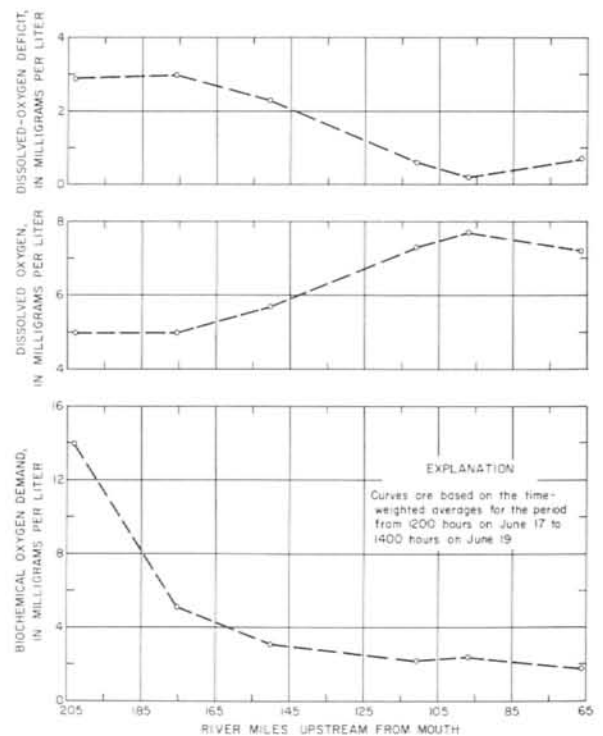
Figure 6.—Time-Weighted Averages of Biochemical Oxygen Demand, Dissolved Oxygen, and Dissolved-Oxygen Deficit for the San Antonio River
