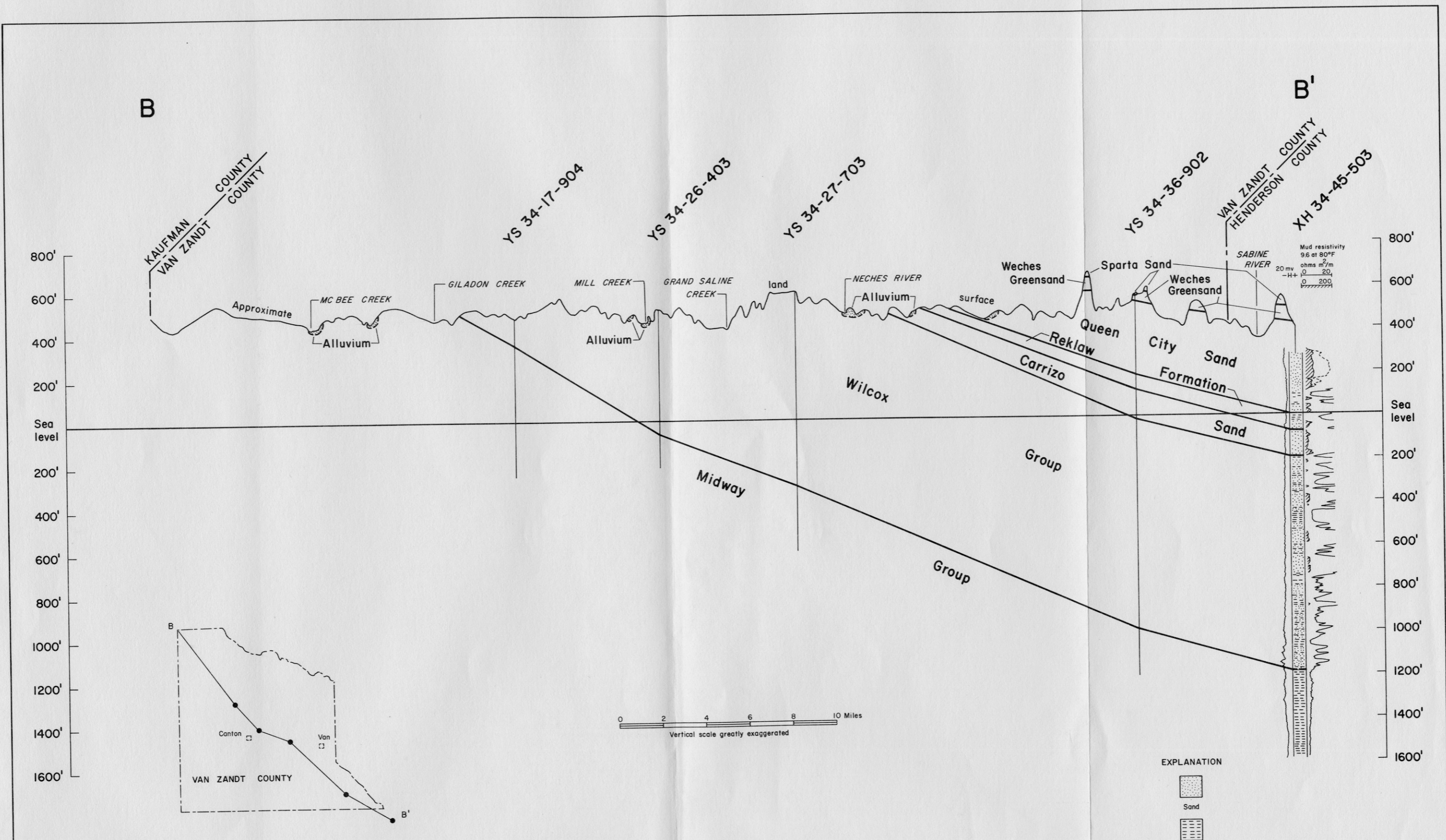
Figure 8 Correlation of Geologic Units Along Line B-B'
