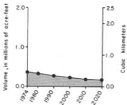
Estimated Volume of Water in Storage, Garza County
