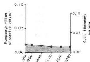
Estimated Pumpage, Garza County
