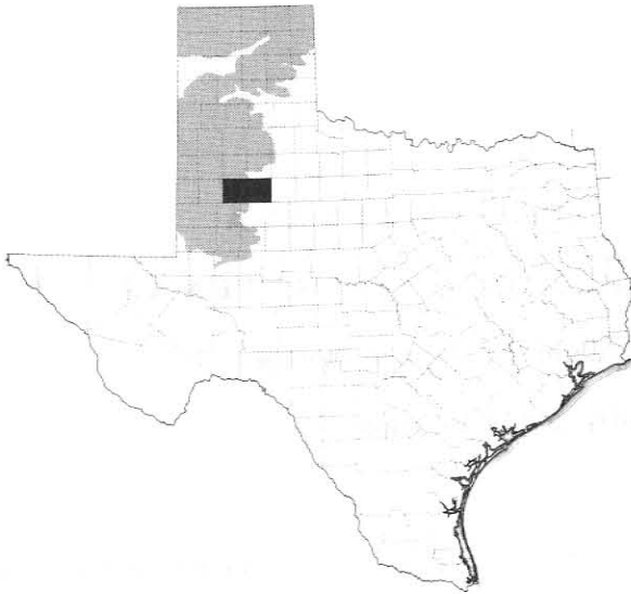
Location of Lynn and Garza Counties, and Extent of the Ogallala Aquifer in Texas
