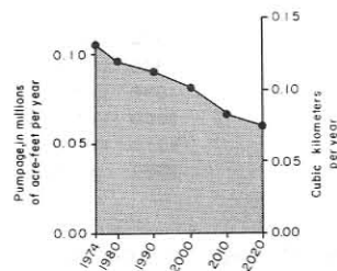
Estimated Pumpage, Lynn County
