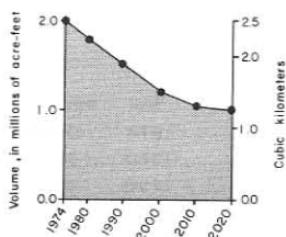
Estimated Volume of Water in Storage, Lynn County
