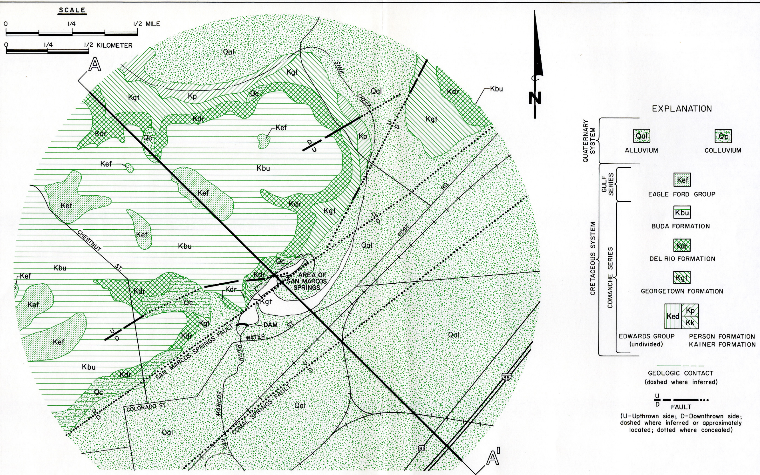
Figure 7 Surface Geology of San Marcos Springs Locality
