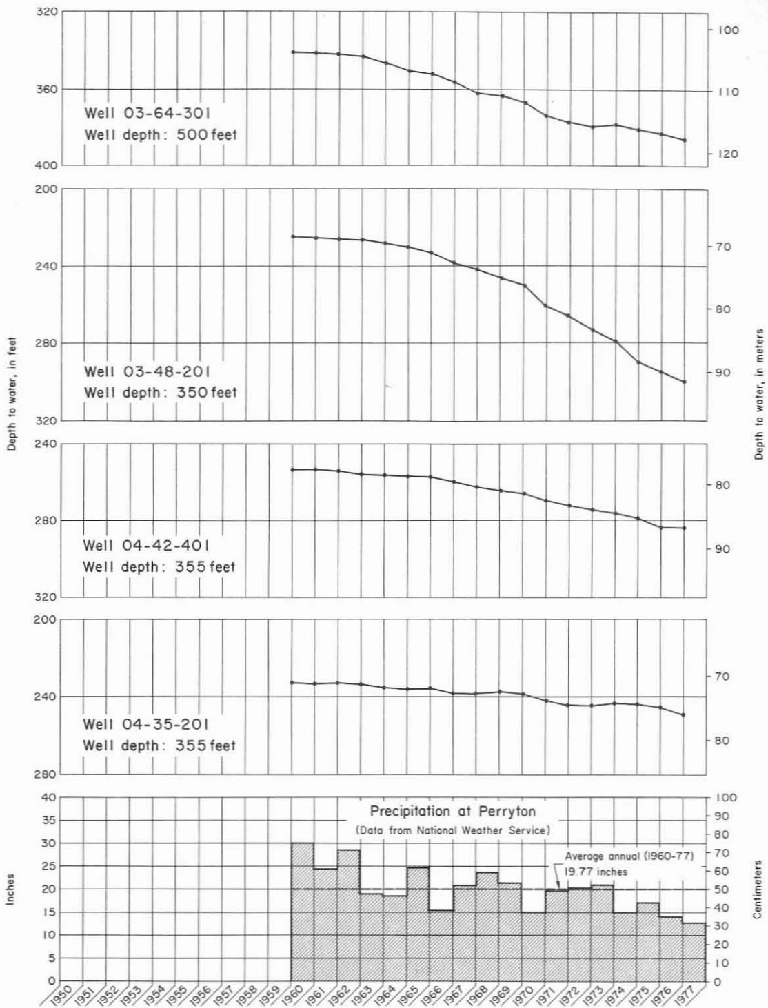
Hydrographs of Selected Wells in Ochiltree County and Precipitation at Perryton
