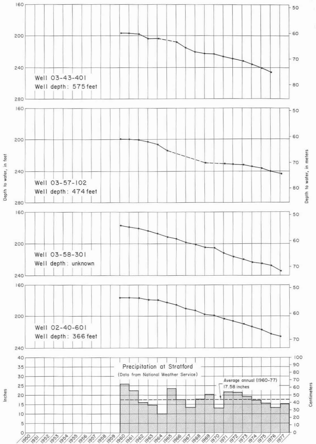
Hydrographs of Selected Wells in Sherman County and Precipitation at Stratford
