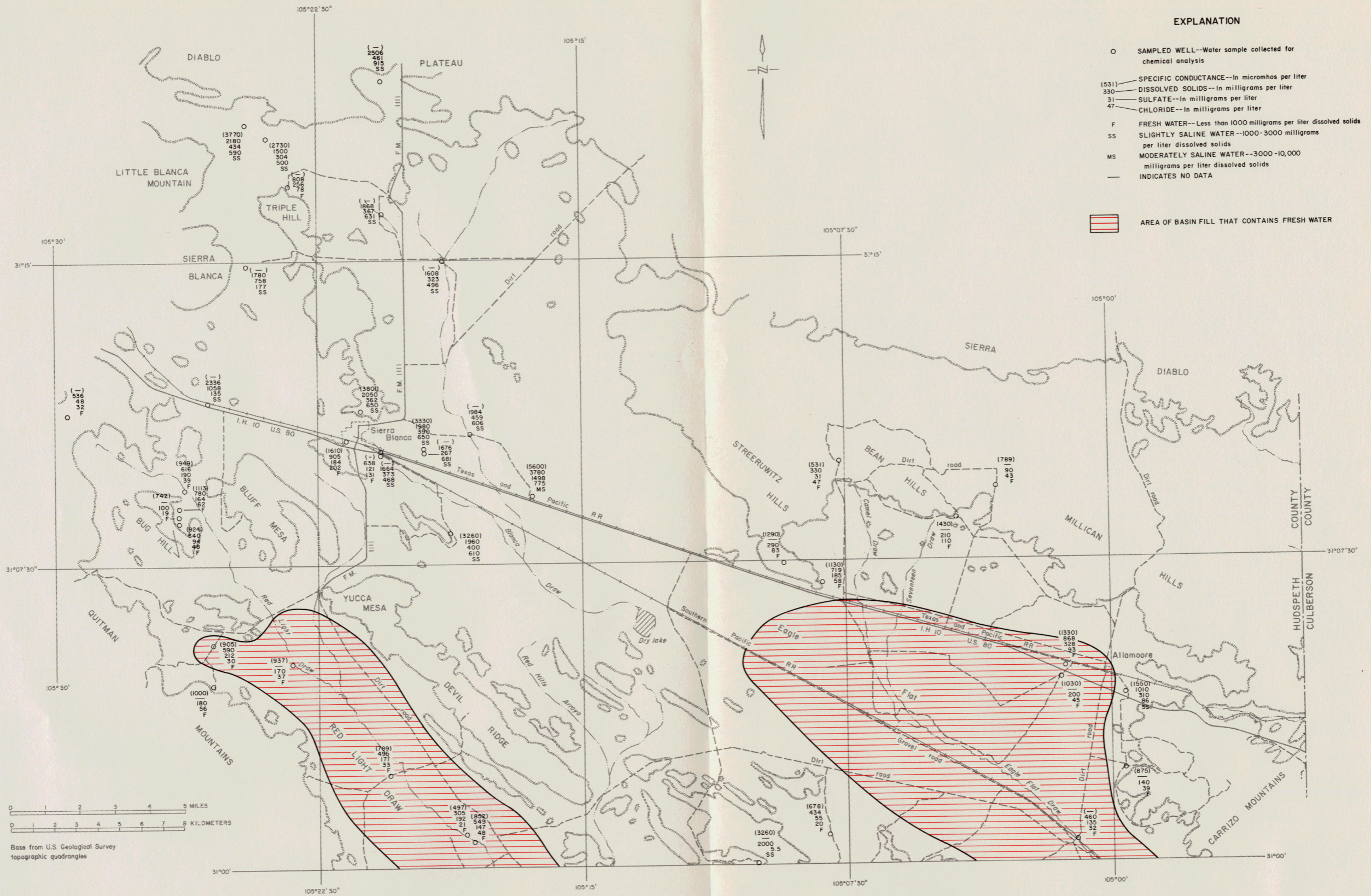
Figure 19 Quality of Ground Water in Eagle Flat, Northern Red Light Draw, and Adjacent Areas
