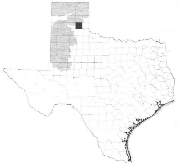
Location of Donley County, and Extent of the Ogallala Aquifer in Texas
