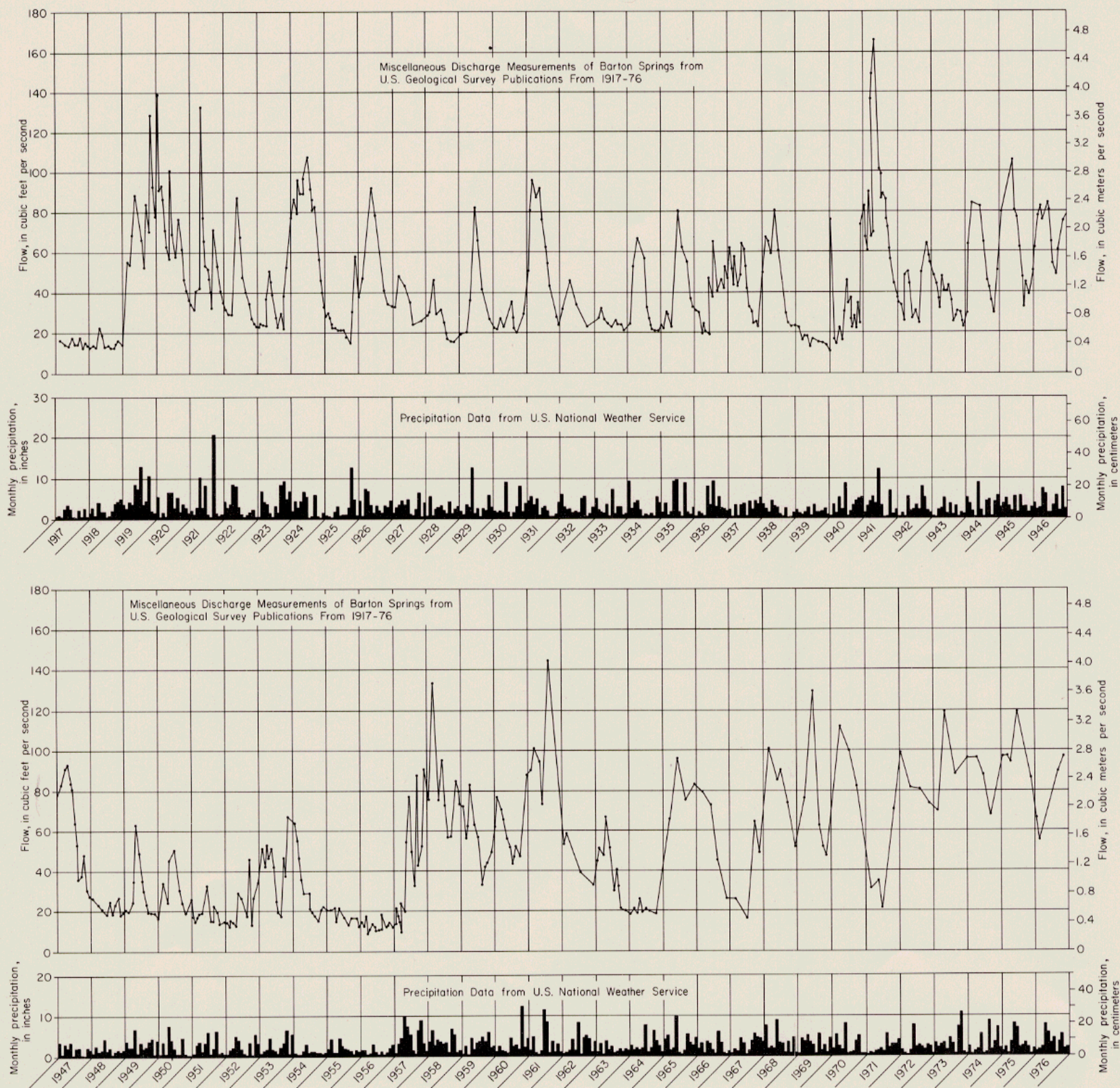
Figure 20 Flow of Barton Springs and Precipitation at Austin, 1917-76
