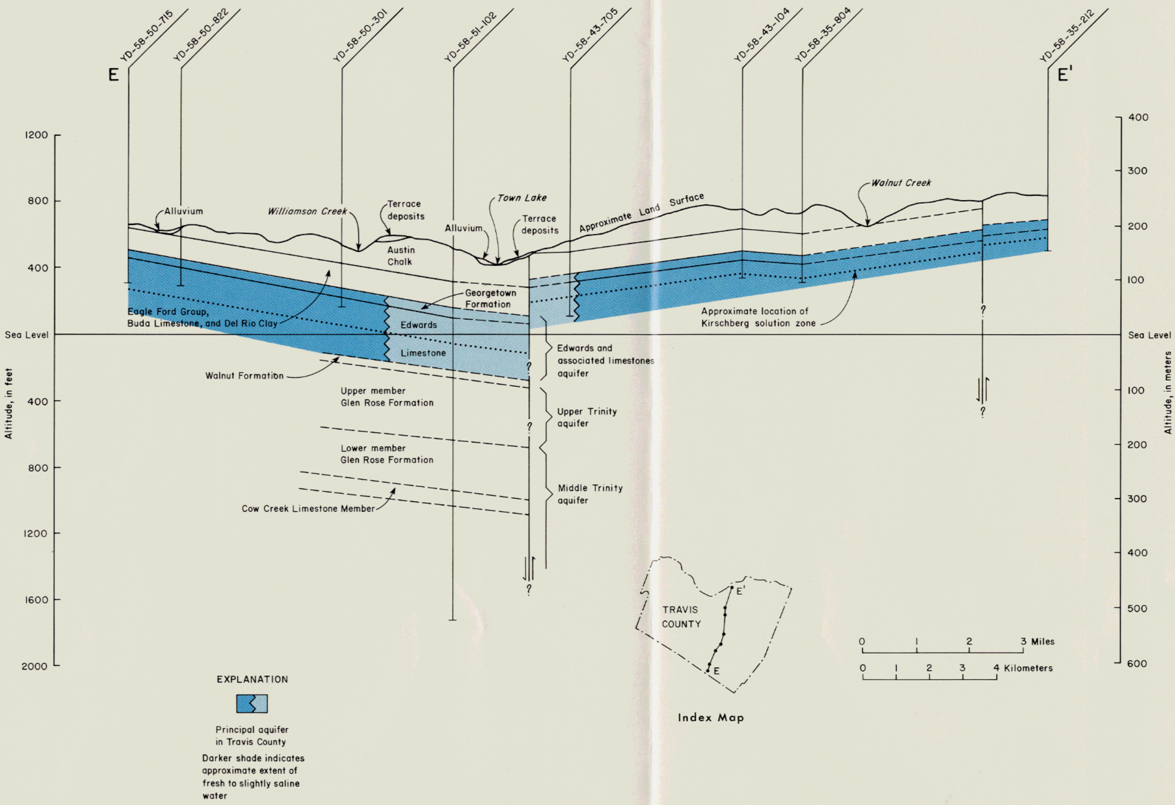
Figure 30 Geologic Section E-E'
