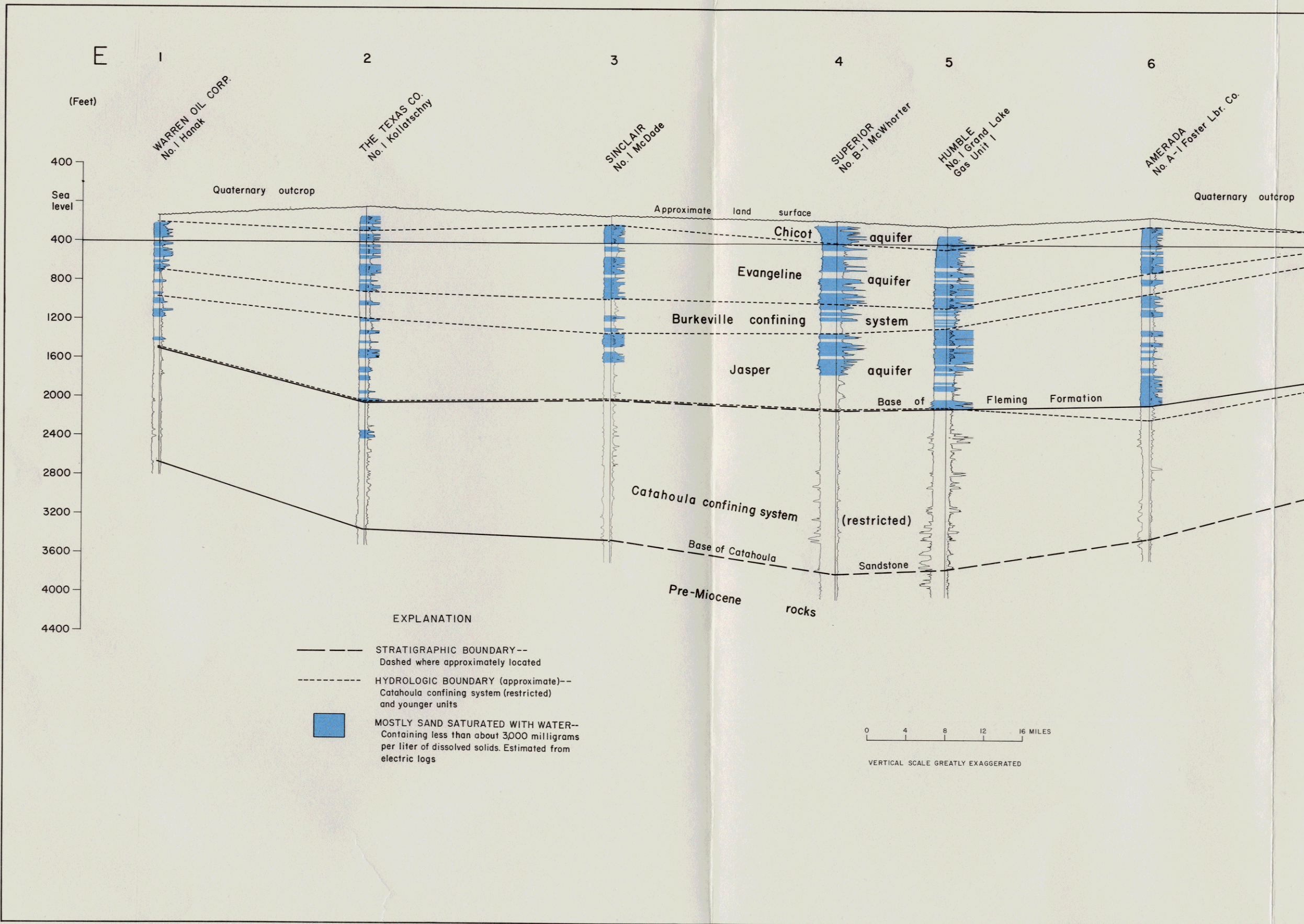
Figure 7.—Stratigraphic and hydrologic section, E-E'.
