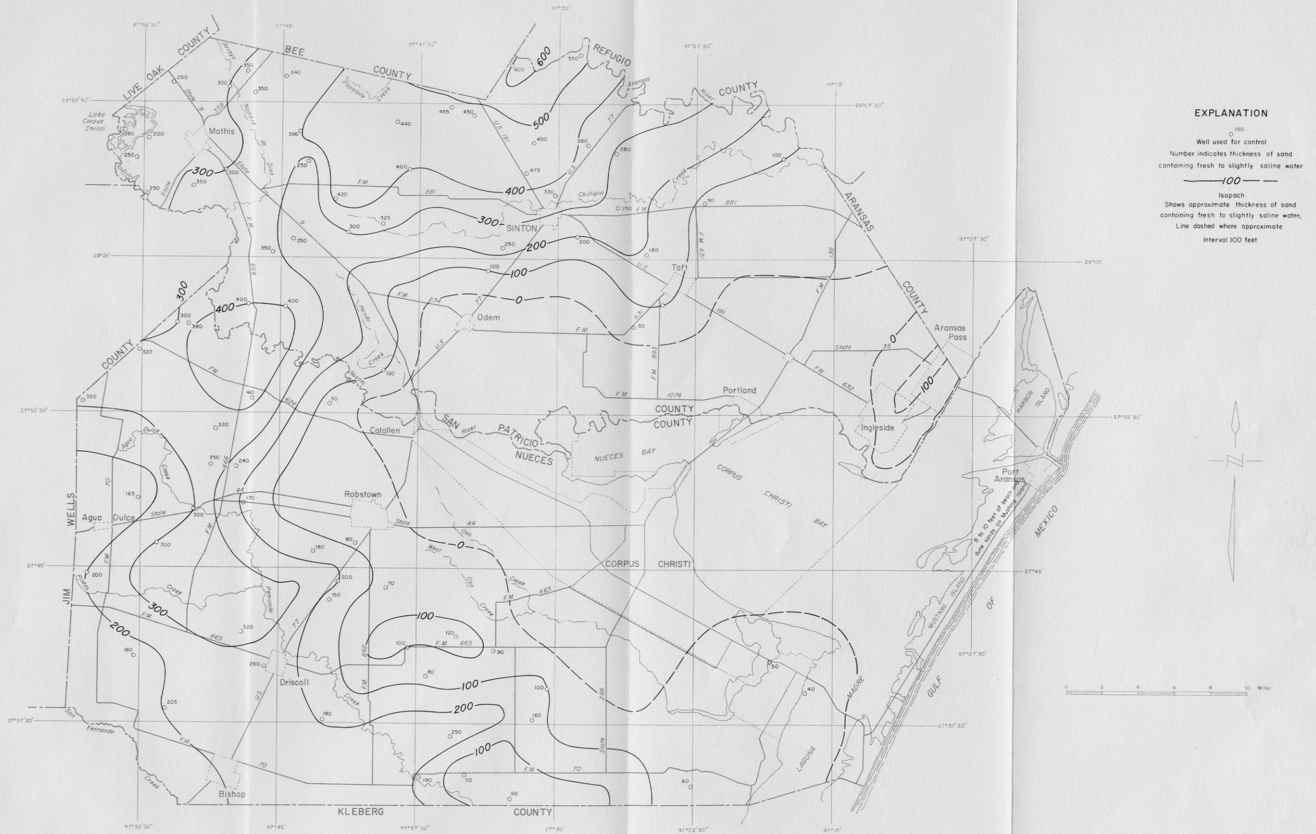
Figure 13 Approximate Thickness of Sand Containing Fresh to Slightly Saline Water in the Gulf Coast Aquifer
