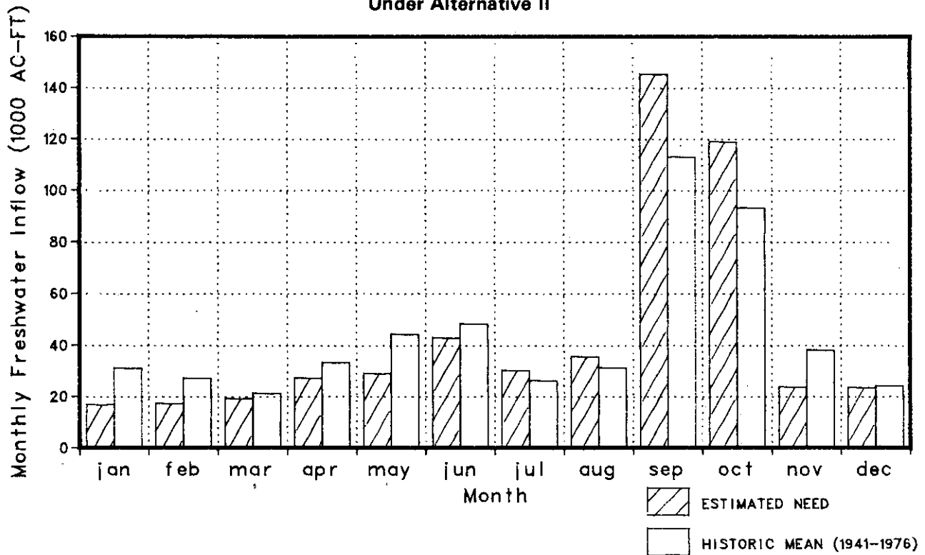
Figure 9-13. Comparison Between Mean Historical Freshwater Inflow and Inflow Needs for Lower Laguna Madre Under Alternative II
