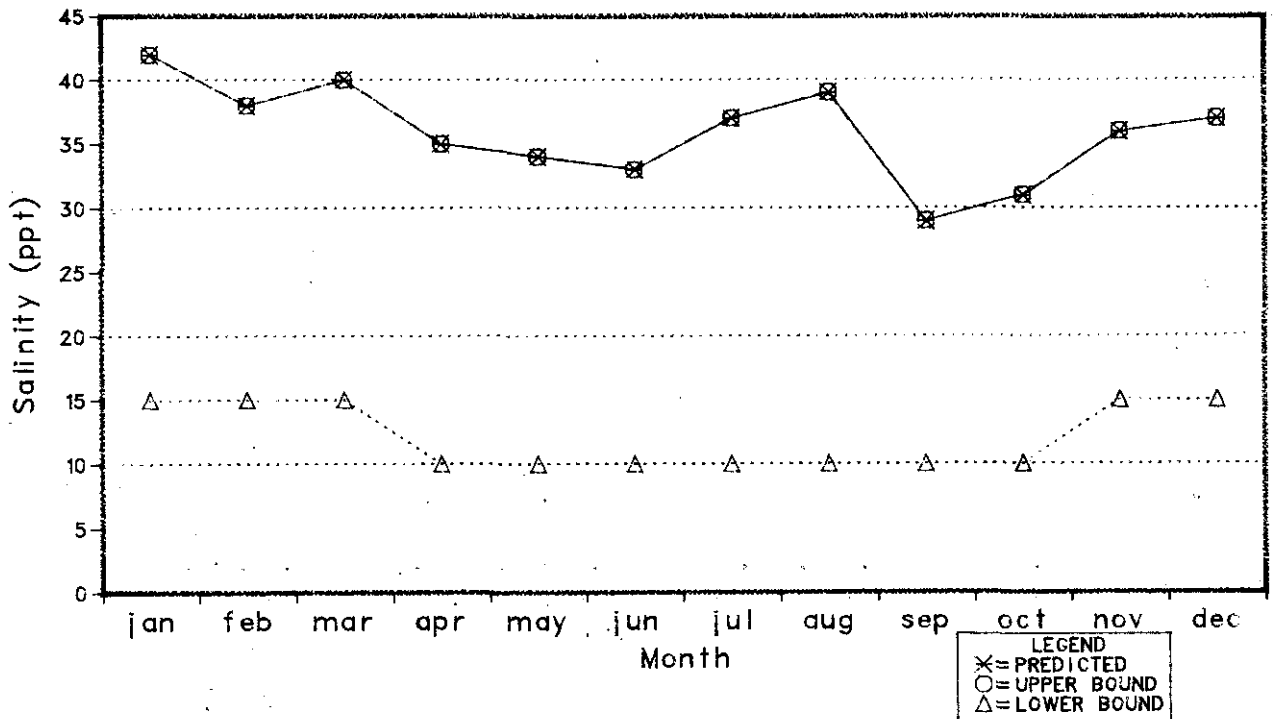
Figure 9-3. Average Monthly Salinities at Intersection of Intracoastal Waterway and Arroyo Colorado Under Alternative I
