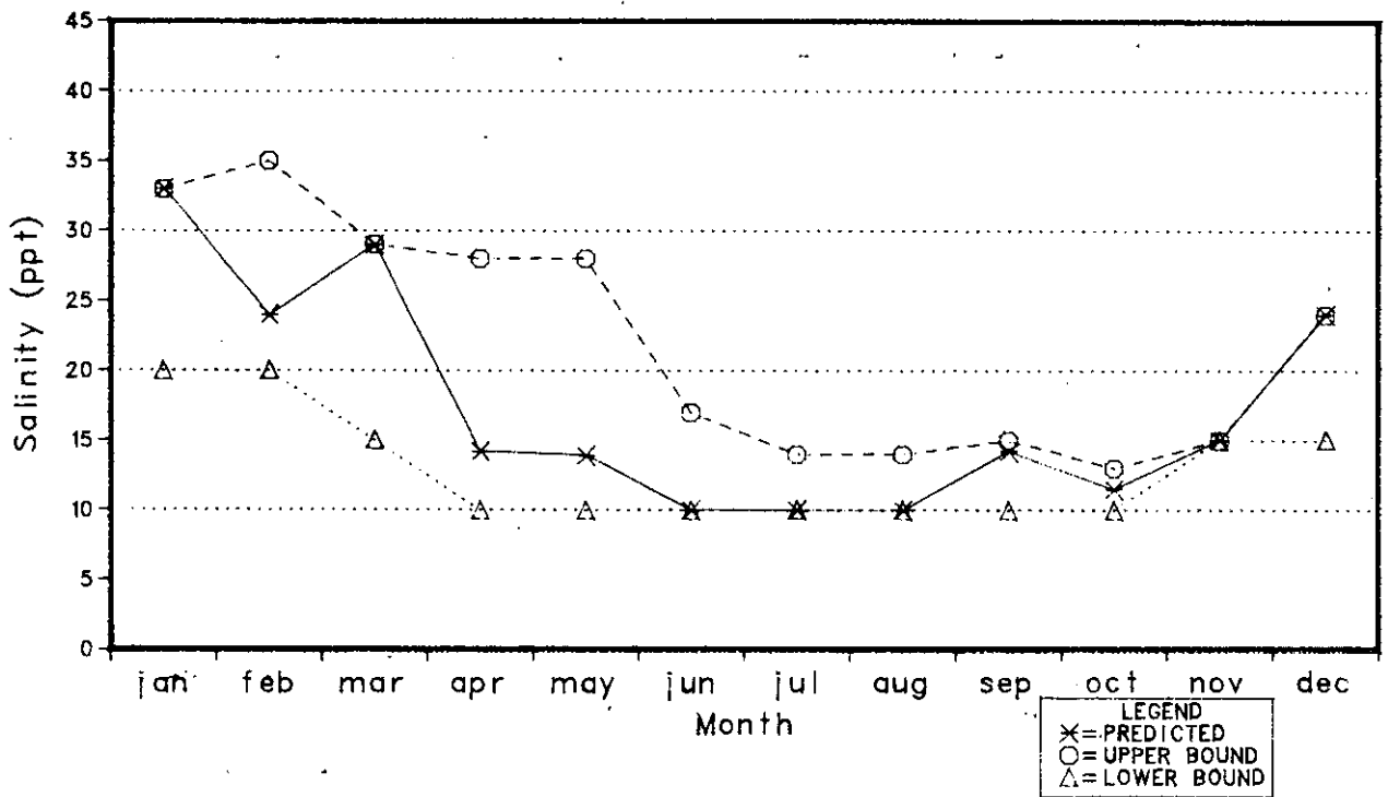
Figure 9-18. Average Monthly Salinity in Upper Baffin Bay Under Alternative III
