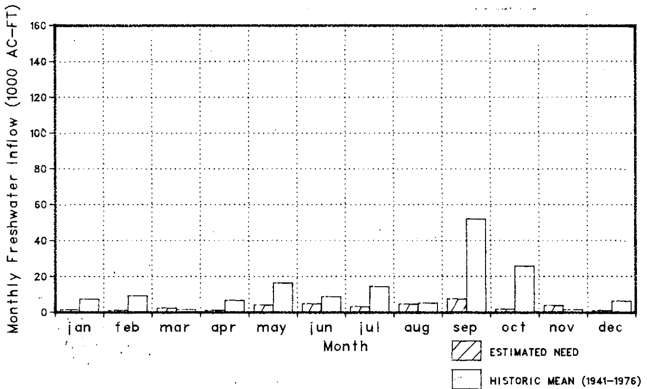
Figure 9-4. Comparison Between Mean Historical Freshwater Inflow and Inflow Needs for Baffin Bay and Upper Laguna Madre Under Alternative I
