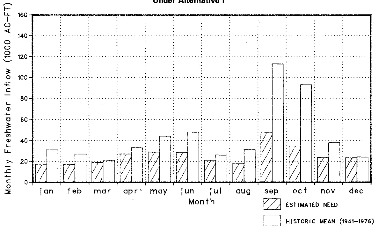
Figure 9-5. Comparison Between Mean Historical Freshwater Inflow and Inflow Needs for Lower Laguna Madre Under Alternative I
