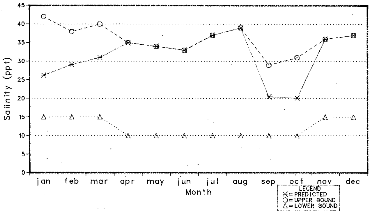
Figure 9-19. Average Monthly Salinities at Intersection of Intracoastal Waterway and Arroyo Colorado Under Alternative III
