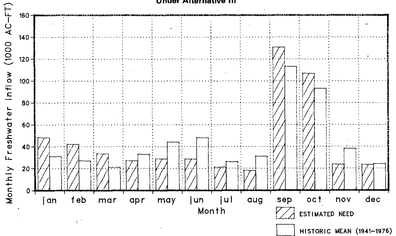
Figure 9-21. Comparison Between Mean Historical Freshwater Inflow and Inflow Needs for Lower Laguna Madre Under Alternative III
