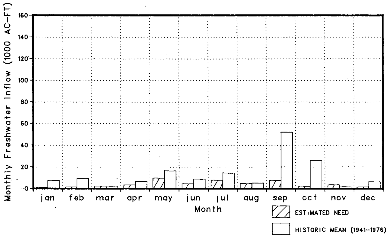
Figure 9-12. Comparison Between Mean Historical Freshwater Inflow and Inflow Needs for Upper Laguna Madre and Baffin Bay Under Alternative II
