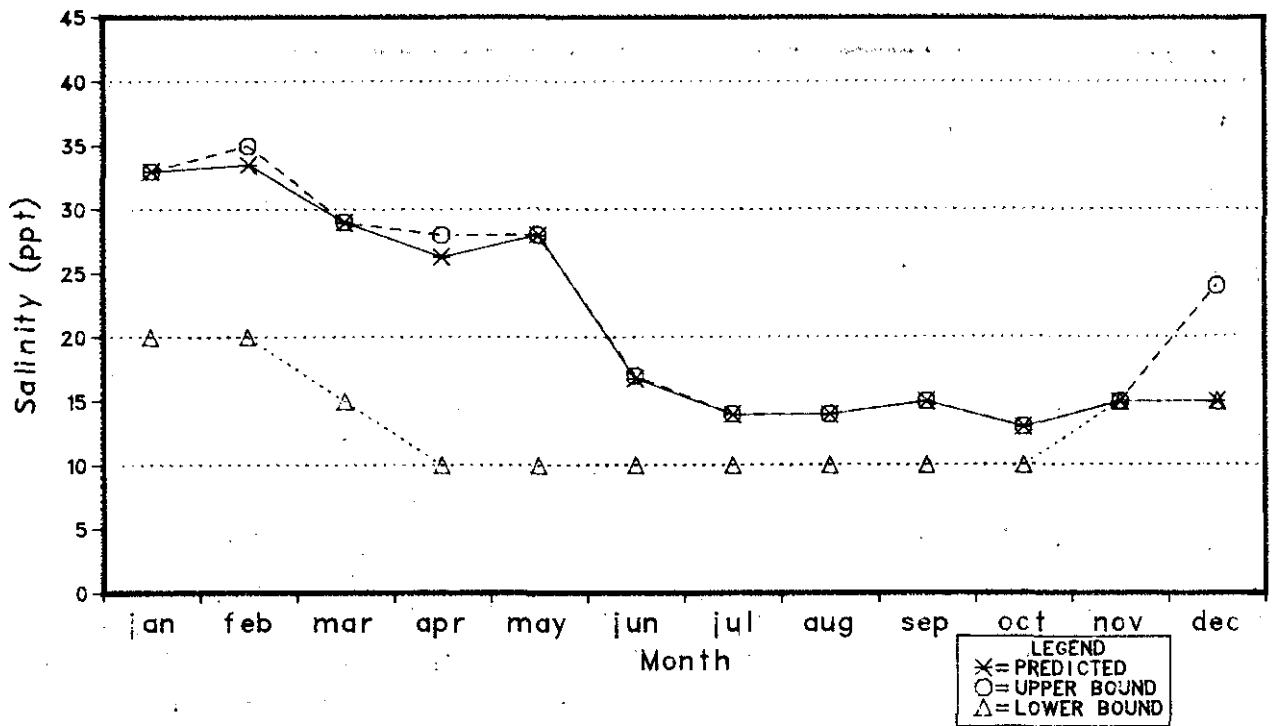
Figure 9-2. Average Monthly Salinities in Upper Baffin Bay Under Alternative I
