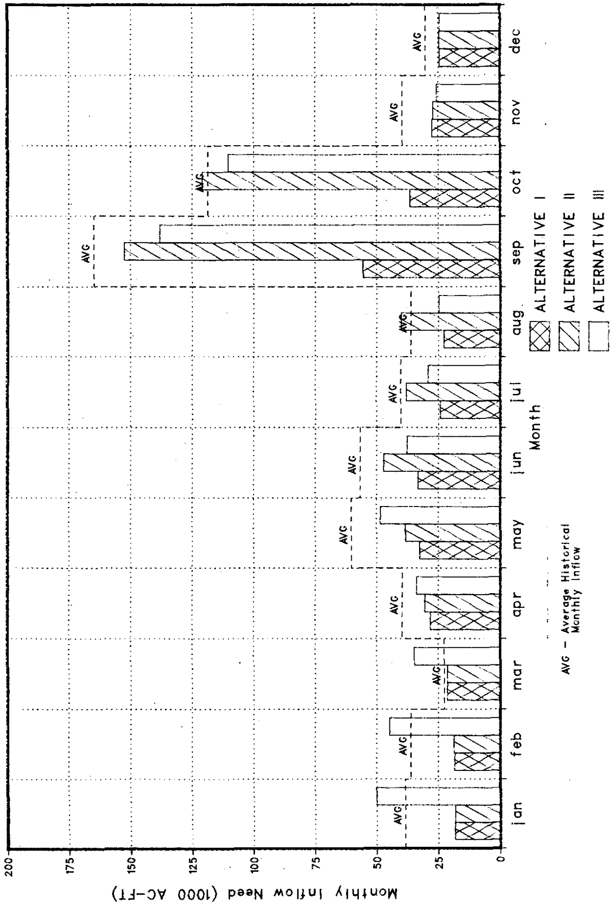
Figure 1-2. Estimated Monthly Freshwater Inflow Needs for the Laguna Madre Estuary Under Alternatives I, II, III
