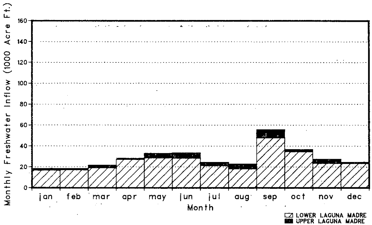
Figure 9-6. Estimated Freshwater Inflow Needs for the Laguna Madre Estuary Under Alternative I.
