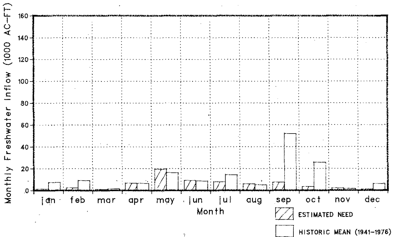
Figure 9-20. Comparison Between Mean Historical Freshwater Inflow and Inflow Needs for Upper Laguna Madre and Baffin Bay Under Alternative III
