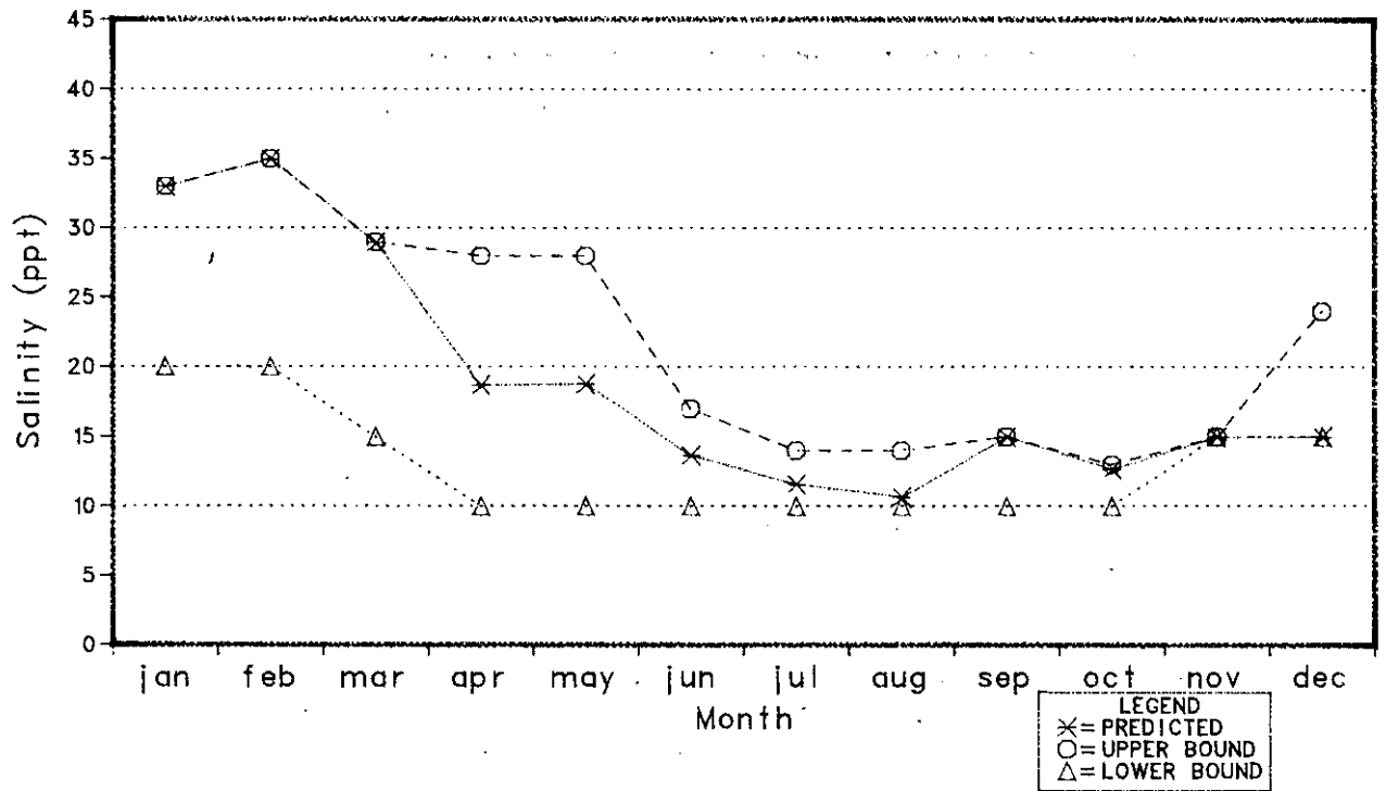
Figure 9-10. Average Monthly Salinity in Upper Baffin Bay Under Alternative II.
