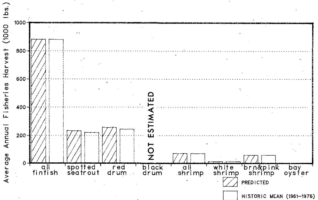
Figure 9-15. Comparison Between Upper Laguna Madre Historical Fisheries Harvests and Predicted Harvests Under Alternative II
