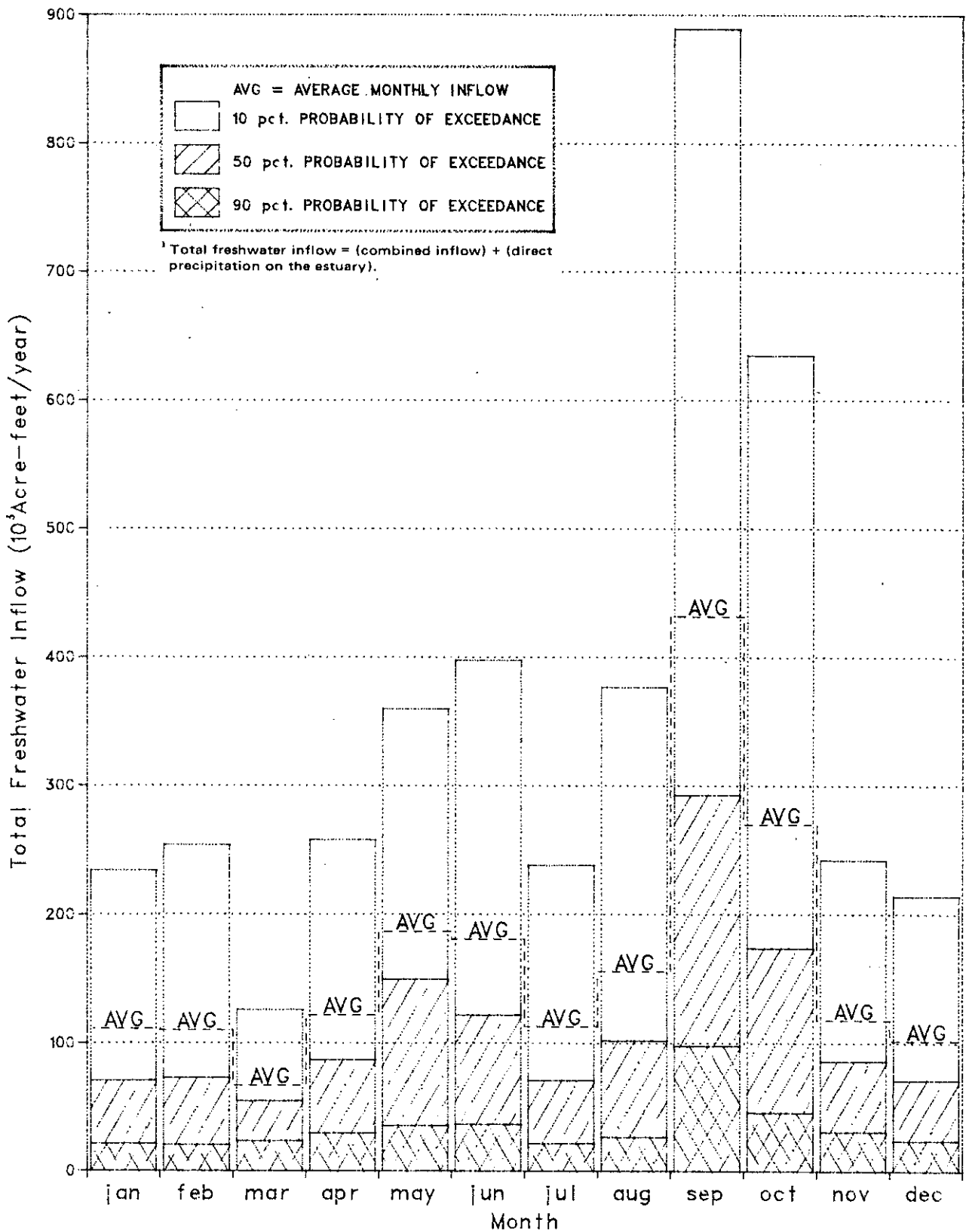
Figure 4-4. Monthly Distribution of Total Freshwater Inflow, 1 Laguna Madre Estuary, 1941-1976
